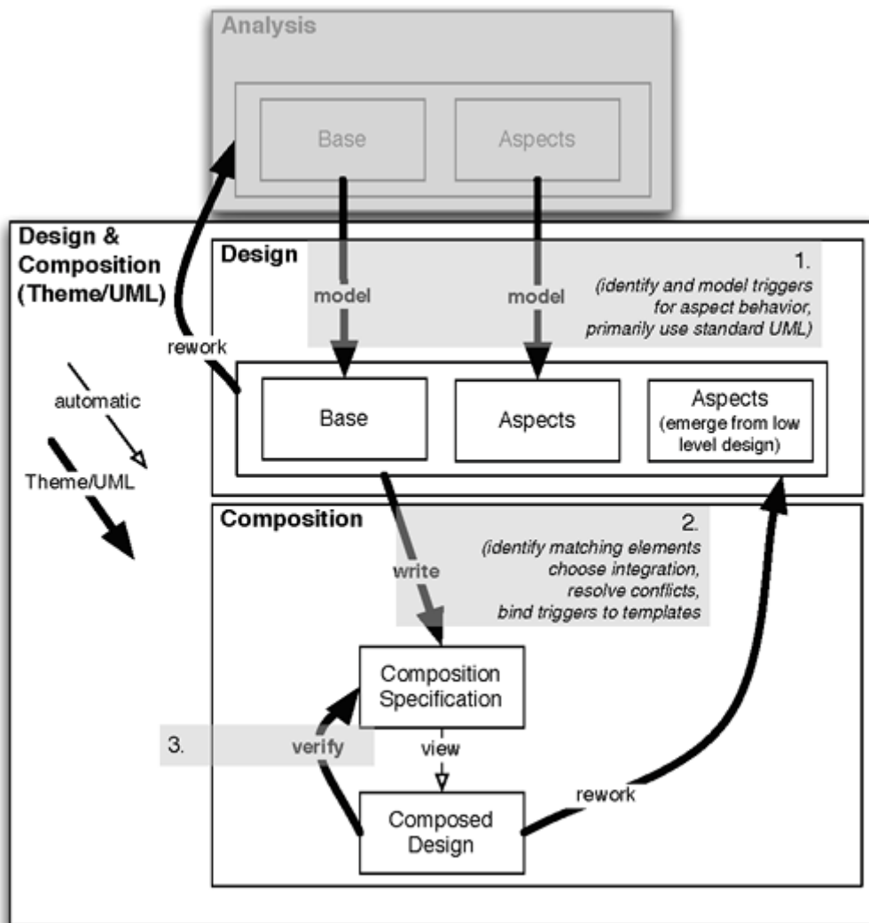
Figure 3-6 Overview of the Theme/UML process
