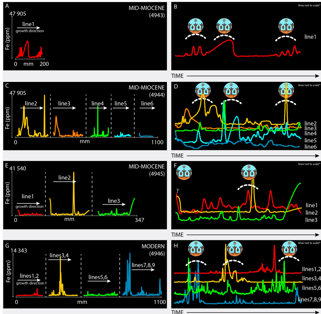
Figure 11. Elemental trend line obtained for Fe measurements (line numbers as in Fig. 4). (A), (C), (E) and (G) Record of Fe abundance along growth direction (in mm). (B), (D), (F) and (H) Same datasets stacked and slightly adjusted (vertically and horizontally) to compare different transects that represent similar portions of the molar. * Lines not to scale: mean horizontal scaling factor of 5.1; mean vertical scaling factor of 3.3 (see Table S1 in Appendix). Drawing represents dry season periods. Colors represent the different enamel transects analyzed. The same color scheme is used consistently across all figures to maintain clarity and allow for easy comparison of the different lines or transects.
