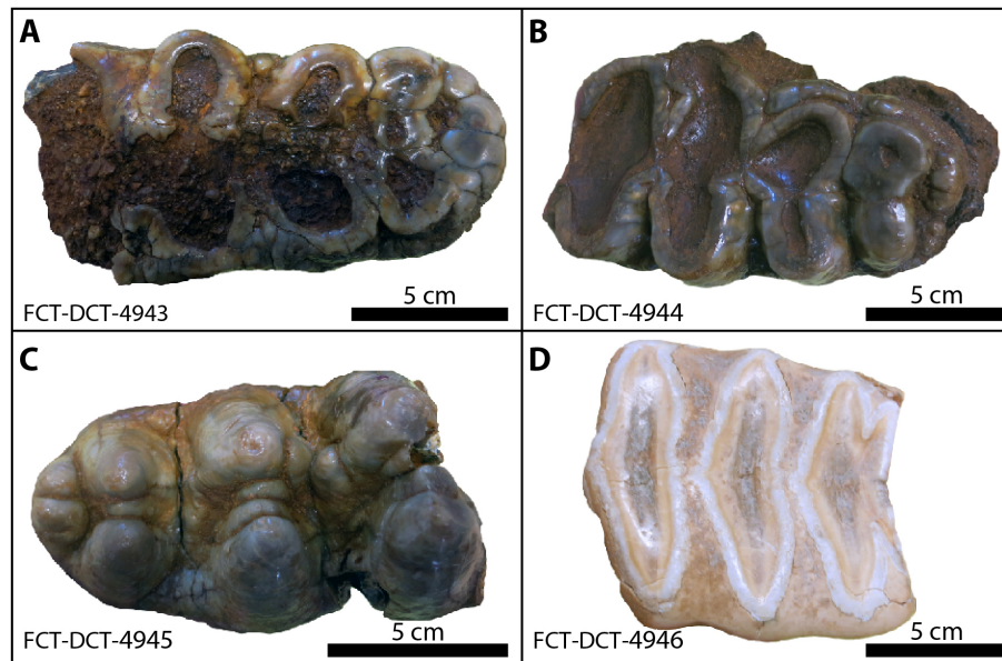
Figure 3. General aspect of uncut molar samples. (A) to (C) Gomphotherium angustidens molars, note less significant wear of the collected samples from (A) to (C). (D) Modern L. Africana molar, showing typical diamond-shaped ridges.
