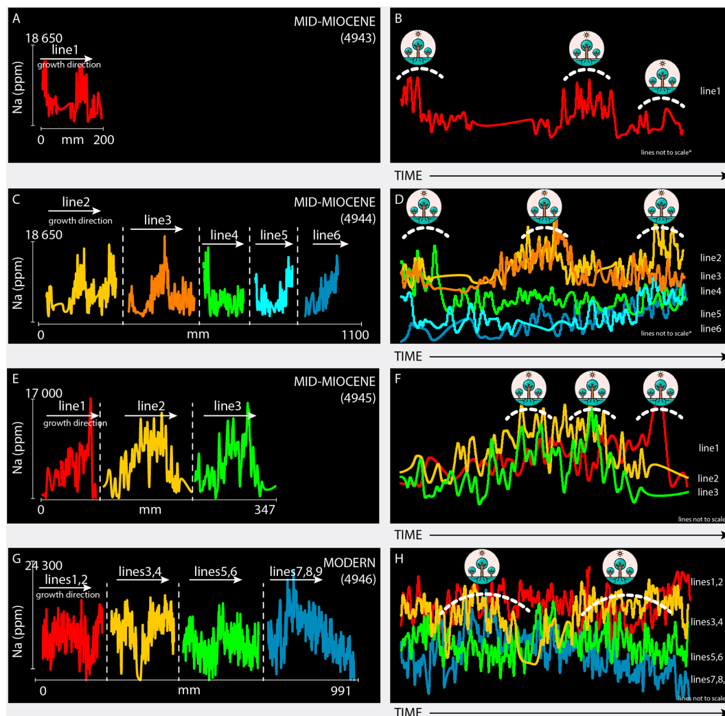
Figure 12. Elemental trend line obtained for Na measurements (line numbers as in Fig. 3). (A), (C) and (E) Record of Na abundance along growth direction (in mm). (B), (D) and (F) Same datasets stacked and slightly adjusted (vertically and horizontally) to compare different transects that represent similar portions of the molar. * Lines not to scale: mean horizontal scaling factor of 5.1; mean vertical scaling factor of 1 (see Table S1 in Appendix). Drawing symbol represents wet season periods. Colors represent the different enamel transects analyzed. The same color scheme is used consistently across all figures to maintain clarity and allow for easy comparison of the different lines or transects.
