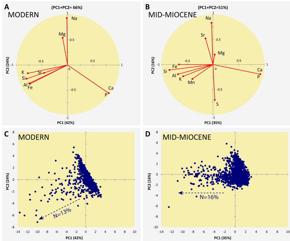
Figure 9. Principal component analysis computed for the modern and Mid-Miocene samples. (A) and (B) Principal component loadings explaining 51 % to 66 % of the total variability of each set of samples. Note similar distribution of elements along the PC axis. Modern Mn and S were not used due to low number of measurements available ( N < 30 %). (C) and (D) Principal component scores indicating sample distribution along the PCA space. Note main clusters of samples in both cases, with only few samples (13 % to 16 % of the total number of samples) departing from the observed main trend.
