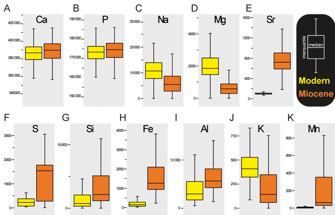
Figure 8. Boxplot representation (median and interquartile distance) of absolute elemental concentrations (in ppm). (A) and (B) note similar distribution of Ca and P; (C) and (D) lowered values for ancient samples regarding Na and Mg; (E) to (K) overall higher median values for the remaining proxies (except K). See Table 2 for full elemental range, mean and standard deviation.
