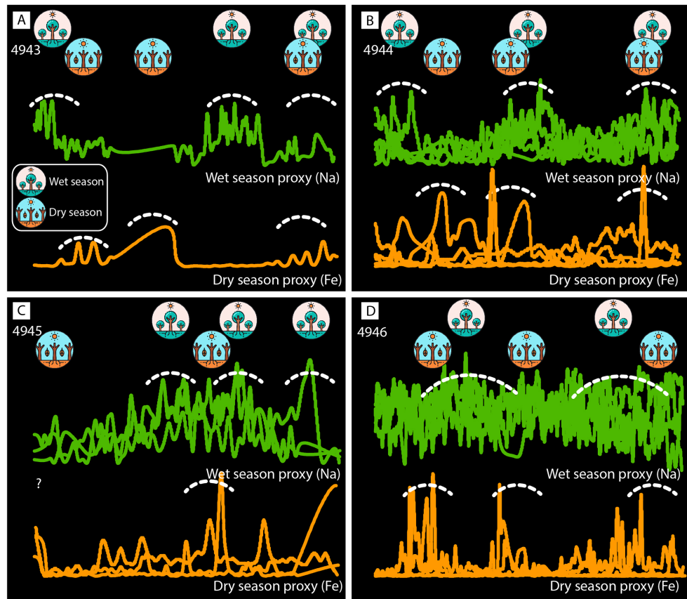
Figure 13. Compilation of elemental trend lines for Fe and Na as shown in Figs. 11 and 12. (A) to (C) Mid-Miocene transects in growth direction showing alternating peaks of higher abundance of the chosen elements. (D) Modern transects in growth direction showing alternating peaks of higher abundance of the chosen elements.
