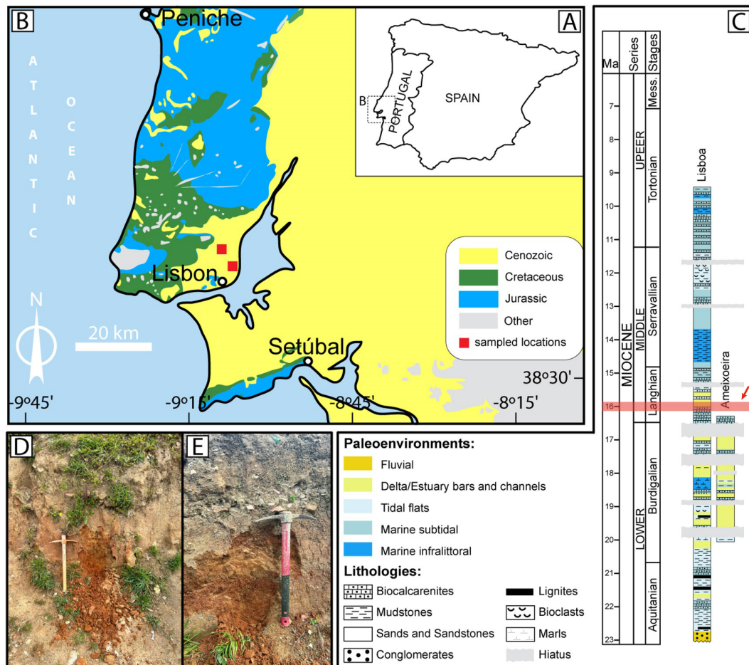
Figure 2. Geographical setting of the studied areas. (A) Location of the Portuguese mainland in the Iberia Peninsula. (B) Regional distribution of main geological outcrops at the Lisbon area (adapted from LNEG-LGM, 2010). Squares indicate the location of studied sections. (C) General biostratigraphic scheme for the Miocene and stratigraphic context of studied deposits at the Lisbon area (adapted from Pais et al., 2012). (D) and (E) Field aspect at the localities where the samples were extracted. The molars analysed in this study originate from the Quinta da Farinheira in the Lower Tagus Basin (Areias do Vale de Chelas, Lisbon). The Chelas unit has been designated SDL1 by Antunes and Ginsburg (2003) and Vb by Berkely-Cotter (1956), with an estimated age of ( \sim 15.9 – 16.1 Ma) and is highlighted by a red arrow. It belongs to the Langhian stage and the MN5 biozone (13.7–16.0 Ma).
