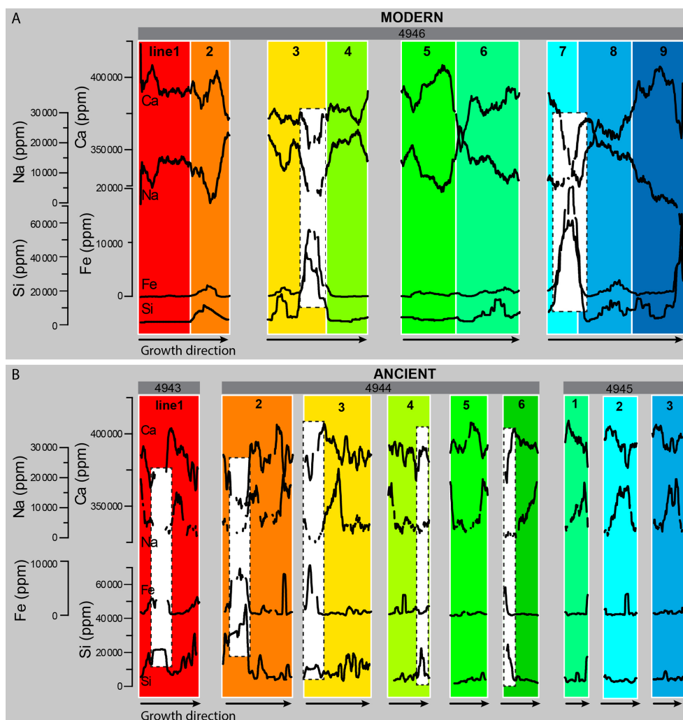
Figure 10. Elemental trend of selected proxies (Ca, Na, Fe and Si) for all measured transects (see Figs. 4 and 5 for exact measurement sites). (A) Trend lines for modern transects. (B) Trend lines for Mid-Miocene transects. Note overall similar records of Ca vs. Na and Fe vs. Si, as well as lack of clear enrichment or depletion trends along each transect. Note opposite variation pattern for Ca and Na, except when Fe and Si become significantly higher (white dashed boxes). Trend lines smoothed (10 points adjacent averaging); numerals according to Fig. 4. Colors represent the different enamel transects analyzed. The same color scheme is used consistently across all figures to maintain clarity and allow for easy comparison of the different lines or transects.
