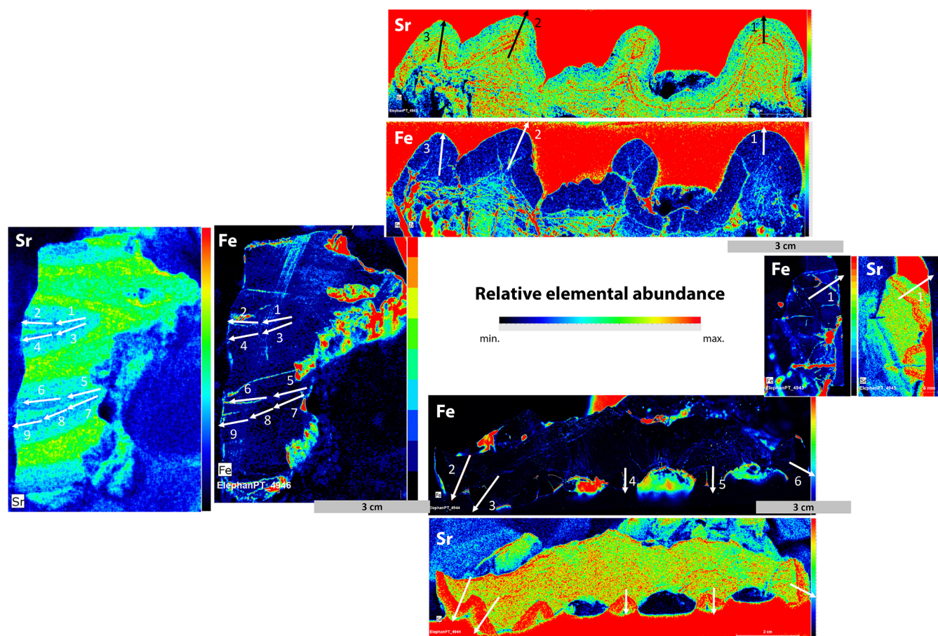
Figure 5. Relative elemental abundance for all specimen, here shown for iron and strontium (distribution of other elements can be found at https://doi.org/10.5281/zenodo.14882824 , Coimbra et al., 2025). Note the lack of areas denoting higher iron abundance along selected transects and the clear Sr concentration pattern highlighting well-preserved tooth morphology.
