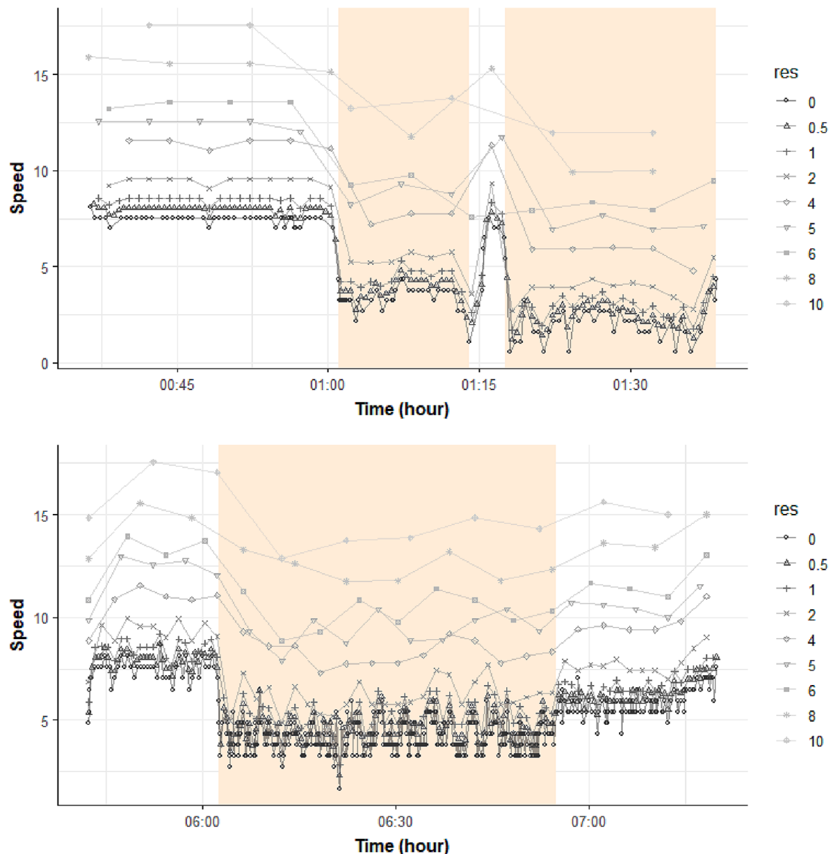
Fig. 2. Speed by time plot of a bivalve dredge (upper panel) and an octopus traps (lower panel) section of a boat trip example (only a section shown) to illustrate the effect of changes due to decreasing temporal resolution (increase time interval between points). Note that a constant was added to the speed by resolution level on the y axes to avoid overlap and improve visualization).
