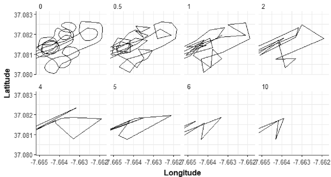
Fig. 3. Detail of a bivalve dredge boat trip, showing the typical loops registered for this gear. See the changes in the data with decreasing temporal resolution (increase time interval between points).
