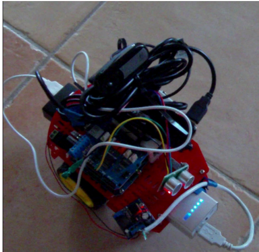
Fig. 1 A rudimentary prototype of the robotic assistant.
