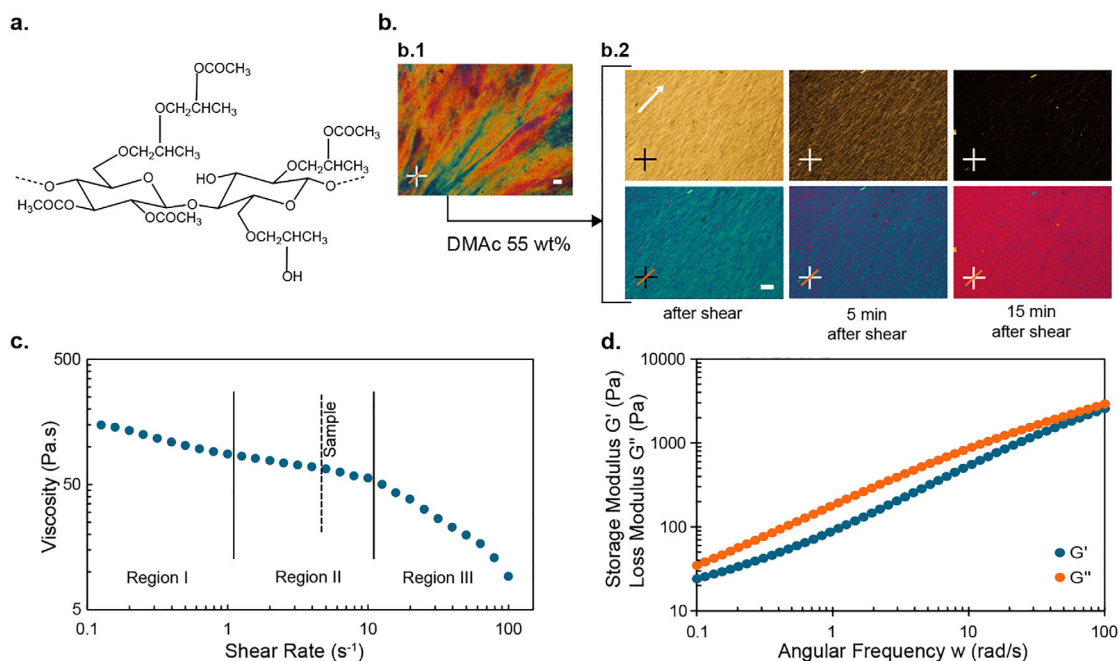
Figure 1. Precursor cellulose-based liquid crystalline materials. a) Idealized structure of acetoxypropylcellulose (APC) with a degree of molar etherification of 2.0, a degree of etherification of 1.5, and a degree of esterification of 2.0. b. Polarized optical microscopy (POM) photos taken in transmission. b.1) Texture of APC, between cross polars and a lambda plate (530 nm), 30 min after shearing. b.2) Textures observed between crossed polars (first row) and between crossed polars with a lambda plate (530 nm) (second row), after shearing a solution of 55 wt.% of APC in dimethylacetamide (DMAc), evolution after shear from 5 to 15 min. c) Viscosity versus shear rate curve for APC/DMAc (55 wt.%) (the shear rate used to make the films is indicated in the graph by "Sample"). d) Loss modulus ( G' ) and storage modulus ( G'' ) versus angular frequency ( \omega ) for APC/DMAc (55 wt.%). Scale bars: 100 \mu\text{m} (b.1, b.2.).
