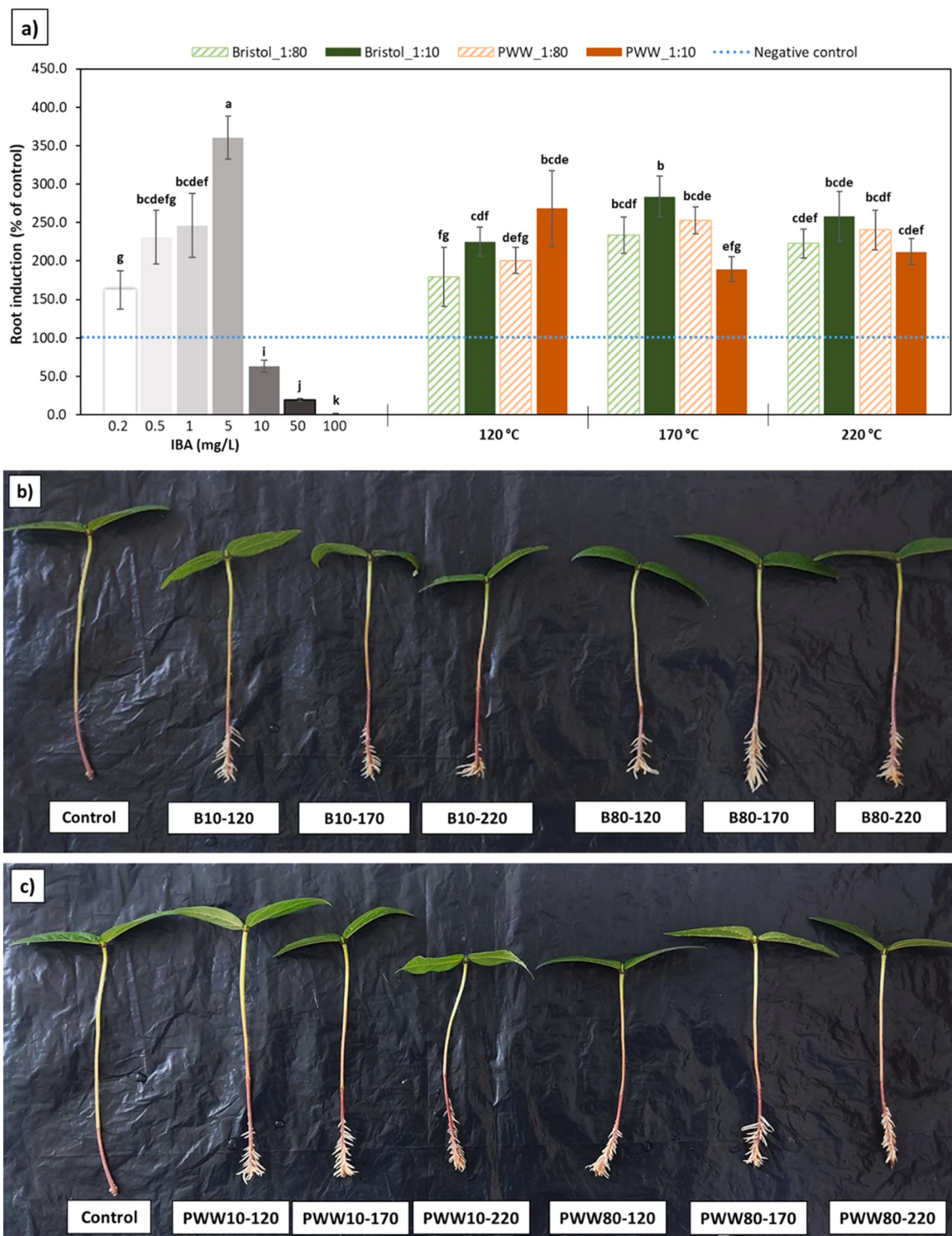
Fig. 4. Root development of mung bean treated with extracts (at 0.5 g/L) of Tetradismus obliquus , grown in Bristol medium or piggery wastewater (PWW), after subcritical water extraction at different temperatures (120, 170, and 220 °C) and biomass loading (1:10 and 1:80 (g dry biomass/mL water)): a) Root induction (%). Distilled water was used as the negative control (dotted blue line) and a standard curve of Indole-3-acetic Acid (IBA) was used as positive control (0.2 – 100 mg/L). The columns and error-bars represent mean \pm standard deviation ( n=3 ). Different letters indicate significant difference ( p < 0.05 ) among treatments according to Games-Howell's two-sided post-hoc test; b) Photograph of mung bean plants treated with extracts from biomass grown in Bristol (B) medium; c) Photograph of mung bean plants treated with extracts from biomass grown in piggery wastewater (PWW).
