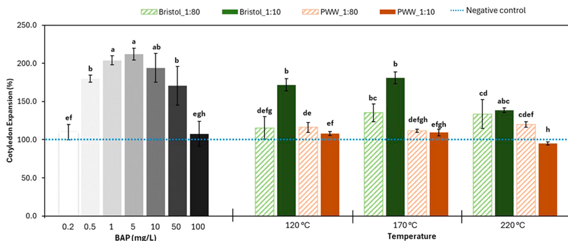
Fig. 6. Expansion of excised cucumber cotyledons treated with extracts of Tetradismus obliquus , grown in Bristol medium or piggy wastewater (PWW), after subcritical water extraction at different temperatures (120, 170, and 220 °C) and biomass loading (1:10 and 1:80 (g dry biomass/mL water)), compared to distilled water (negative control – dotted blue line). A standard curve of 6-benzylaminopurine (BAP) was used as positive control (0.2 – 100 mg/L). The columns and error-bars represent mean \pm standard deviation ( n=3 ). Different letters indicate significant difference ( p < 0.05 ) among treatments according to Games Howell's two-sided post-hoc test.
