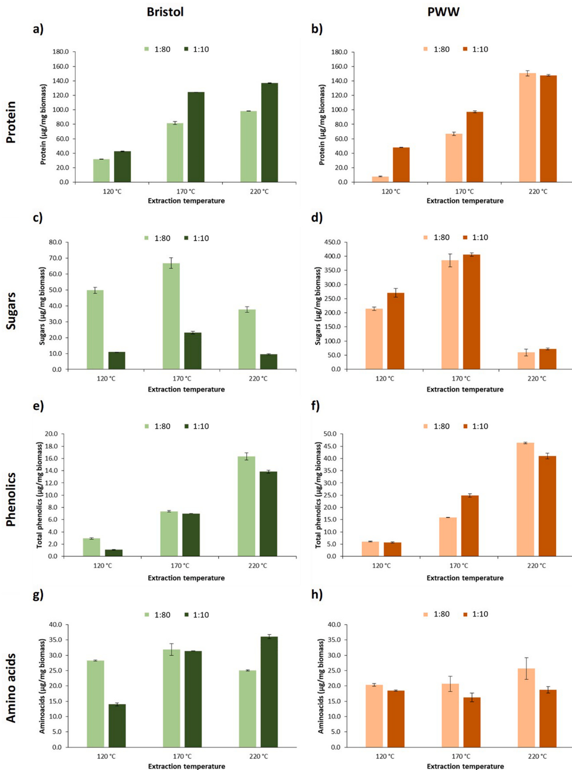
Fig. 2. Extraction yield of extracted compounds from Tetrademus obliquus , grown in synthetic Bristol medium or piggery wastewater (PWW), submitted to subcritical water extraction at different temperatures (120, 170, and 220 °C) and biomass loadings (1:10 and 1:80 (g dry biomass/mL water)): a) Protein; b) Sugars; c) Phenolics; and d) Amino acids. The columns and error-bars represent mean \pm mean deviation ( n=2 ).
