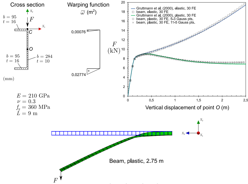
Figure 6: Channel cantilever beam.
