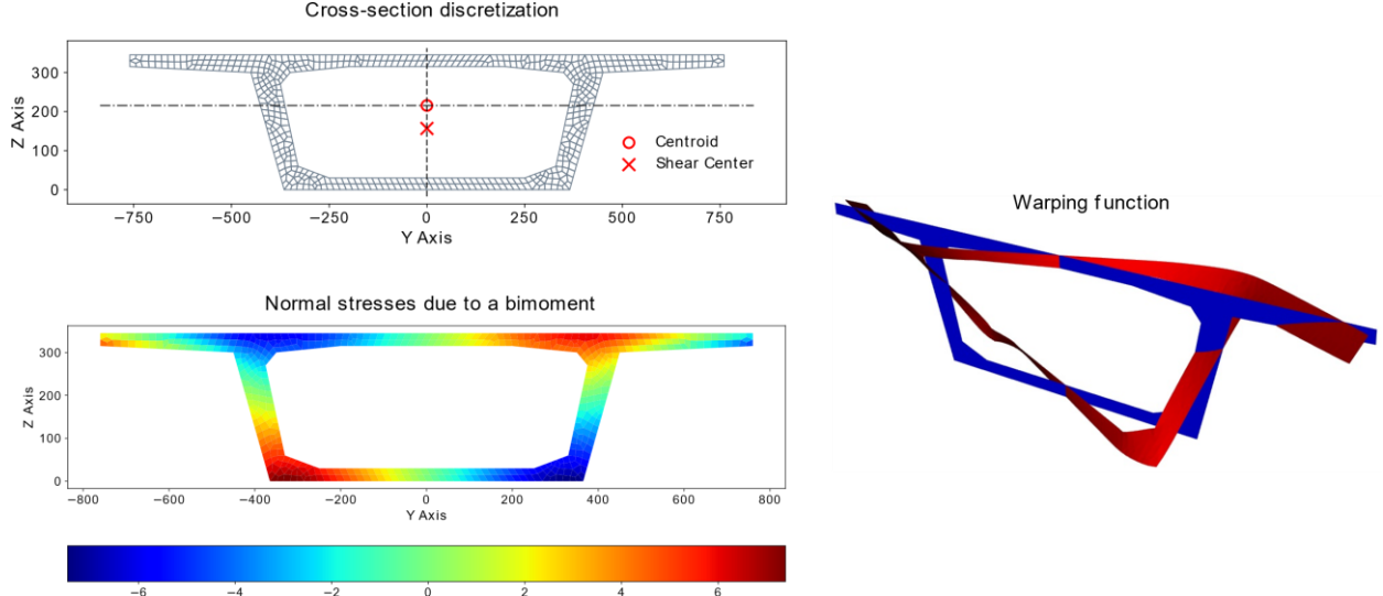
Figure 3: Torsion-warping function and normal stresses due to a bi-moment for a box girder bridge cross-section.
