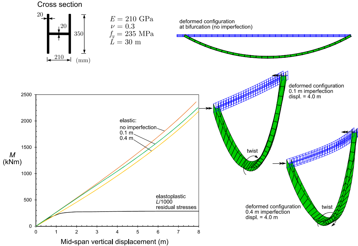
Figure 11: Buckling of a wide flange H-section beam.
