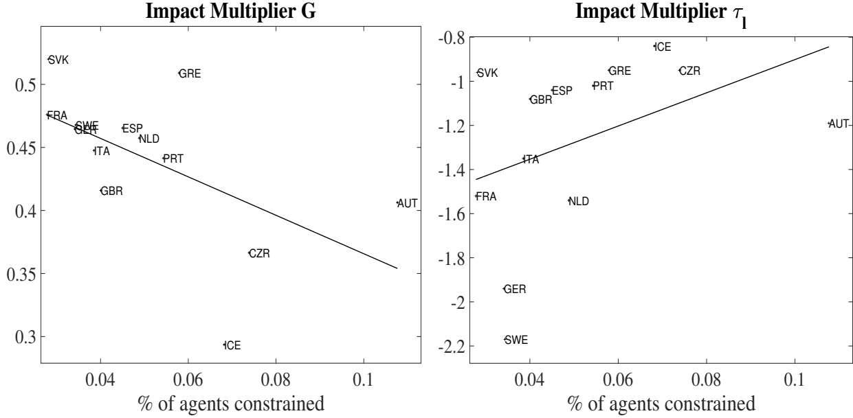
Figure 11: Impact multiplier and percentage of agents constrained. On the left panel we have the cross-country data for a consolidation done by decreasing G (correlation coefficient -0.68 , p -val 0.01 ), while on the right panel we have the cross-country data for a consolidation done by increasing the labor tax (correlation coefficient 0.55 , p -val 0.06 )
