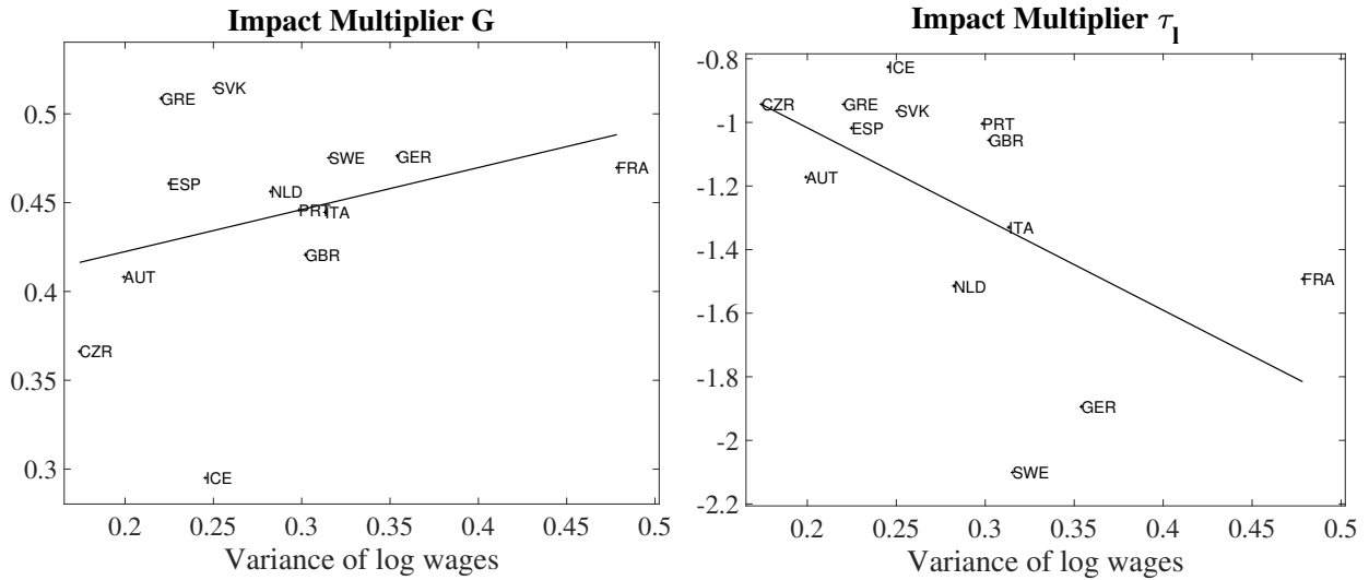
Figure 28: Impact multiplier for the experiment when \rho_u = 0.8 and \text{Var}(\ln(w)) . On the left panel we have the cross-country data for a consolidation done by decreasing G (correlation coefficient 0.35 , p\text{-val} 0.24 ), while on the right panel we have the cross-country data for a consolidation done by increasing the labor tax (correlation coefficient -0.71 , p\text{-val} 0.01 ).
