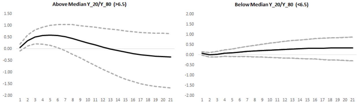
Figure 14: Cumulative output multiplier, as defined in (27), to a government consumption shock (90 percent error bands in gray)
