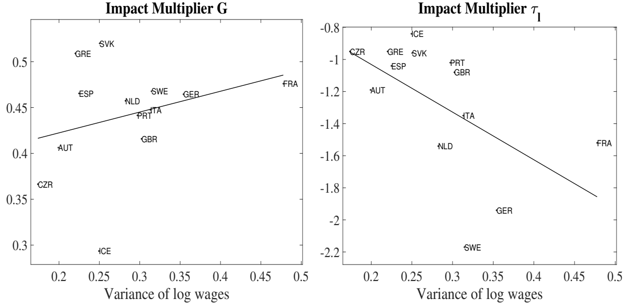
Figure 9: Impact multiplier and \text{Var}(\ln(w)) . The left panel displays the cross-country data for a consolidation implemented by decreasing G (correlation coefficient 0.35 , p-val 0.25 ), and the right panel displays the cross-country data for a consolidation implemented by increasing the labor tax (correlation coefficient -0.60 , p-val 0.03 ).
