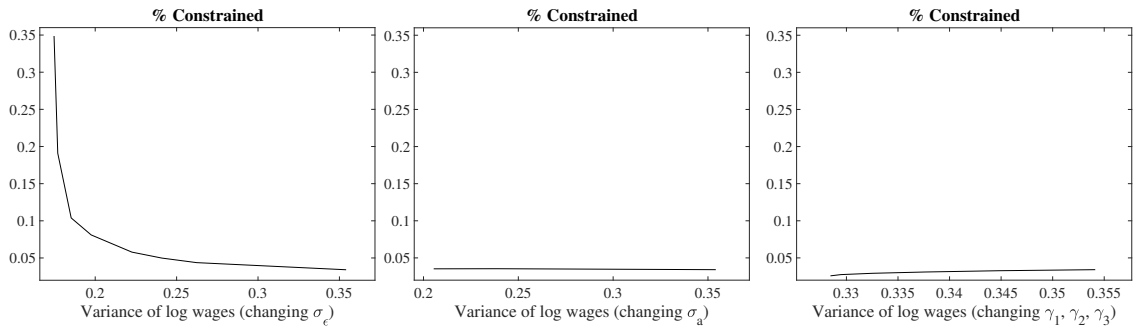
Figure 7: Share of credit-constrained agents in the German benchmark economy when changing the variance of risk (left panel), the variance of ability (middle panel), and the age profile of wages (right panel).
