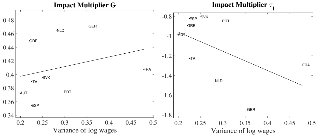
Figure 23: Impact multiplier and \text{Var}(\ln(w)) in a model calibrated to match the liquid wealth distribution. On the left panel we have the cross-country data for a consolidation done by decreasing G (correlation coefficient 0.4500; p-value 0.2298), while on the right panel we have the cross-country data for a consolidation done by increasing the labor tax (correlation coefficient -0.3833; p-value 0.3125).
