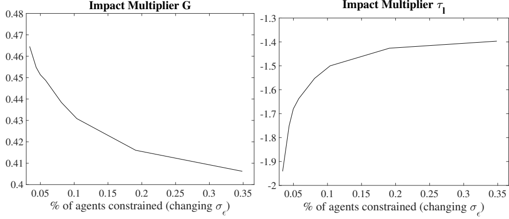
Figure 8: Impact multiplier for the G-consolidation (left panel) and for the \tau_1 -consolidation (right panel) plotted against the share of credit-constrained agents in the German benchmark economy, when decreasing the variance of risk.
