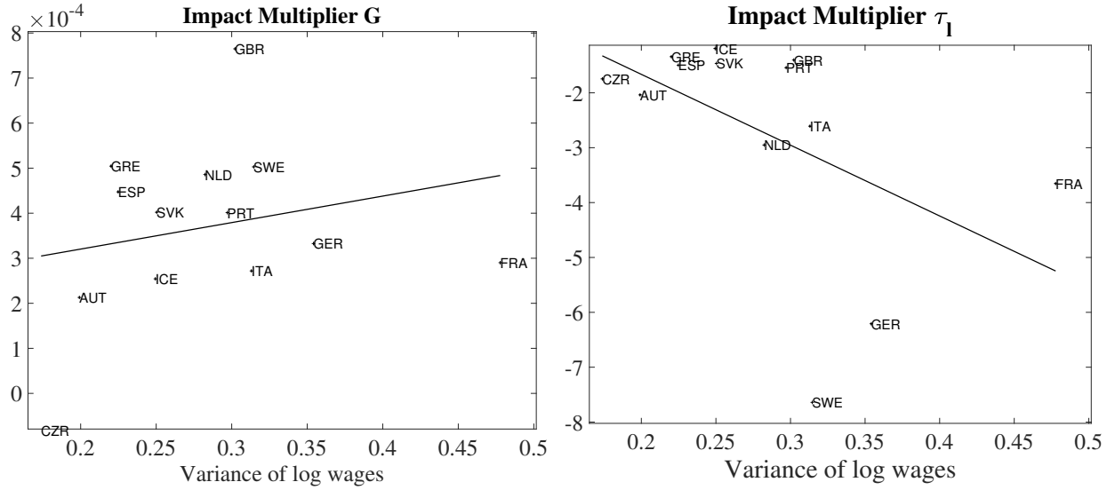
Figure 26: Impact multiplier and \text{Var}(\ln(w)) in a partial equilibrium model. On the left panel we have the fiscal multiplier across countries for the G consolidation, in a setting where wages and interest rate are constant. On the right panel, we have the fiscal multipliers across countries for the labor tax experiment in the same constant wages and interest rate environment.
