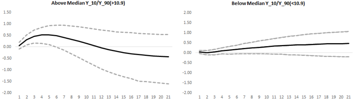
Figure 15: Cumulative output multiplier, as defined in (27), to a government consumption shock (90 percent error bands in gray)
