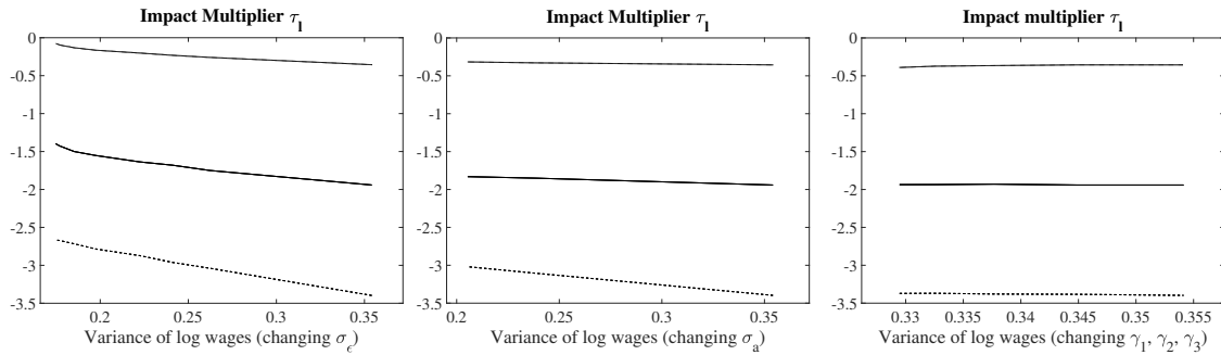
Figure 19: Impact multiplier for the consolidation through government spending in the German benchmark economy when changing the variance of risk (left panel), the variance of ability (middle panel), and the age profile of wages (right panel). The dashed line illustrates the results when \sigma = 0.5 , the solid line for the benchmark value of \sigma = 1.2 and the dotted line for \sigma = 4 .
