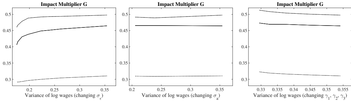
Figure 18: Impact multiplier for the consolidation through government spending in the German benchmark economy when changing the variance of risk (left panel), the variance of ability (middle panel), and the age profile of wages (right panel). The dashed line illustrates the results when \sigma = 0.5 , the solid line for the benchmark value of \sigma = 1.2 and the dotted line for \sigma = 4 .
