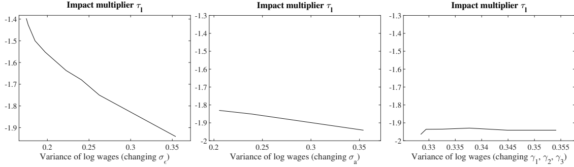
Figure 5: Impact multiplier for the labor tax consolidation in the benchmark model for Germany when changing the variance of risk (left panel), the variance of ability (middle panel), and the age profile of wages (right panel).
