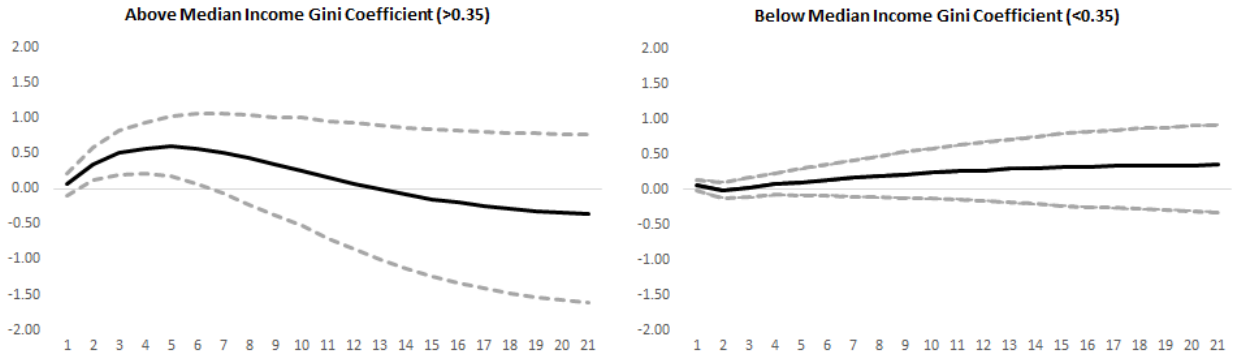
Figure 16: Cumulative output multiplier, as defined in (27), to a government consumption shock (90 percent error bands in gray)
