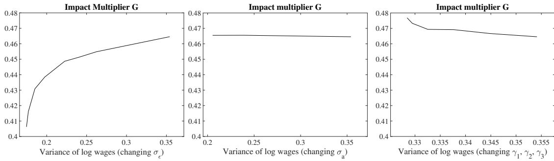
Figure 6: Impact multiplier for the consolidation through government spending in the German benchmark economy when changing the variance of risk (left panel), the variance of ability (middle panel), and the age profile of wages (right panel).
