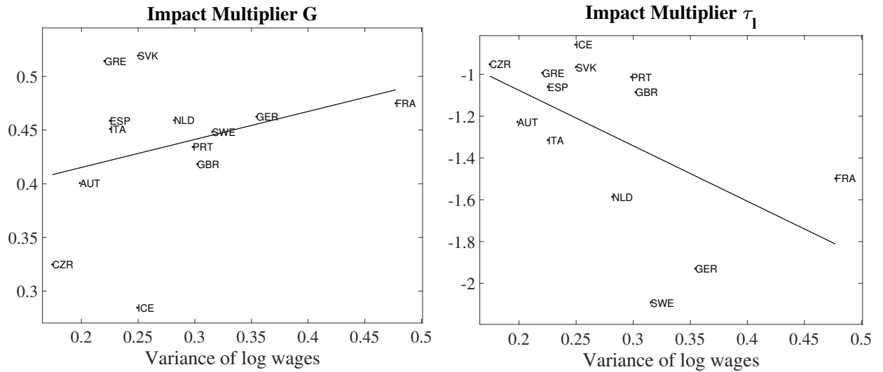
Figure 27: Impact multiplier for the experiment where risk and ability each explain 50 percent of the variance of log wages and \text{Var}(\ln(w)) . The left panel displays the cross-country data for the G consolidation multiplier (correlation coefficient 0.31 , p-val 0.30 ), whereas the right panel displays cross-country data for the labor tax consolidation (correlation coefficient -0.60 , p-val 0.03 ).
