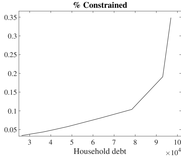
Figure 12: The fraction of liquidity-constrained agents (y-axis) and household debt level (x-axis), when changing the level of idiosyncratic risk in the German benchmark economy.
