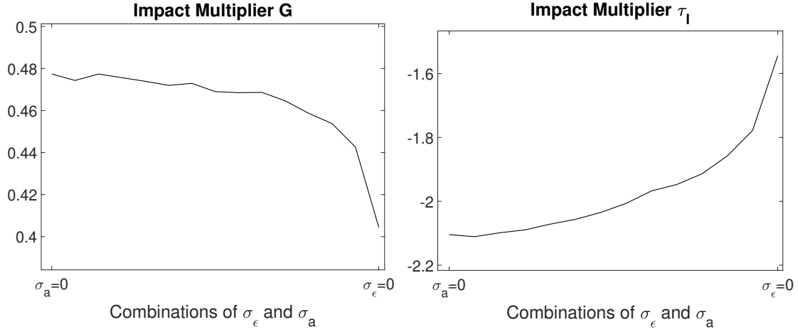
Figure 17: Impact multiplier for the G-consolidation (left panel) and for the \tau_1 -consolidation (right panel) for different combinations of variance of ability and risk on the x-axis, keeping variance of log wages constant. The variance of ability is increasing from left to right. When the variance of ability is zero, all inequality is due to risk, which is calibrated to keep the variance of log wages at the benchmark value. When the variance of risk is zero, all inequality is due to the variance of ability, which is calibrated to match the variance of log wages.
