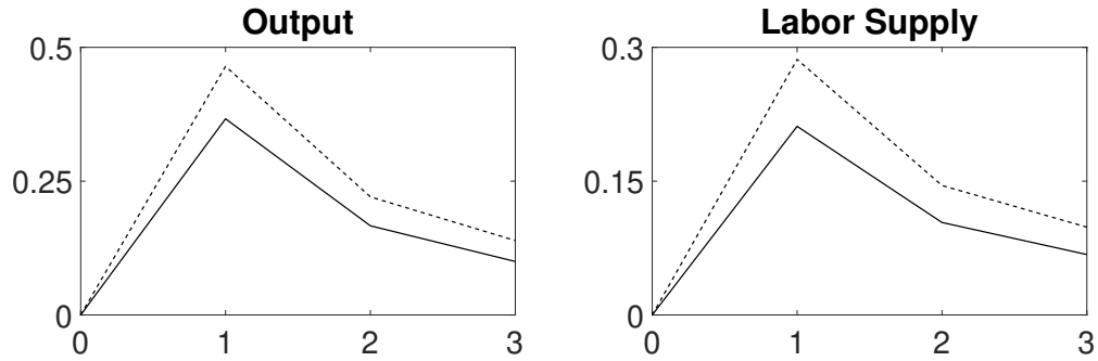
Figure 4: Government spending consolidation: Output cumulative multiplier (left panel) and Labor Supply cumulative multiplier (right panel) in the first three periods in Germany (dashed line) and Czech Republic (solid line)
