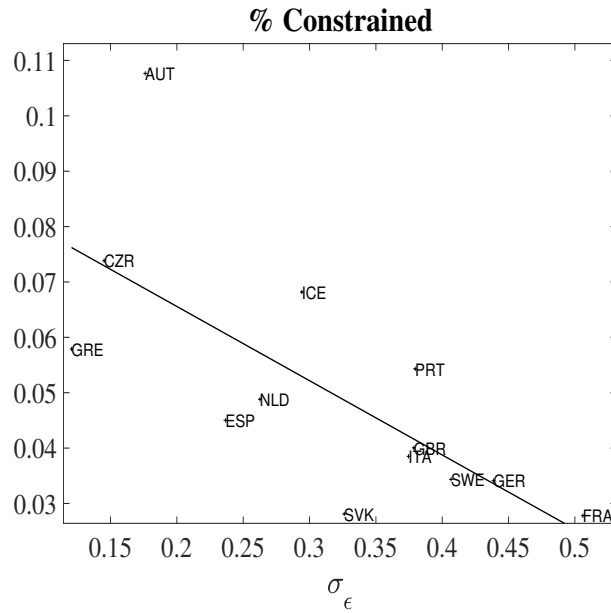
Figure 10: Percentage of agents constrained in the y-axis and variance of idiosyncratic risk on the x axis. Correlation coefficient of -0.73 and p-value of 0.00
