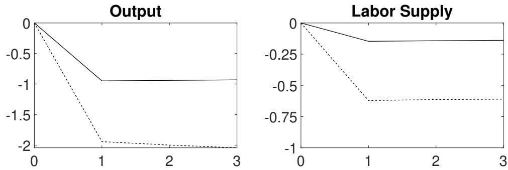
Figure 3: Labor tax consolidation: Output cumulative multiplier (left panel) and Labor Supply cumulative multiplier (right panel) in the first three periods in Germany (dashed line) and Czech Republic (solid line)
