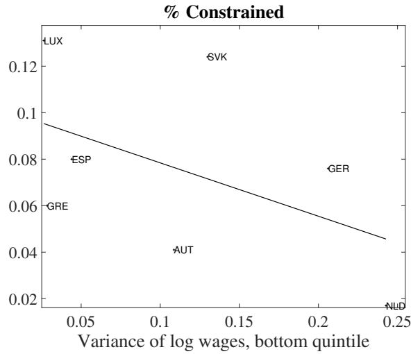
Figure 13: The relationship between wage volatility of the lowest 20 percent of earners and the share of households who felt credit constrained. Correlation coefficient of -0.48 and p-value of 0.27. Wage data comes from Luxembourg Income Study survey year 2010, which corresponds most closely to the survey responses of HFCS 1st wave. Constrained households are households who answered affirmatively to survey questions regarding either being rejected when seeking credit, not receiving full amount requested, or forgoing requesting credit due to expectation of being rejected.
