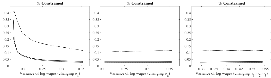
Figure 20: Percentage of constrained agents in the benchmark model for Germany when changing the variance of risk (left panel), the variance of ability (middle panel), and the age profile of wages (right panel). The dashed line illustrates the results when \sigma = 0.5 , the solid line for the benchmark value of \sigma = 1.2 and the dotted line for \sigma = 4 .
