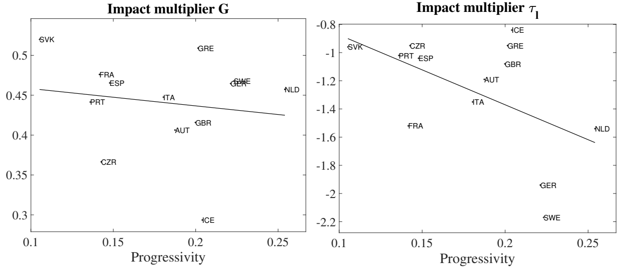
Figure 22: Impact multiplier and \theta_1 . The left panel displays the cross-country data for a consolidation implemented through decreasing G (correlation coefficient -0.1209, p-val 0.6961), while the right panel displays the cross-country data for a consolidation implemented through increasing the labor tax (correlation coefficient -0.4209, p-val 0.1521)
