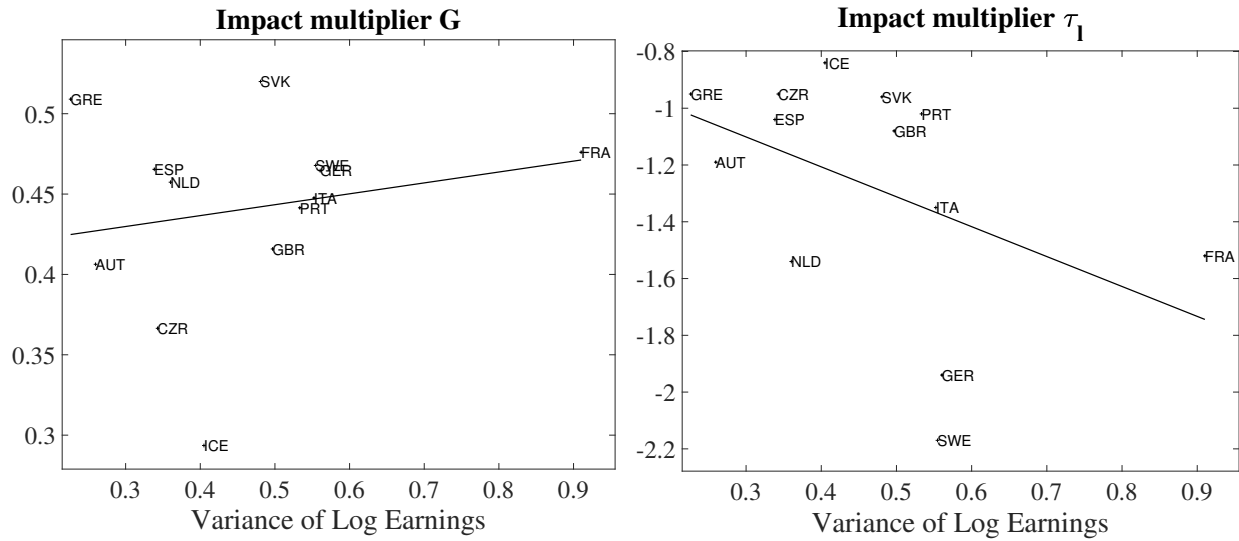
Figure 21: Impact multiplier and variance of disposable labor earnings. The left panel displays the cross-country data for a consolidation implemented through decreasing G (correlation coefficient 0.1868, p-val 0.5413), while the right panel displays the cross-country data for a consolidation implemented through increasing the labor tax (correlation coefficient -0.4924, p-val 0.0873).
