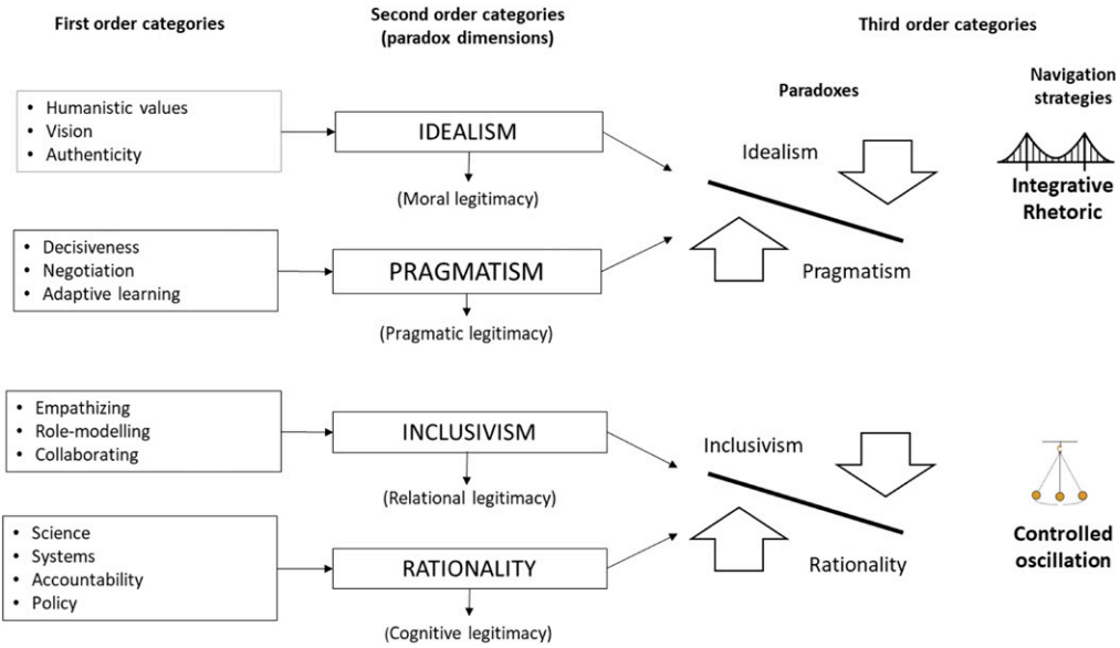
Figure 1. Data structure.
