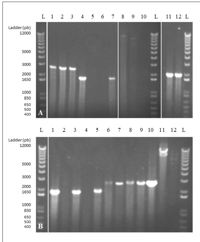
Figure 3.6 – Panel A: Screening of NCTC 8325-4 \Delta 773 mutants derivivate from the Down integrate NCTC 8325-4::pMAD del 773 (colony 1D obtained in the Integration) by agarose gel electrophoresis analysis of DNA fragments amplified by PCR. PCR fragments amplified from DNA extracted from several colonies are shown in the different lanes. Lanes 1 to 3, 5 and 6 – PCR for NCTC 8325-4 \Delta 773 DNA resulting in bands (or with no amplification) corresponding to a non-deleted gene colony; Lanes 4 (colony 1D.20), 7 (colony 1D.23), 11 and 12 – PCR for NCTC 8325-4 \Delta 773 DNA resulting in bands corresponding to a deleted gene colony; Lane 8 – PCR resulting from NCTC 8325-4::pMAD del 773 (1D) DNA (negative control); Lane 9 – PCR resulting from NCTC 8325-4 DNA (negative control); Lane 10 – PCR carried out with no template DNA (negative control); Lanes L – DNA ladders with band sizes (in base pairs).
