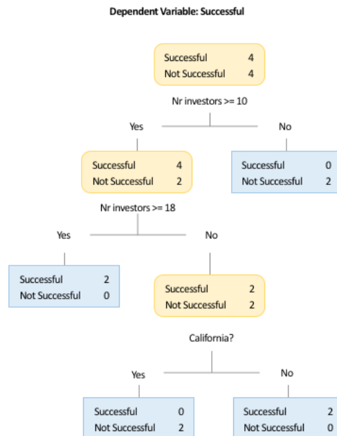
Figure 13 – Decision Tree sample tree (example)
