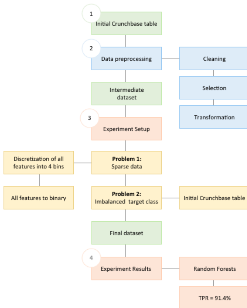
Figure 1 - Methodology Overview
