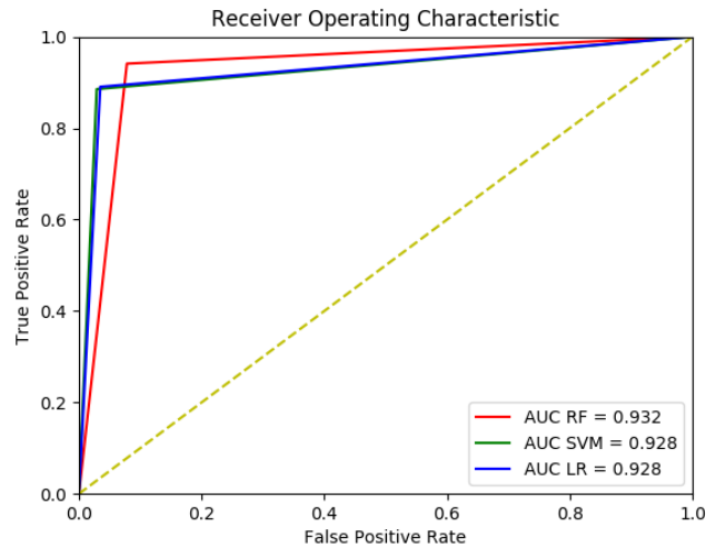
Figure 11 - ROC Curve
