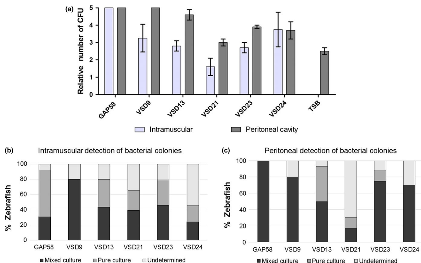
FIGURE 4 (a) Relative number of CFUs in intramuscular and peritoneal region of zebrafish inoculated with SDSD isolates (VSD13, VSD9, VSD21, VSD23, and VSD24) or S. pyogenes GAP58. For control purposes, zebrafish were inoculated with 10 \mu l of TSB-0.5YE. The relative CFUs in both anatomic regions were scored as follows: 0, no colonies; 1: 1 to 50 colonies; 2: 51 to 200 colonies; 3: 201 to 500 colonies; 4: > 500 colonies. (b) Percentage of zebrafish that died before 15 days of experiment with mixed and pure colonies in the intramuscular region. (c) Percentage of zebrafish that died before 15 days of experiment with mixed and pure colonies in the peritoneal region. Pure culture: containing colonies of the respective SDSD isolate. Mixed culture: contains colonies from more than one type of bacteria
