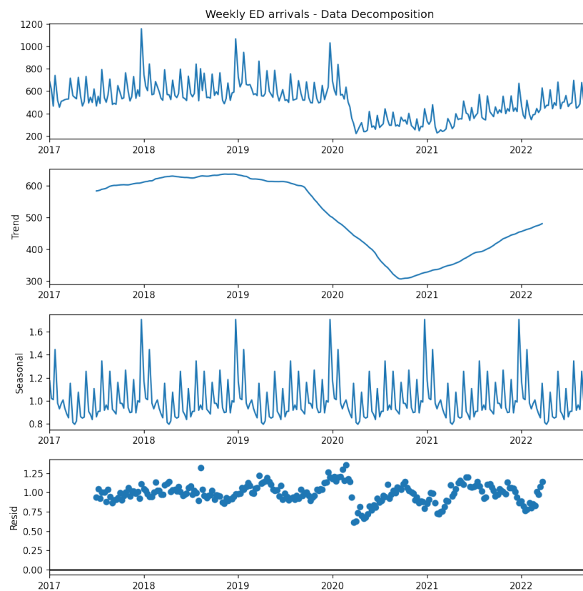
Figure A.48: Unit 3 - Seasonal Decompose
