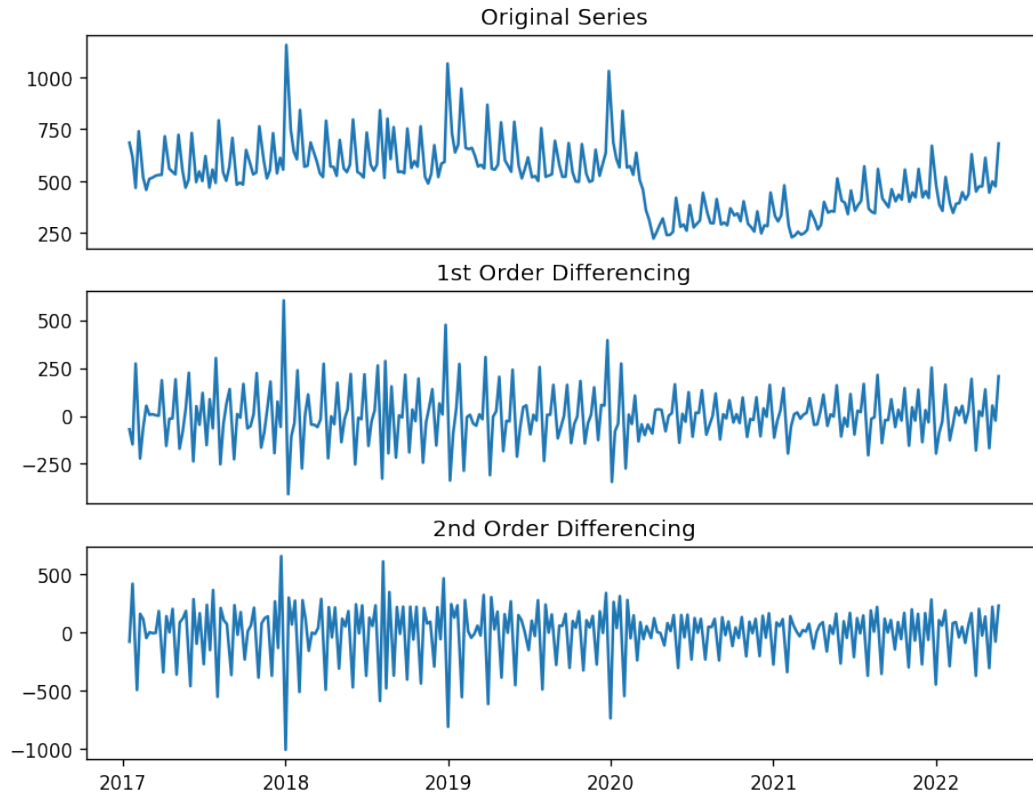
Figure A.49: Unit 3 - First and Second Order of Differentiation
