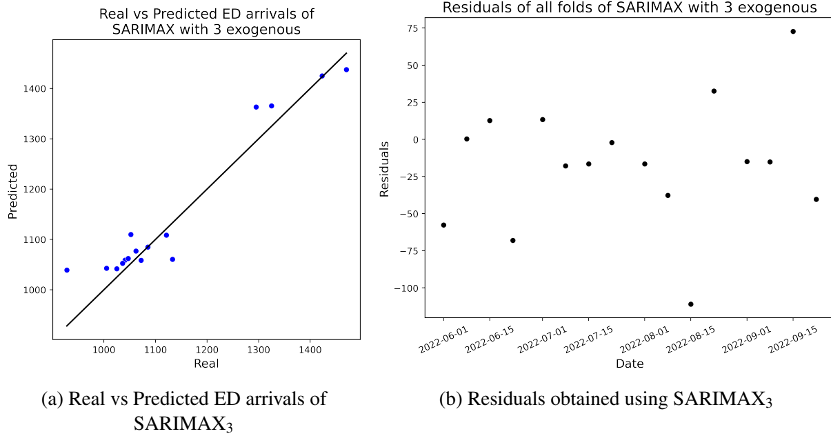
Figure 6.2: SARIMAX 3 residuals
