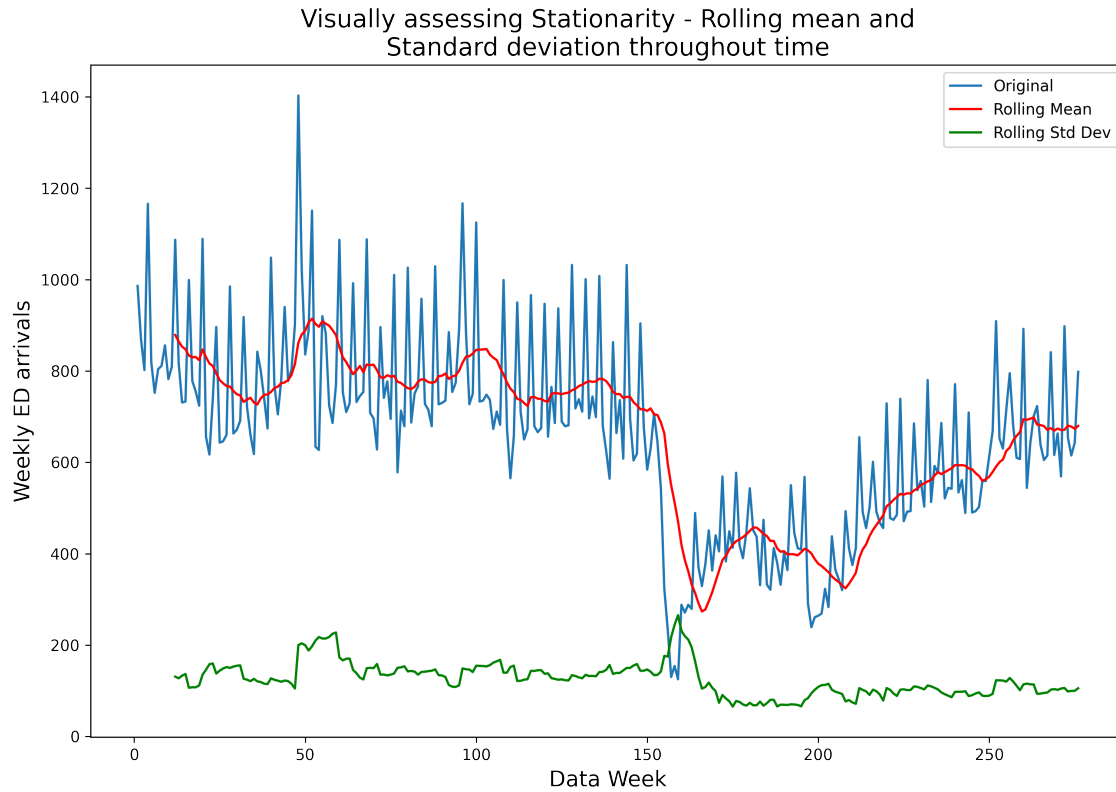
Figure A.30: Stationarity of the NU ED arrivals dataset
