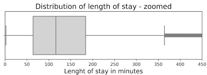
Figure A.53: Unit 18 - Distribution of Length of Stay
