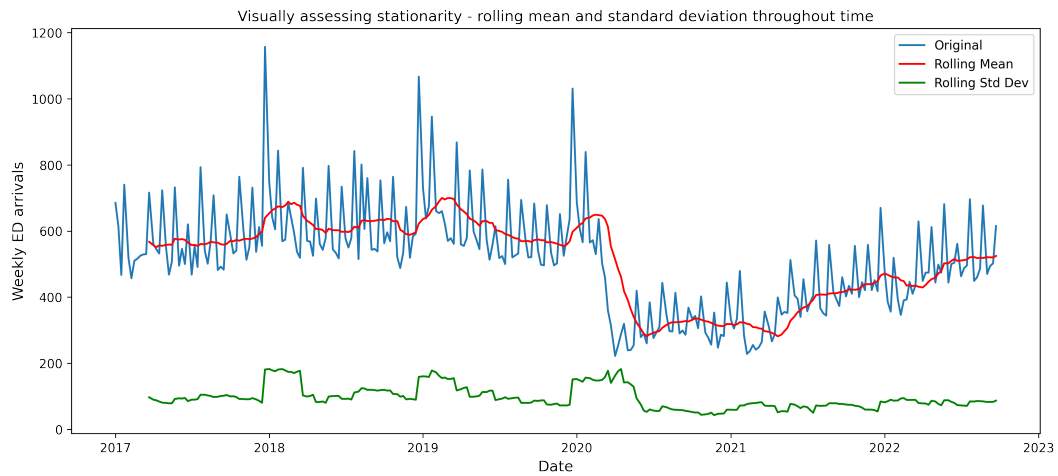
Figure A.47: Unit 3 - Rolling Mean and Standard Deviation throughout the years
