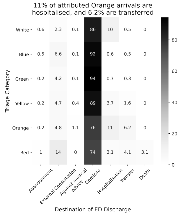
Figure A.42: Unit 3 - Percentage of ED Discharge Destination per Triage Category
