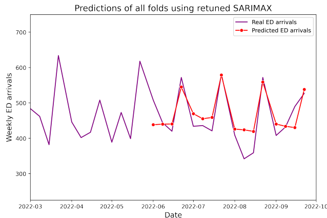
Figure 8.5: SARIMAX UP-7 Weekly Predictions of All folds
