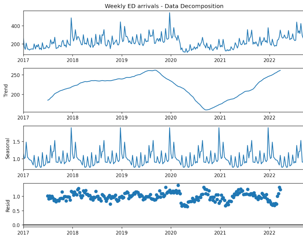
Figure A.56: Unit 18 - Seasonal Decompose
