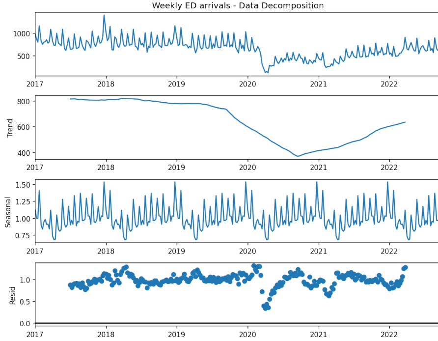
Figure A.31: Decomposition of the NU ED arrivals dataset
