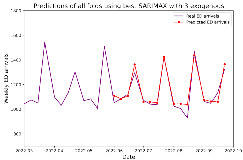
Figure 6.1: \text{SARIMAX}_3 predictions of all folds
