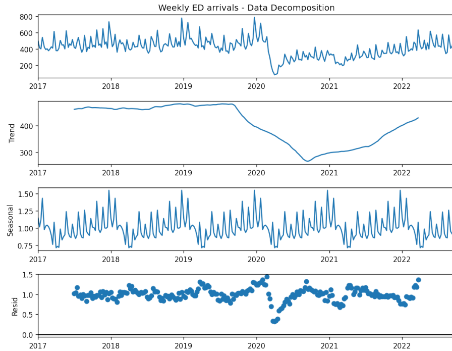
Figure A.38: Urgent Season Decompose
