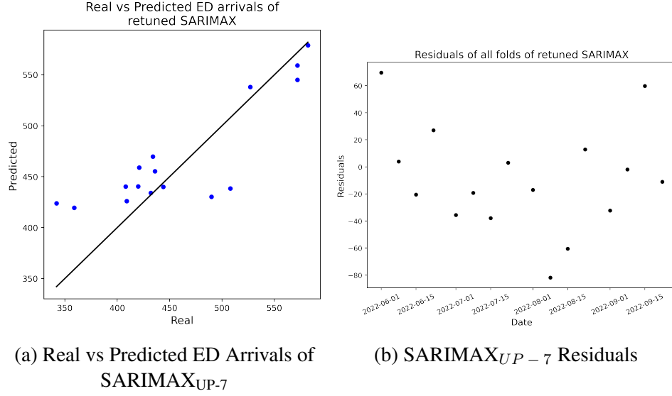
Figure 8.6: SARIMAX UP-7 Best Model
