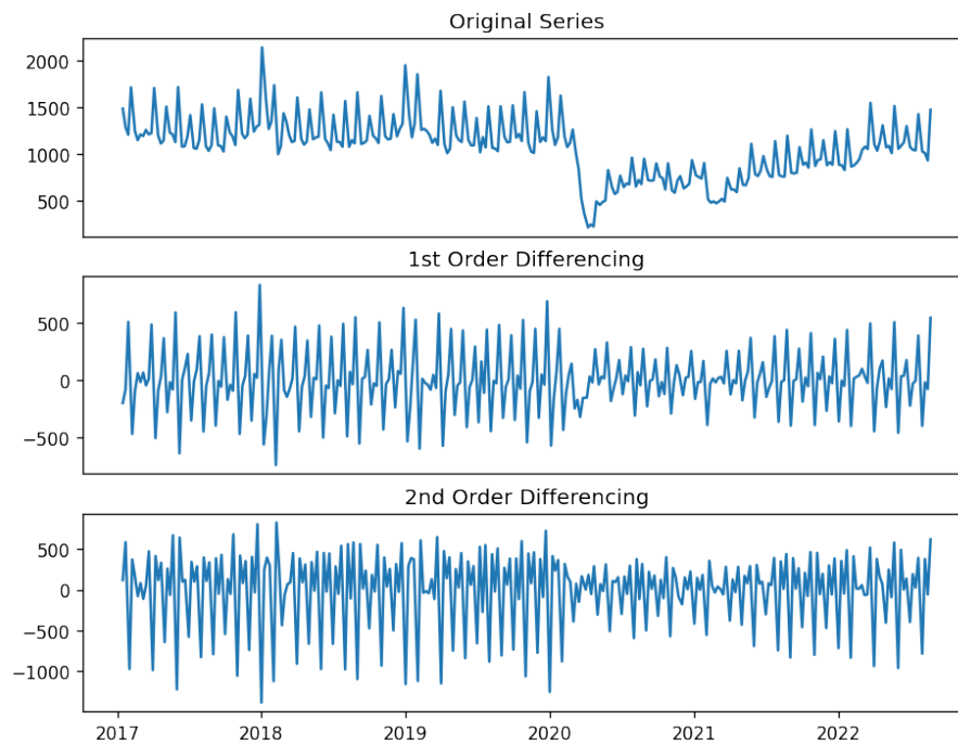
Figure A.21: Differentiation order - All Data
