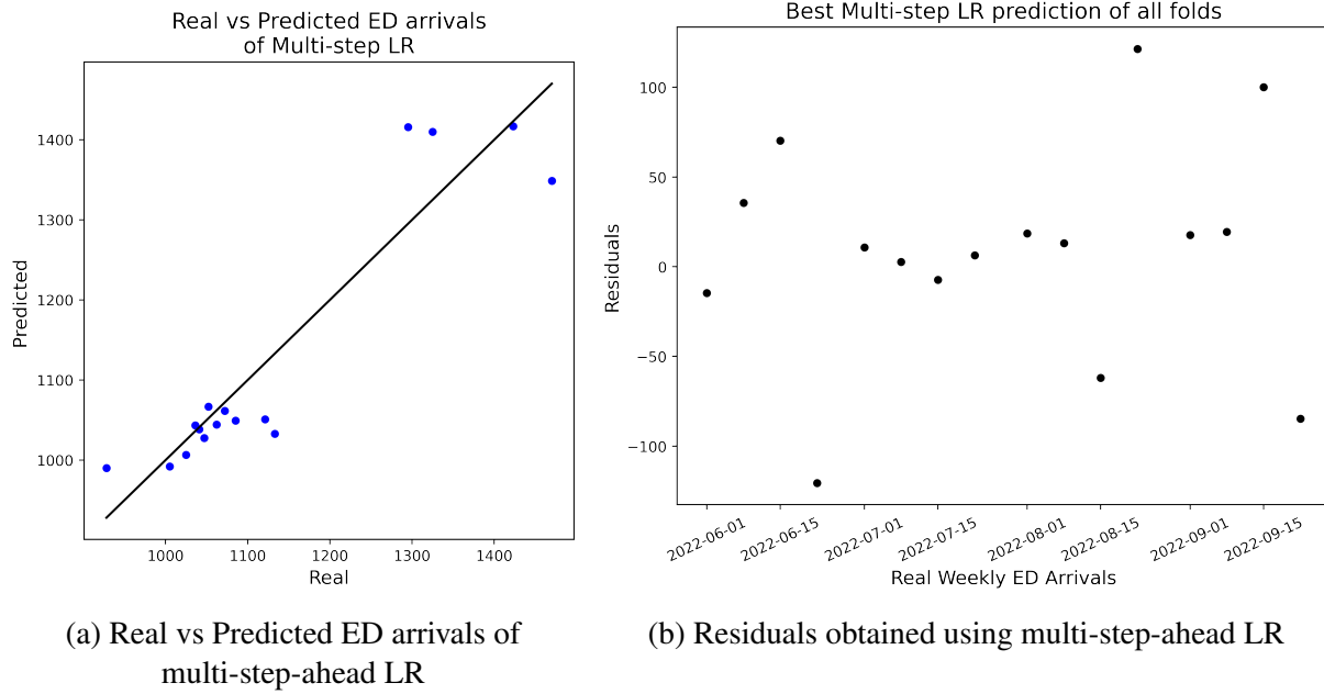
Figure 6.4: Multi-step-ahead LR residuals
