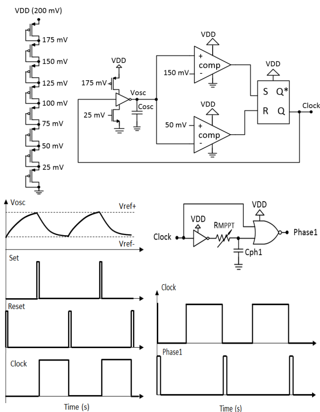
FIGURE 11. Circuits of Clock and Phase 1 signals.
