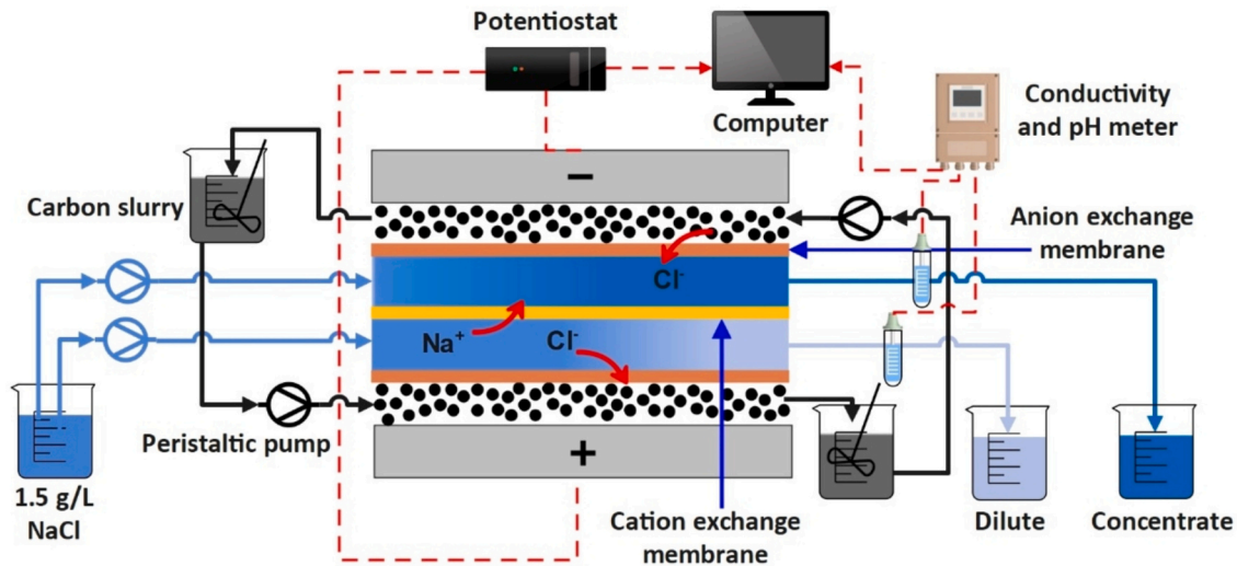
Fig. 3. The schematic diagram of the FCDI set-up used in desalination experiments.
