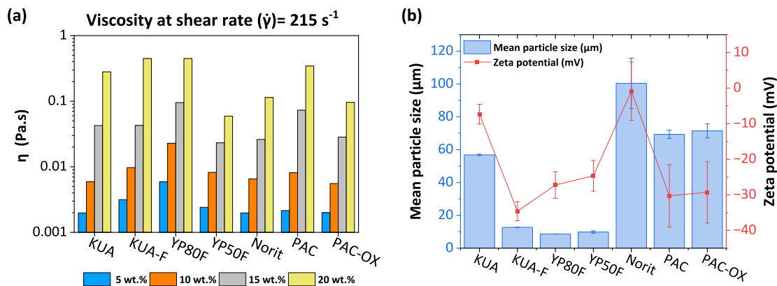
Fig. 7. (a) Viscosity of activated carbon at the shear rate of 215 \text{ s}^{-1} , (b) Mean particle size and zeta potential of activated carbons.
