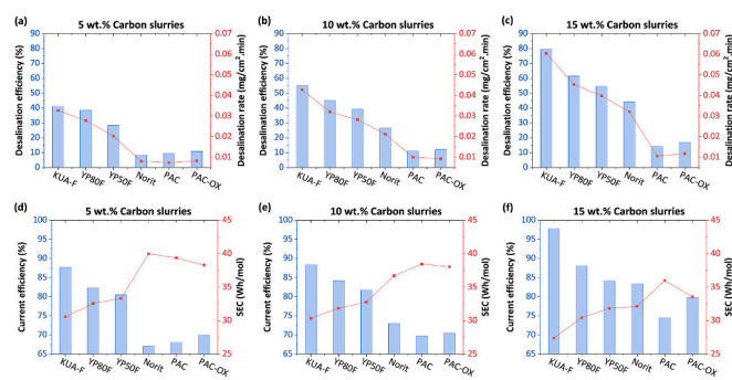
Fig. 9. Desalination efficiency and rate (a-c) and current efficiency and specific energy consumption (SEC) (d-f) at 5 wt%, 10 wt% and 15 wt% activated carbon loadings during desalination of a 1.5 g/L NaCl solution mimicking brackish water.
