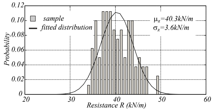
Figure 12. Fitting the resistance distribution for X_p=0\% .
