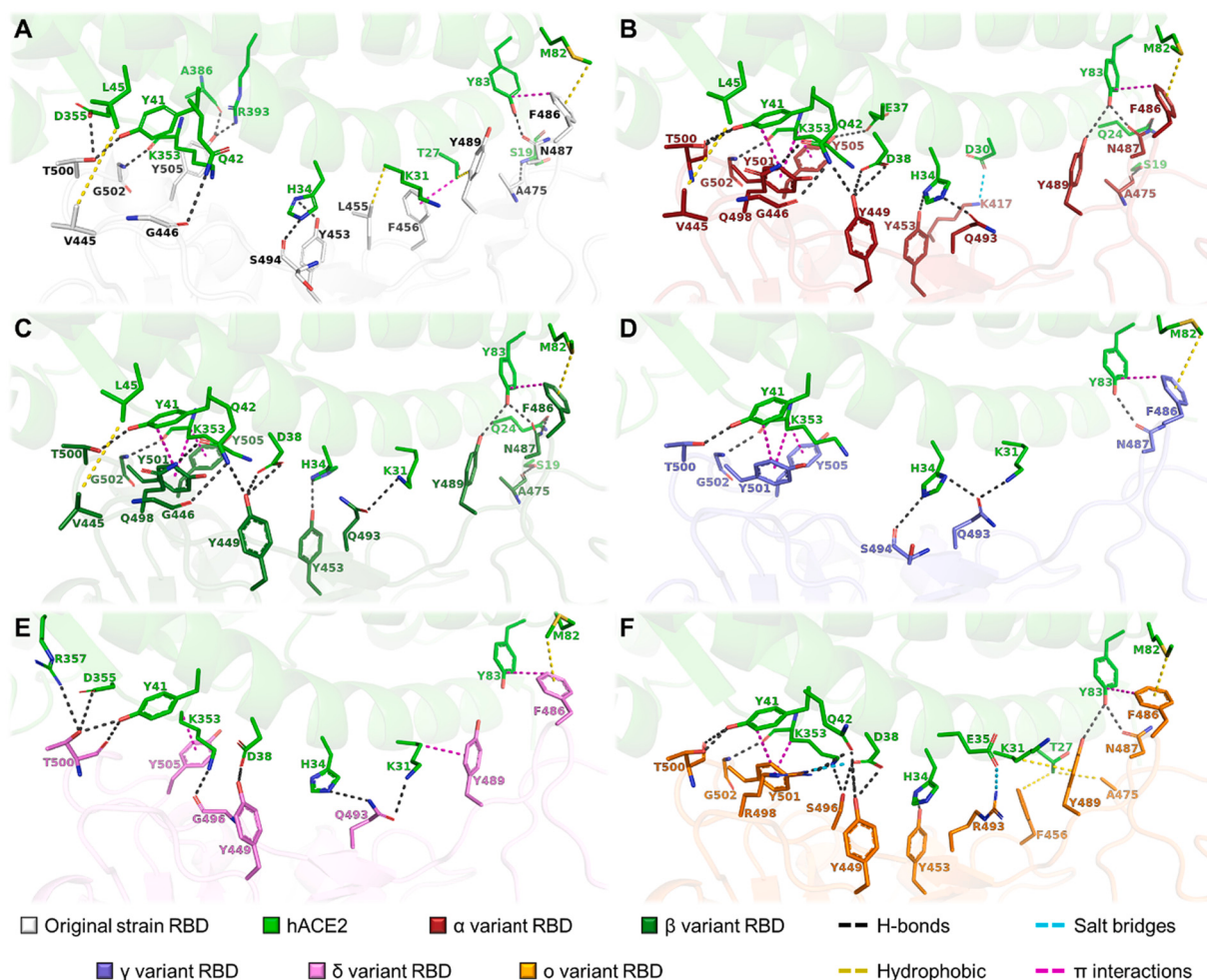
Fig. 3. Intermolecular interactions between the native ligand hACE2 (green) and the RBD pertaining to the (A) original strain (white) (PDB 7DF4), (B) \alpha variant (dark red) (PDB 7EFK), (C) \beta variant (dark green) (PDB 7EKG), (D) \gamma variant (slate blue) (PDB 7V84), (E) \delta variant (violet) (PDB 7V8B) and (F) \omicron variant (orange) (PDB 7T9L). Hydrogen bonds are represented as black dashed lines, salt bridges as cyan, hydrophobic interactions as yellow and \pi interactions as magenta. (For interpretation of the references to colour in this figure legend, the reader is referred to the web version of this article.)
