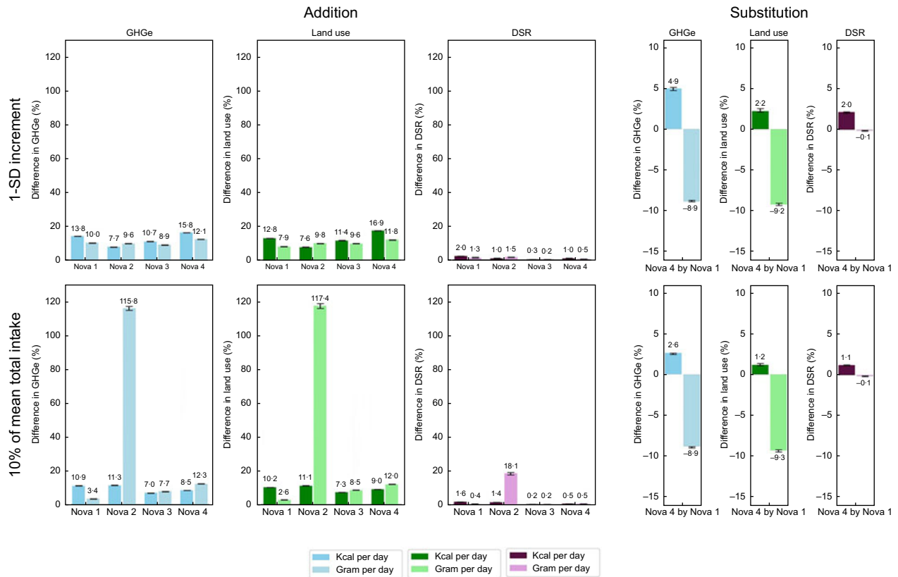
Figure 1. Linear association between the consumption of each Nova class and dietary greenhouse gas emissions (GHGe), land use and DSR. The left panel shows the additive estimates for 1 sd or 10% of mean total absolute intake increase in consumption (95% confidence intervals) across Nova classes, while the right panel presents substitution estimates for 1-sd or 10% of mean total absolute intake substitution of Nova 4 for Nova 1 among 368 733 adults enrolled in the European Prospective Investigation into Cancer and Nutrition (EPIC) study. Nova 1: unprocessed or minimally processed foods, Nova 2: processed culinary ingredients, Nova 3: processed foods and Nova 4: ultra-processed foods. Additive models were mutually adjusted for each Nova class. Substitution models were adjusted for Nova 1, 2, 3 and total intake. Both models were also adjusted for socio-demographic and anthropometrics covariates including: age at recruitment (years), BMI (kg/m 2 ), height (cm), sex (male, female), educational level (none, primary school, secondary school/technical school, higher education, unknown), smoking status at baseline (never, former, current and unknown), physical activity (Cambridge index; inactive, moderately inactive, moderately active, active and unknown) and alcohol intake (non-drinker, > 0–6, > 6–12, > 12–24 and > 24 gram per day), and centre was included as a random intercept. For consumption in kcal per day, the sds are 271.6 for Nova 1, 145.2 for Nova 2, 336.0 for Nova 3 and 394.11 for Nova 4. For consumption in gram per day, the sds are 833.3 for Nova 1, 23.5 for Nova 2, 308.1 for Nova 3 and 264.3 for Nova 4. The 10% of the mean total absolute intake in kcal per day was 218.8 and 281.9 for total absolute intake in gram per day. Substitution models substituted 1-sd of Nova 4 with an equivalent amount of Nova 1. All P values < 0.001. To facilitate direct comparison, the same y-axis scale was used for both 1sd and 10% increment estimates. This may reduce visual contrast for smaller effect sizes but improves interpretability across models.
