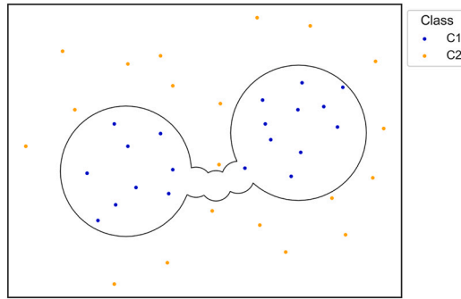
Fig. 5. Boundary of the connected cloud of spheres.
