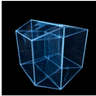
Fig. 1. An image from the 3D projection of a Tesseract performing a simple rotation about a plane in 4-dimensional space.
