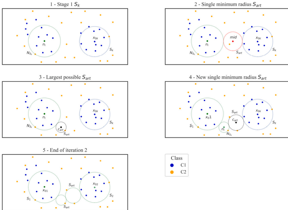
Fig. 14. Generation of artificial spheres at iteration 2 for the Separation data set.
