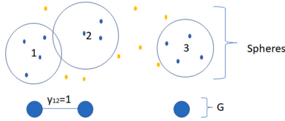
Fig. 6. Graph induced by the spheres.
