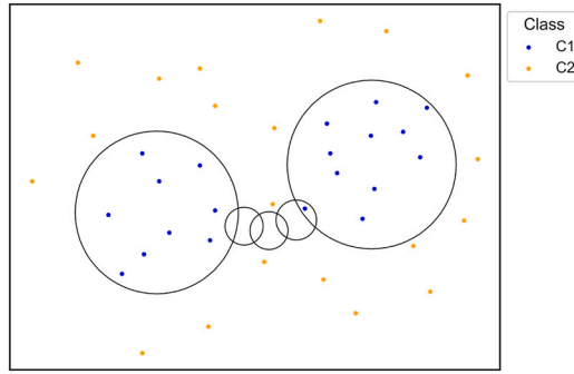
Fig. 4. Connected cloud of spheres.
