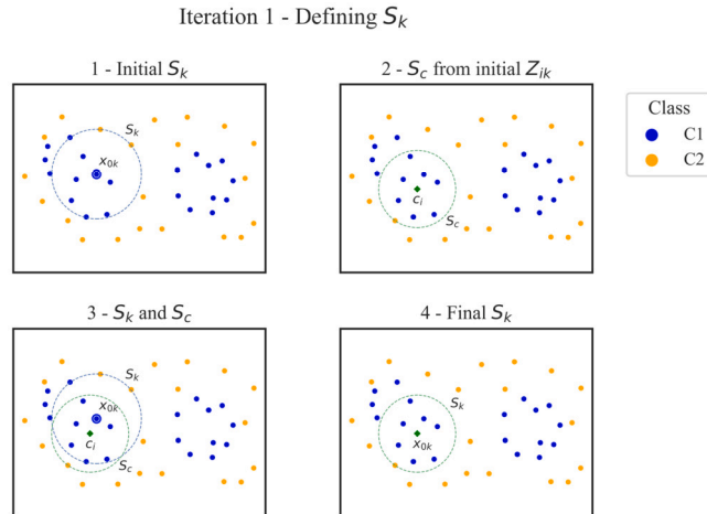
Fig. 13. Generation of S_k at iteration 1 for the Separation data set.
