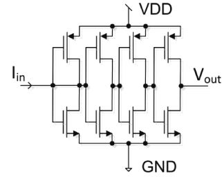
Fig. 4. Schematic diagram of the proposed comparator
