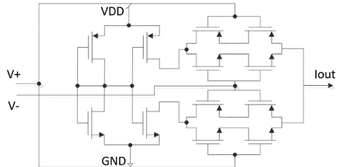
Fig. 5. Schematic diagram of the D/A current mode converter
