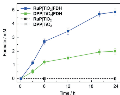
Figure 4. Photocatalytic \text{CO}_2 reduction to formate with FDH in a colloidal dye-sensitized \text{TiO}_2 system. Conditions: 12 nM FDH , 10 mM DTT, 0.83\text{ mg mL}^{-1} \text{TiO}_2 , 16.7\text{ }\mu\text{M} dye ( RuP or DPP ), 100 mM TEOA, 100 mM \text{NaHCO}_3 , pH 6.5, 25^\circ\text{C} , total volume: 1.0 mL, assembled in an anaerobic glove box, UV-filtered simulated solar-light irradiation: 100\text{ mW cm}^{-2} , AM 1.5G, \lambda > 420\text{ nm} . Error bars correspond to standard deviation ( N=3 ). Dashed traces show control experiments in the absence of FDH .
