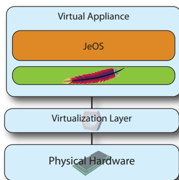
Figure 2.1: Virtual appliance
