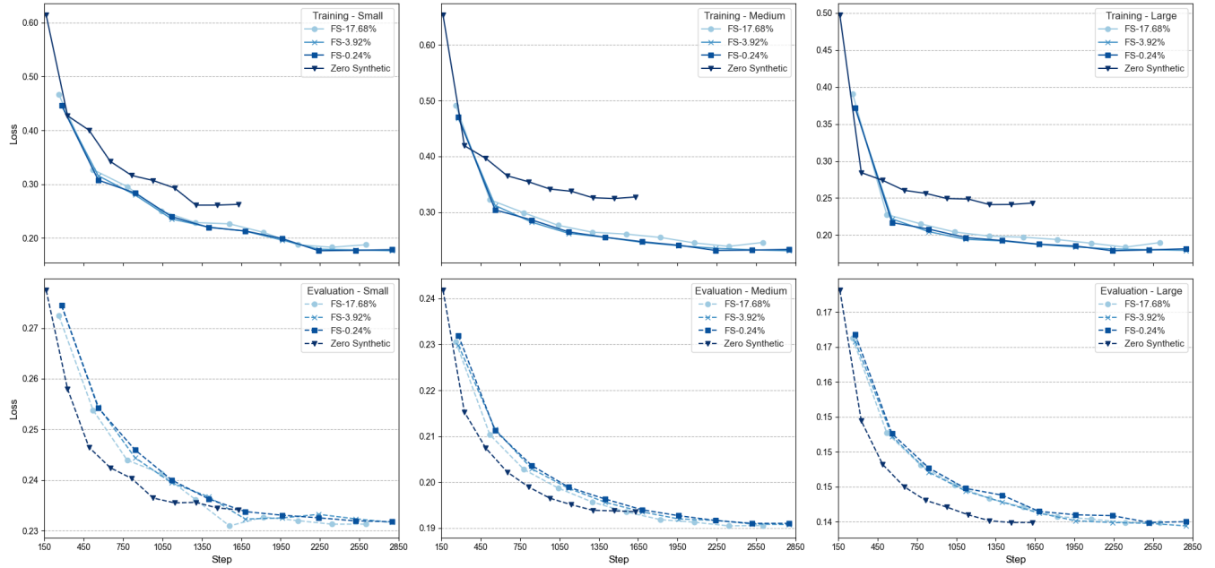
FIGURE 4. Training and evaluation losses of Whisper models fine-tuned on filtered synthetic data FS settings and Zero-Synthetic. The top row represents the training loss curves. The bottom row shows the corresponding evaluation loss curves. Due to the smaller dataset size, the Zero-Synthetic configuration completed fine-tuning earlier. The FS-0.24% configuration, with the most synthetic data retained, required the longest training time. Refer to Table 2 for details on the composition of each dataset.
