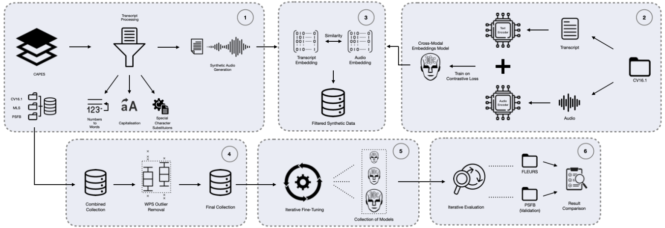
FIGURE 2. Detailed Methodology Overview: The process begins with the collection and preprocessing of transcripts for synthetic audio generation. The second step employs a contrastive learning approach for the cross-modal embedding model. In the third step, this model calculates the similarity between the synthetic audio and corresponding transcripts, creating several subsets of filtered data. The fourth step involves final preprocessing based on words per second (WPS) for the combined audio collection, which includes both synthetic and real data. The fifth step outlines the iterative fine-tuning process applied to each data subset (filtered and unfiltered). Finally, the last step demonstrates the evaluation of each model on two distinct data subsets.
