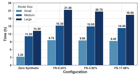
FIGURE 5. Runtime in hours for conducting each experiment, based on the specified model size.
