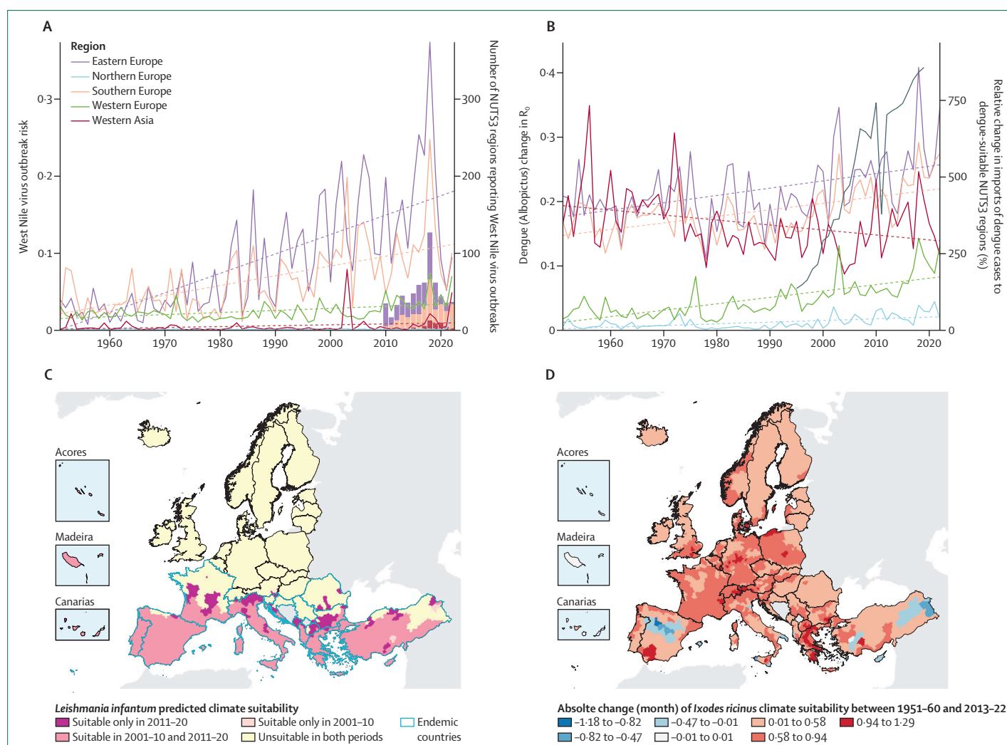
Figure 3: Climatic suitability for West Nile virus, dengue, Leishmania infantum , and Ixodes ricinus ticks in Europe
