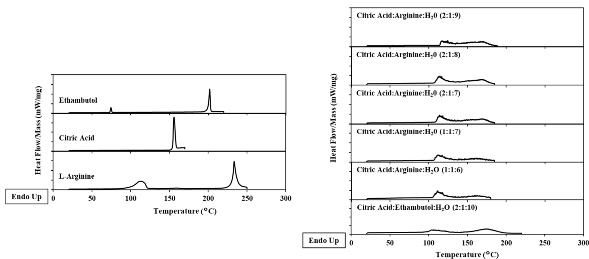
Figure 2. Thermograms obtained in hermetic capsules of initial components (a) and THEDES (b).
