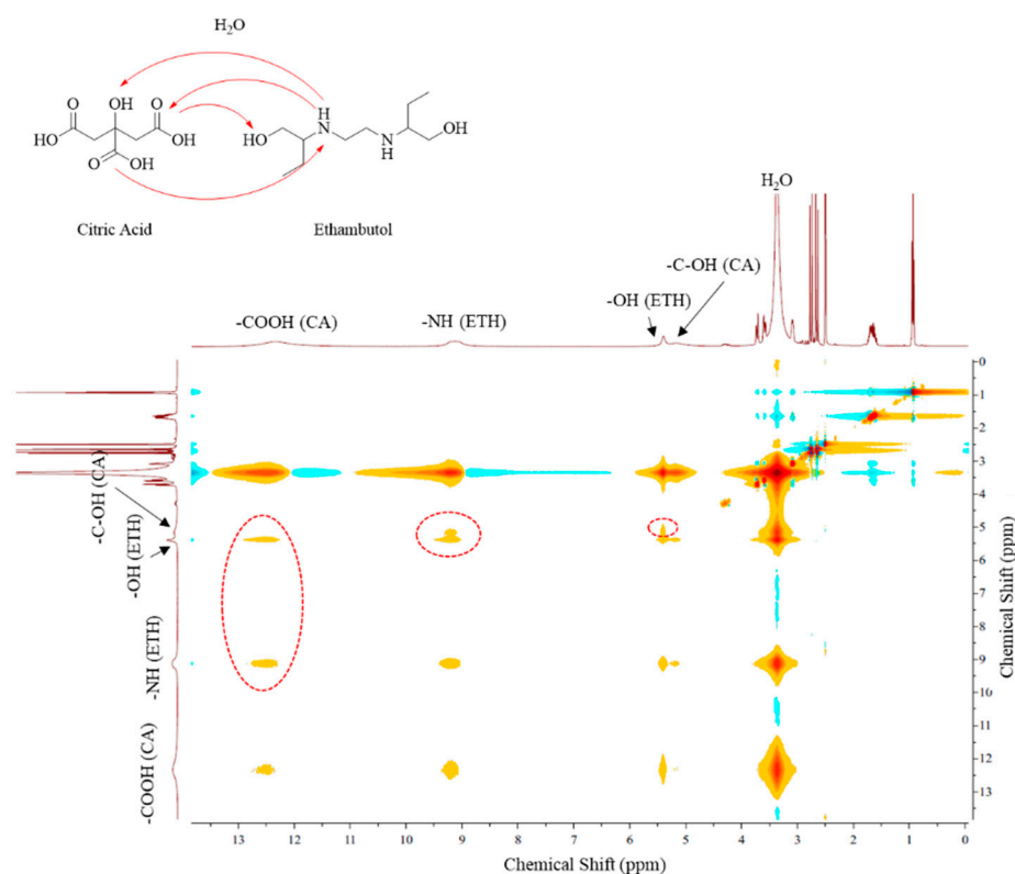
Figure 3. ^1\text{H} - ^1\text{H} -nuclear Overhauser enhancement spectroscopy (NOESY) with detected interactions between citric acid and ethambutol.
