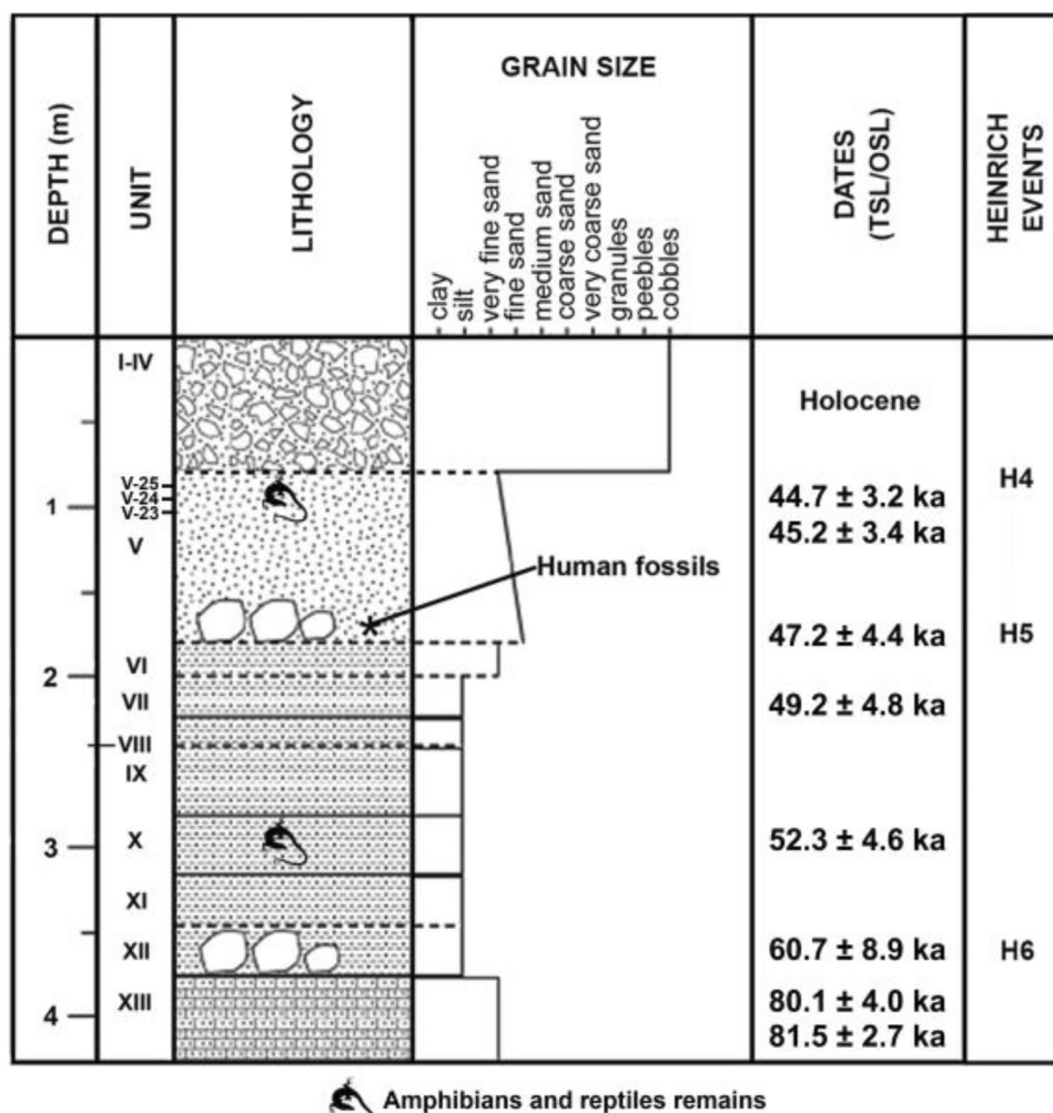
Fig. 4 Lithostratigraphic column of El Salt showing the different Stratigraphic Units (SU) described by Fumanal (1994), lithology of each SU and its proposed datation (Galván et al., 2014). Modified from Garralda et al. (2014)
