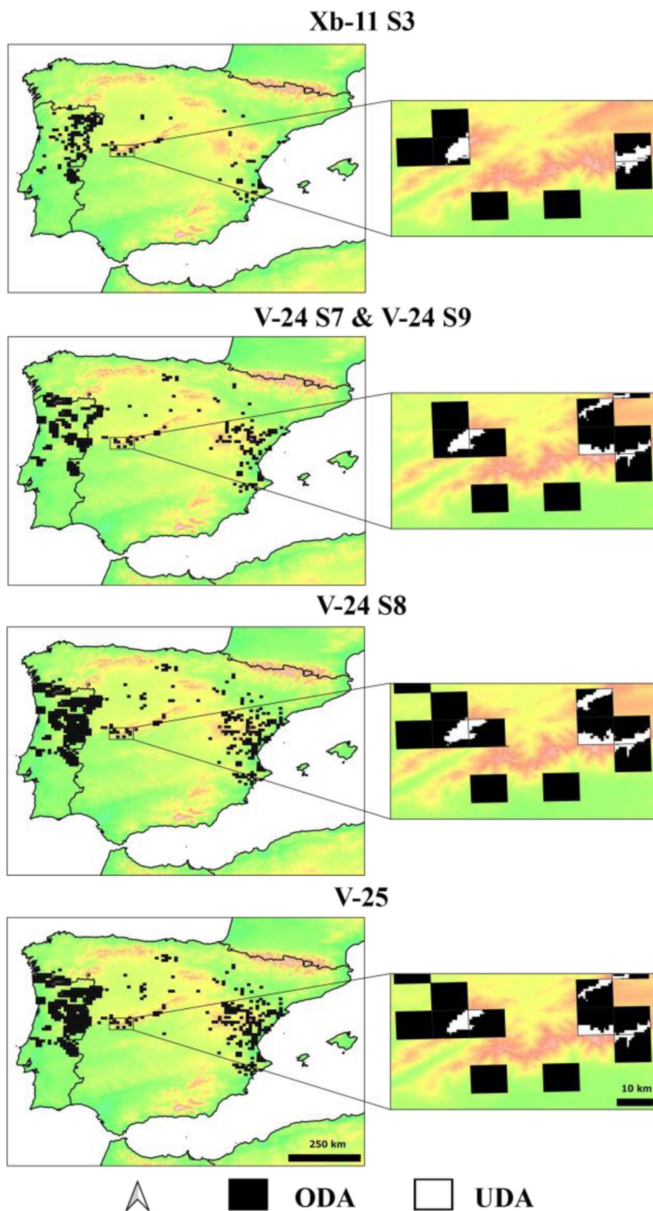
Fig. 6 Common distribution areas for the different assemblages of fossil herpetofauna from El Salt site denoted as 10 \times 10 km UTM square grids. The ODA (black area) and UDA (white area) is indicated in each square
