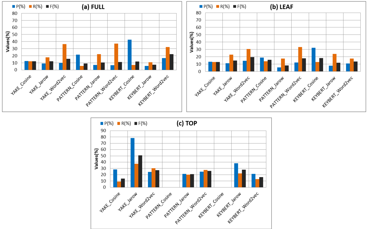
Figure 21: P (%), R (%) and F (%) values for NLP based tool employed for ranking-based evaluation method for (a) FULL (b) LEAF and (c) TOP approaches.
