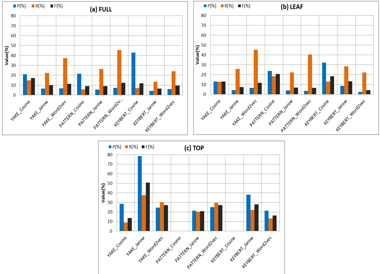
Figure 17: P (%), R (%) and F (%) values for NLP based tool employed for direct matching evaluation method for (a) FULL (b) LEAF and (c) TOP approaches
