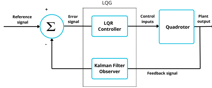
Figure 2.1: Block diagram of an LQR controller with Kalman Filters applied to a quadrotor (adapted from [10])
