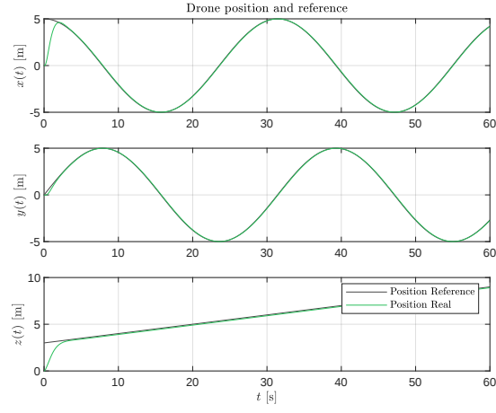
Figure 5.5: Position overtime in X, Y, and Z
