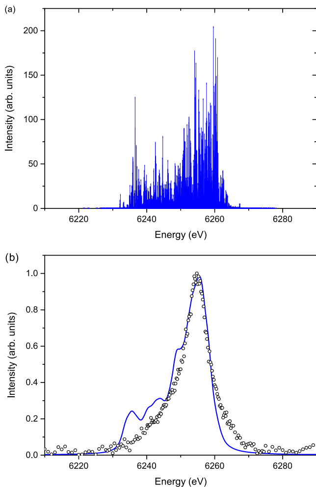
FIGURE 5 (color online) (a) Theoretical stick spectrum of the K^h\beta_{1,3} transition. The positions of the sticks correspond to the energies of the different hypersatellite components and their heights to the transition probabilities of the latter. (b) Comparison between the simulated K^h\beta_{1,3} hypersatellite spectrum (blue solid line) with the experimental one (open circles). The theoretical spectrum was obtained by summing all Voigtians attached to the components of the stick spectrum
