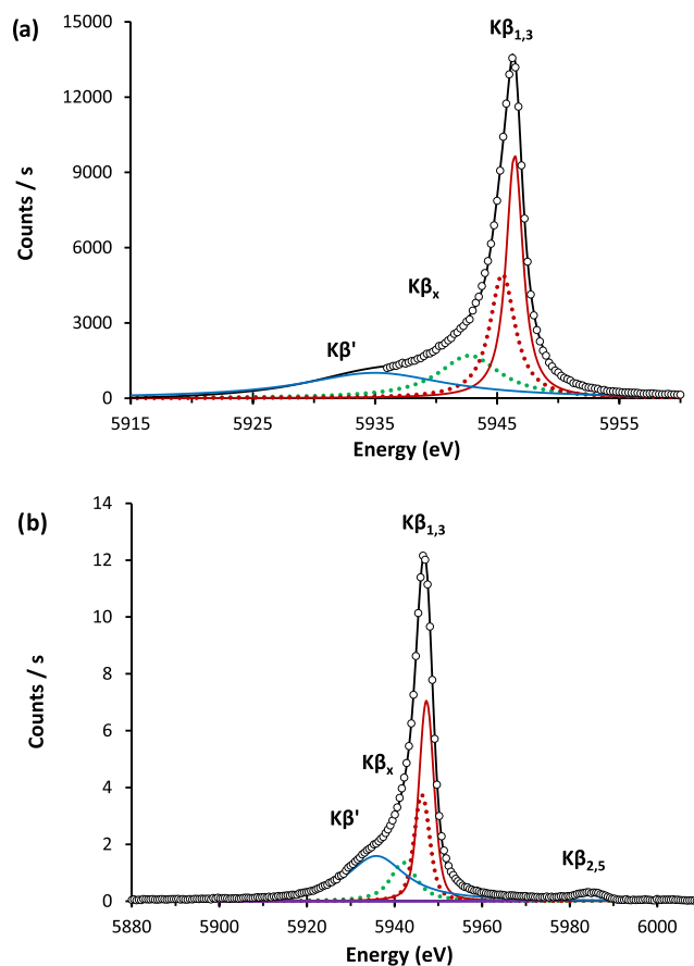
FIGURE 1 (color online) (a) Fit of the K\beta_{1,3} spectrum of Cr measured at Stanford Synchrotron Radiation Lightsource (SSRL). Shown are the background subtracted experimental spectrum (open circles), the total fit (black curve) together with the four individual Voigt components of the fit: The red solid and red dotted lines for the main K\beta_{1,3} transition, the green dotted line for the K\beta_x transition, and the blue line for the K\beta' transition. (b) Same as (a) but for the K\beta_{1,3} spectrum measured in Fribourg. In the latter measurement, the energy range was extended to include the K\beta_{2,5} transition
