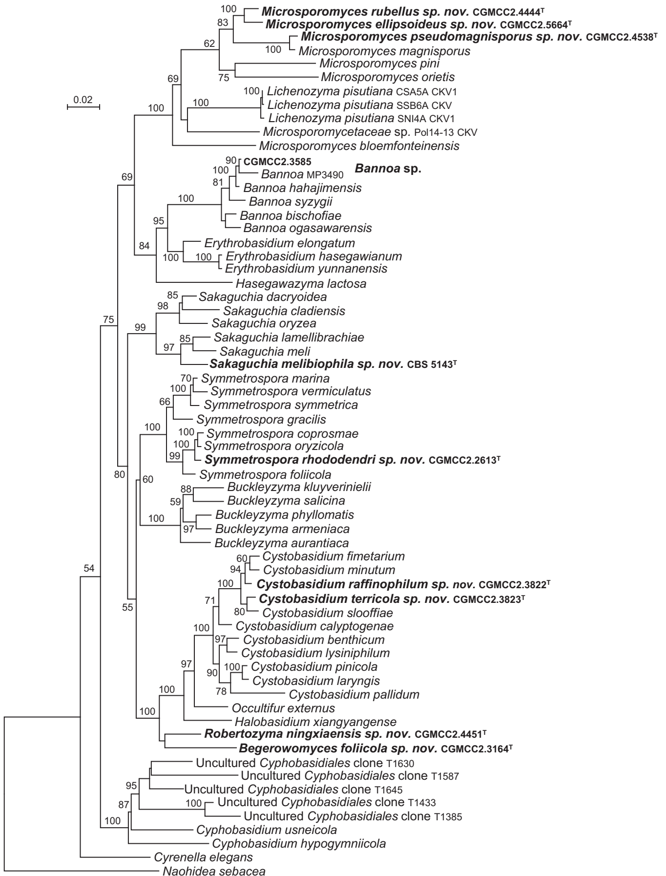
Fig. 6. Phylogenetic tree inferred using the combined sequences of SSU rDNA, LSU rDNA D1/D2 domains and ITS region (including 5.8S rDNA), depicting the phylogenetic positions of Lichenozyma and new taxa (in bold) within Cystobasidiomycetes ( Pucciniomycotina ). The tree was constructed using maximum likelihood analysis and over 50 % from 1 000 bootstrap replicates is shown. Bar = 0.02 substitutions per nucleotide position.
