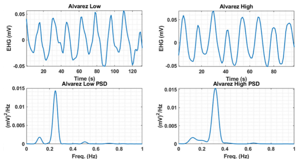
Fig. 2 AlvL (left column) and AlvH (right column) waveforms (top row) and Welch spectra (bottom row). The dominant frequency peak distinguishes both Alvarez types. The plots were obtained using the methodology presented in Esgalhado et al. (2020b)
