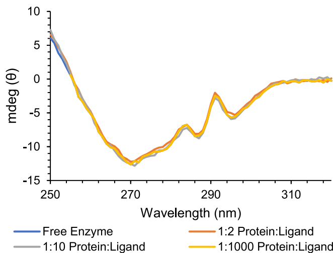
Fig. 5. Circular dichroism spectra in the Near-UV range of zinc(II)-WT-hCAII free and bound to increasing concentrations of sodium thiocyanate.
