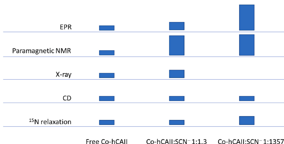
Fig. 7. Qualitative summary of the changes measured by the various experimental techniques for the free protein, the protein in the presence of stoichiometric amounts of thiocyanate, and the protein in thousand-fold excess of thiocyanate. The EPR data were acquired at 4 K, the X-ray at 110 K, and the NMR and CD at 298 K. The blue bars qualitatively reflect the observables of the different techniques, that are: the g-tensors values, for EPR; the axial and rhombic components of the magnetic susceptibility anisotropy tensor, for paramagnetic NMR; the coordination geometry of the metal, for X-ray; the global structure of the protein, for CD; the R_1 values for ^{15}\text{N} relaxation. (For interpretation of the references to colour in this figure legend, the reader is referred to the web version of this article.)
