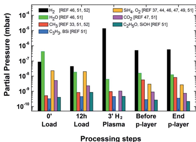
Fig. 5 Partial pressure histograms of the relevant species identified for the different stages of the silicon layers deposition, namely, immediately after loading the substrate in the PECVD system (0' load), after 12 h of vacuum pumping and baking at 145 °C (12 h load), at the end of the initial 3' H_2 cleaning plasma (3' H_2 plasma), before starting the deposition of the p-layer and with stabilized pressure (Before p-layer) and at the end of the p-layer deposition (end p-layer).
