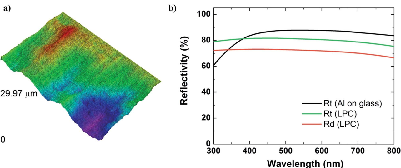
Fig. 2 Surface characterization analysis. (a) 3D profilometer on a 3 \times 2 \text{ mm} area; (b) total ( R_t ) and diffuse ( R_d ) reflection in the visible region of LPC and glass coated with aluminium.
