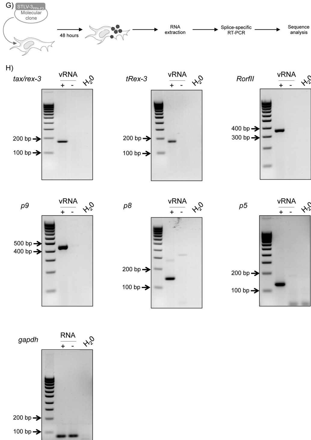
FIG 1 Characterization of STLV-3 pX mRNAs by splice-specific RT-PCR. (A) Strategy for amplifying unknown pX transcripts from 293T cells transfected with the STLV-3 PPA-F3 molecular clone or from STLV-3 PH969 -infected cells. Viral mRNAs, encoded by the pX region, were specifically reverse transcribed. cDNAs were amplified by PCR using forward primers (black arrows) located either in the 5' LTR or before the tax/rax splice donor site, while reverse primers (gray arrows) were located before the tax/rax-3 splice acceptor site. (B) RNAs extracted from STLV-3 PH969 -infected cells (viral RNA [vRNA]) were reverse transcribed by using Rev-7036 primers. cDNAs were amplified by using either Fwd-4984/Rev-7036 or Fwd-273/Rev-7036 primers. The white arrow indicates RorfII cDNA. (C and D) RNA extracted from 293T cells transfected with the STLV-3 PPA-F3 molecular clone (viral RNA) were reverse transcribed by using Rev-7173 primers. (C) cDNAs were amplified by using Fwd-316/Rev-6918 primers. All the bands were purified, cloned, and sequenced. The white arrow indicates the band corresponding to p9 cDNA. (D) cDNAs were amplified by using Fwd-316/Rev-7173 primers. All the bands were purified, cloned, and sequenced. The white arrow indicates the band corresponding to both p8 and p5. (E) Exon composition of the newly identified STLV-3 PPA-F3 RNAs. Other spliced viral RNAs are also shown. Numbers and arrows indicate splice sites. Boxes indicate ORFs, and asterisks represent positions of the start codon within each ORF. Putative proteins identified in this report were named according to the in silico prediction of their molecular weight. (F) Consensus motifs of mammalian splice donor (sd) and splice acceptor (sa) sites. The dinucleotides essential for these sites are underlined. Sequences of the identified functional splice donor and acceptor sites in viral mRNAs are aligned to the consensus. (G) RNA was extracted 48 h after transfection of 293T cells with the STLV-3 PPA-F3 molecular clone. (H) One-step RT-PCR was performed on 500 ng RNA extracted from STLV-3-transfected (+vRNA) or mock-transfected (-vRNA) 293T cells, using primers located on the splice junctions of tax/rax-3 , tRex-3 , RorfII , p9 , p8 , and p5 viral mRNAs. gapdh was used as a control.
