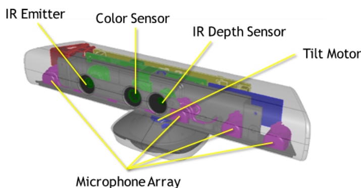
Figura 2.2: Sensor Kinect 3
