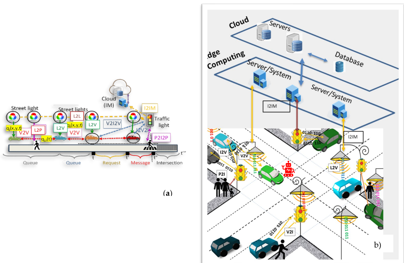
Figure 2. (a) Draft of the V-VLC architecture. Overview of visible light communication channels within the intersection area. (b) Illustration of the sensing transmission in road sensor networks. The diagram shows the three key components of the cooperative sensing framework: roadside infrastructure, sensing data aggregation, and sensing information delivery to CVs.
