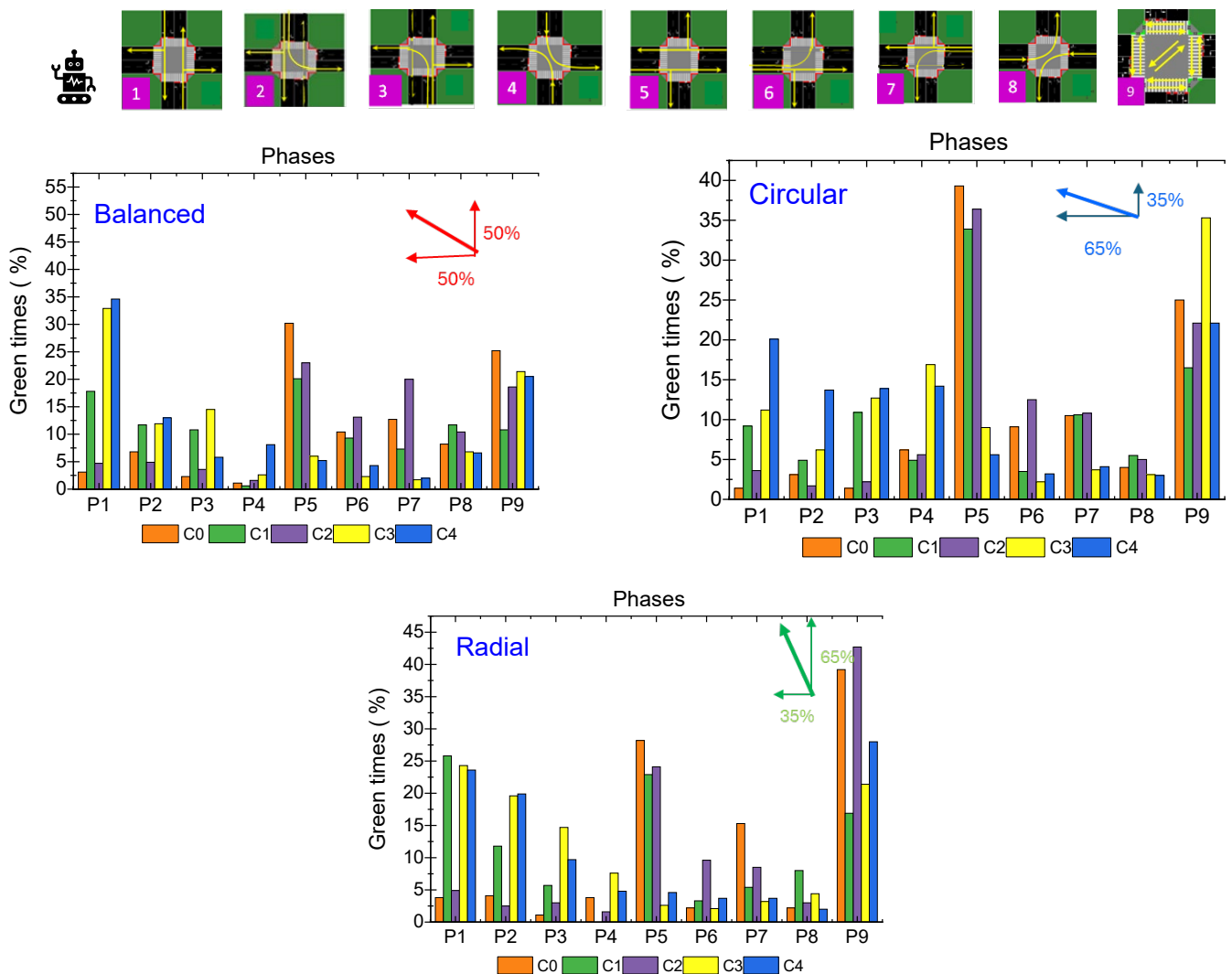
Figure 15. Analysis of the percentage of green time allocated to outbound traffic strategies at intersections C0–C4. Results are shown for Network 1, representing a balanced topology; Network 2 (Circular + Outbound Radial); and Network 4 (Radial + Outbound Radial).
