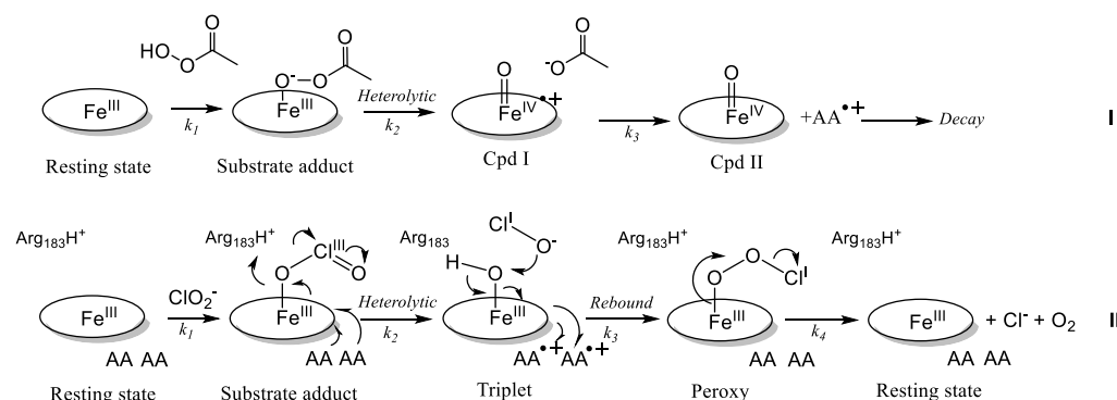
Scheme 2. Proposed Reaction Mechanism of the Reaction between AoCld and (I) Peracetic Acid (II) Chlorite Based on Direct Spectroscopic Evidence Presented in This Work a
