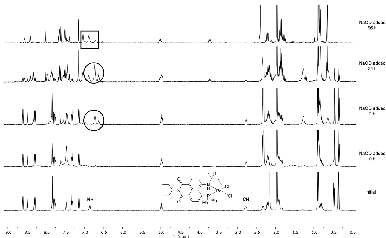
Figure 5. ^1\text{H} NMR spectra in \text{CD}_3\text{CN} of complex 6 in the absence and at different reaction times after the addition of 1.0 equiv. of NaOD.
