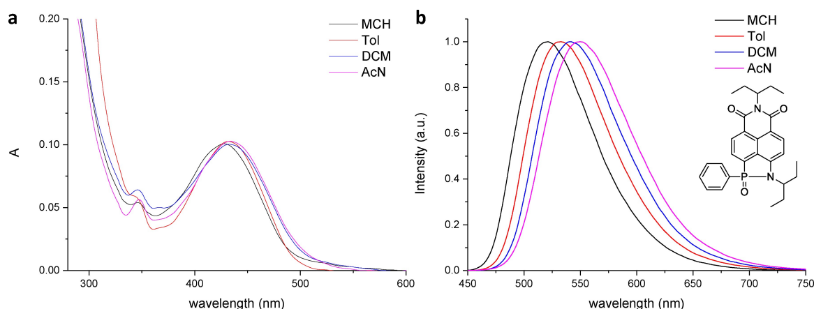
Figure 6. Absorption (a) and emission (b) spectra of isolated compound C in organic solvents. \lambda_{\text{exc}} = 420 nm.
