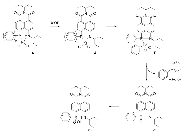
Scheme 6. Proposed mechanism for the base promoted transformation of complex 6 to cyclic phosphorylamide C and phosphinic acid D .
