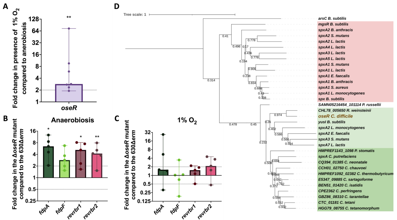
FIG 6 The Spx-like regulator, OseR, regulates the genes encoding the O 2 -reductase in response to O 2 . The expression of the oseR gene in the 630Δ erm strain exposed for 48 h to 1% O 2 and in anaerobiosis was compared by RT-qPCR (A). The expression of the genes encoding the four O 2 -reductases was measured by RT-qPCR in the Δ oseR and the 630Δ erm strain grown for 48 h on agar plates in anaerobiosis or at 1% O 2 . Fold changes correspond to the ratio between the RNA extracted from cells of the Δ oseR mutant and the 630Δ erm strain in anaerobiosis (B) or at 1% O 2 (C). Medians with 95% CI are shown. Five biological replicates were performed for each experiment. The sequence of known Spx and Spx-type proteins of Firmicutes was aligned with the sequence of OseR of C. difficile and a dendrogram was constructed (D). Two sub-families are visible: highlighted in red, the canonical Spx and highlighted in green are Spx-like proteins of the Yusi subfamily, including OseR (in brown) with two sub-families: in light green, the Yusi-like subfamily and in dark green the other proteins of the Yusi subfamily found in Clostridia. Mann-Whitney statistical tests were performed between the ΔCt of the two conditions compared. *: P -value < 0.05; ** < 0.01.
