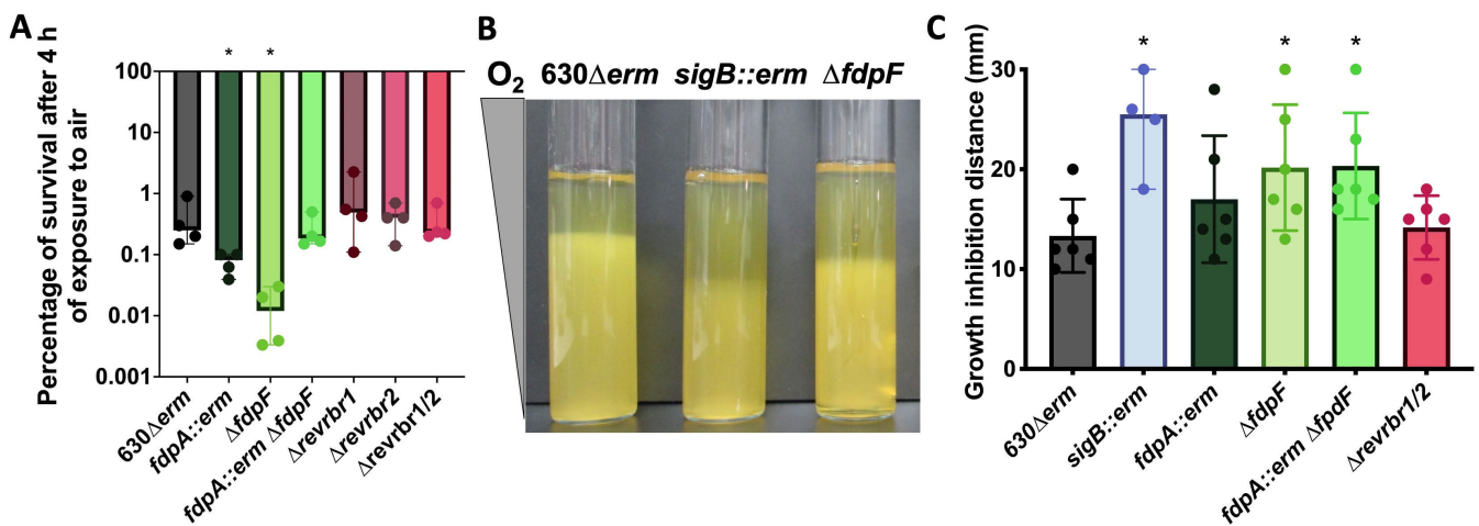
FIG 2 Role of O 2 -reductases in the tolerance to air. Serial dilutions of the 630Δ erm and the mutants were spotted on TY Tau plates. Plates were incubated either in anaerobiosis for 24 h, or in the presence of air for 4 h (Fig. S2A). Plates incubated in air were subsequently incubated in anaerobiosis for 24 h. CFUs were determined for each experiment and the percentage of survival after exposure to air relative to the survival in anaerobiosis was plotted (A). Soft agar tubes were inoculated with various strains and incubated in air (B). The growth inhibition distance for each replicate was determined and plotted (C). At least four biological replicates were performed per experiment. For all plots, a median with 95% CI is shown. Mann-Whitney statistical tests were performed. All comparisons were made with the 630Δ erm strain. *: P -value < 0.05.
