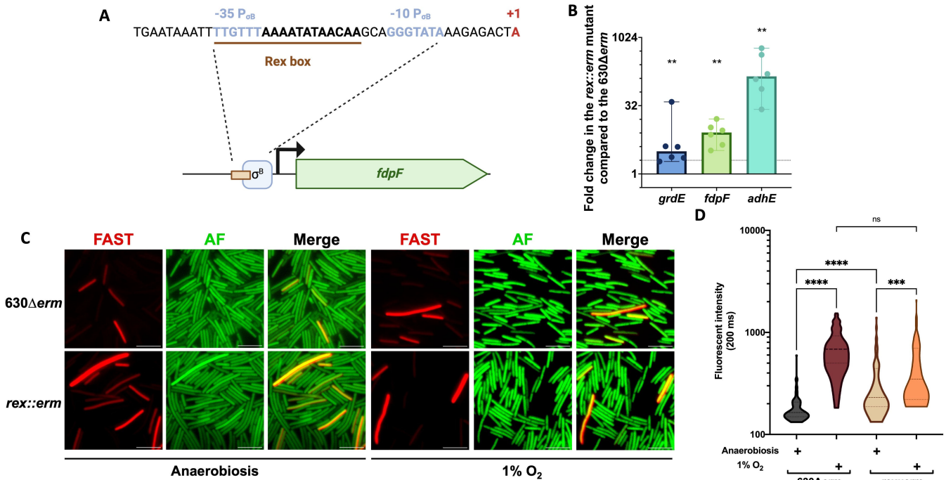
FIG 7 The control of fdpF gene expression by Rex. The identified Rex binding box in the promoter region of fdpF and the \sigma^B -dependent promoter are indicated (A). To confirm the regulation of fdpF by Rex, RT-qPCR experiments were performed on RNA extracted from the rex::erm mutant and the 630Δerm strain grown for 48 h on agar plates in anaerobiosis (B). Six biological replicates were performed. Medians with 95% CI are shown. Expression of fdpF was also tested using a transcriptional fusion between the promoter P_{(fdpF)} and the SNAP cd fluorescent reporter gene introduced into the 630Δerm strain and the rex::erm mutant. Bacteria were grown for 48 h on agar plates in anaerobiosis or at 1% O 2 . Autofluorescence (AF), SNAP fluorescence, and merge are shown (C). Quantification of the fluorescence intensity of the SNAP reporter of images in panel C was performed (D). 600 bacteria out of 2 independent experiments were quantified. Mann-Whitney statistical tests were performed for qPCR and one-way ANOVA for fluorescence intensity. *: P -value < 0.05; **: P <0.01; ***<0.001; ****<0.0001.
