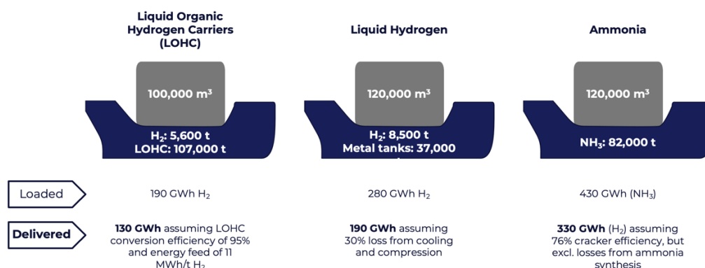
Figure 11: Energy and volumes in exemplary large long-range tankers | Source: Own Creation, following Guidehouse (2022)
