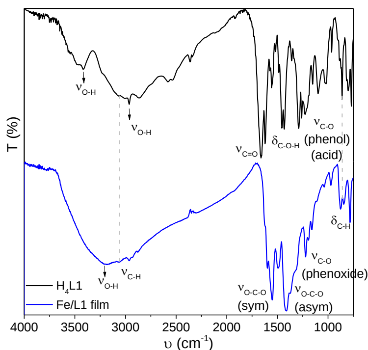
Figure 2.39 - FTIR spectrum of H 4 L1 (black) and DRIFT spectrum of the Fe/L1 film (blue) deposited at -1.3 V. Spectra were recorded in a range of 4000-500 cm -1 .
