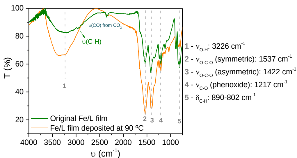
Figure A.77 - DRIFT spectra of the original (green) and the Fe/L film deposited at 90 °C (orange) Fe/L films (2:1:1 ratio of M:H 4 L:PB , respectively). Spectra were recorded in a range of 4000-750 cm -1 and the blank was measured with a gold coated plate.
