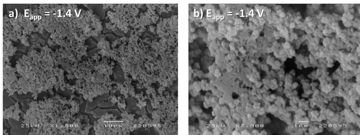
Figure A.55 - SEM images of the Fe/L film (2:1:1 ratio of M:H 4 L:PB, respectively) deposited at -1.4 V and magnified at a) x1500 and b) x7500.
