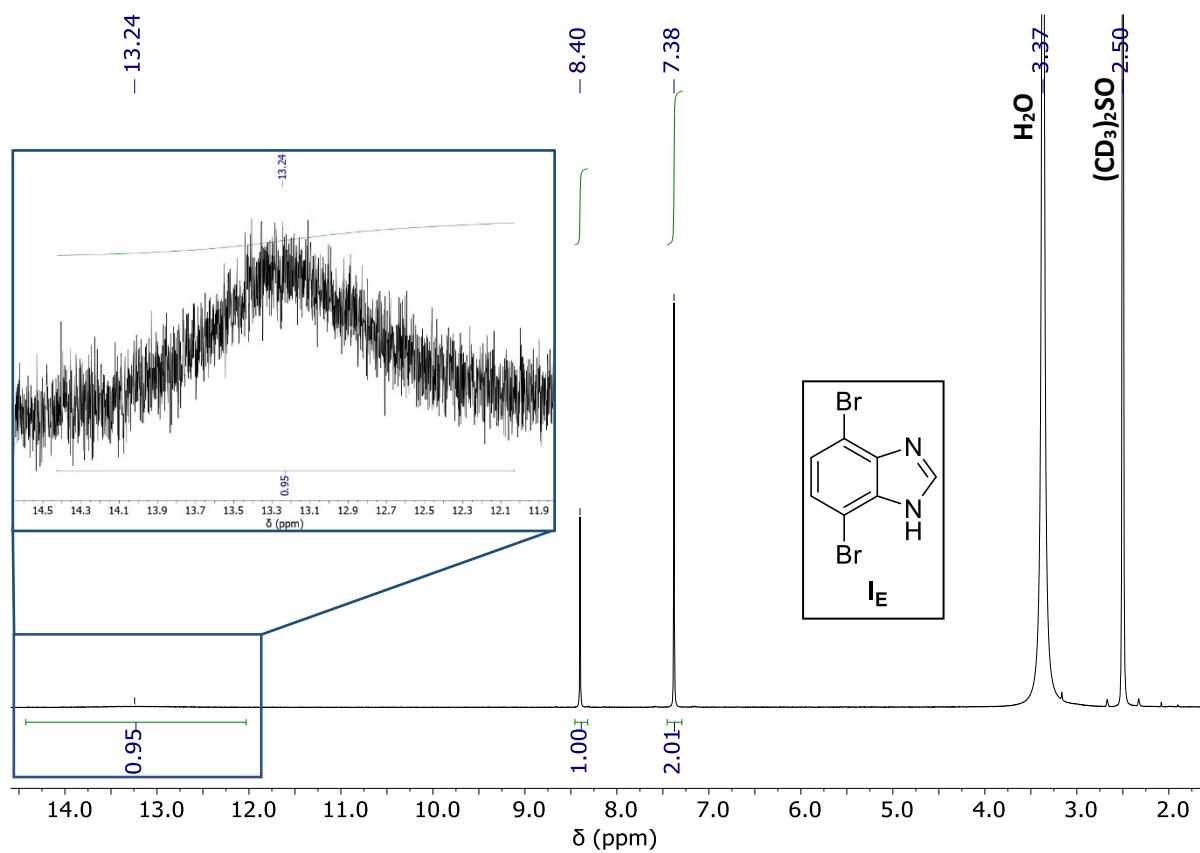
Figure A.12 - 1 H NMR spectrum of IE in (CD 3 ) 2 SO.
