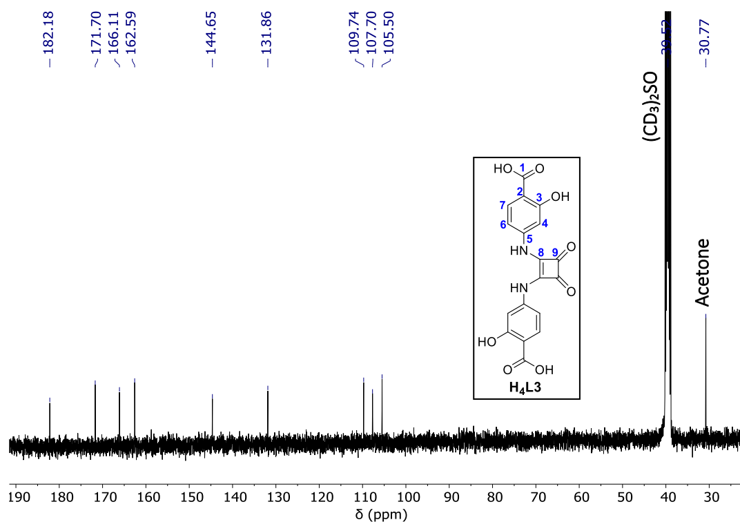
Figure 2.4 - 13 C NMR spectrum of H 4 L3 in (CD 3 ) 2 SO.
