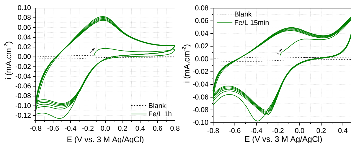
Figure 2.51 - Cyclic voltammograms of the 1-hour and 15-minute Fe/L films (2:1:1 ratio of M:H 4 L:PB , respectively) deposited on the FTO working electrode ( 0.7 \text{ cm}^2 ). CVs were performed in 10 mL of \text{N}_2 saturated 0.1 M of tris-HCl buffer and recorded at 100 \text{ mV.s}^{-1} . The one-compartment electrochemical cell was also constituted by platinum wire as counter and 3 M Ag/AgCl as reference electrodes.
