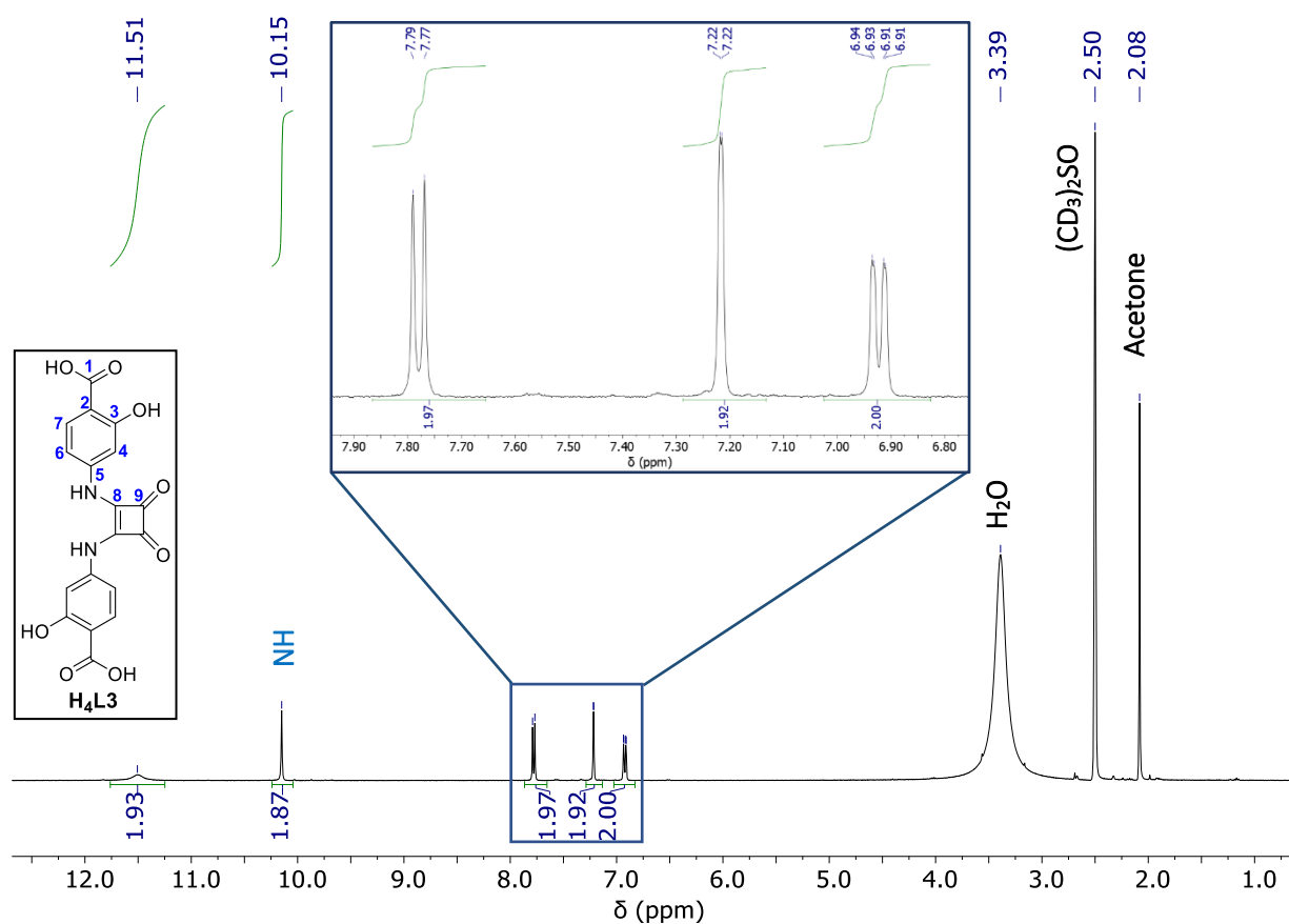
Figure 2.3 - 1 H NMR spectrum of H 4 L3 in (CD 3 ) 2 SO.
