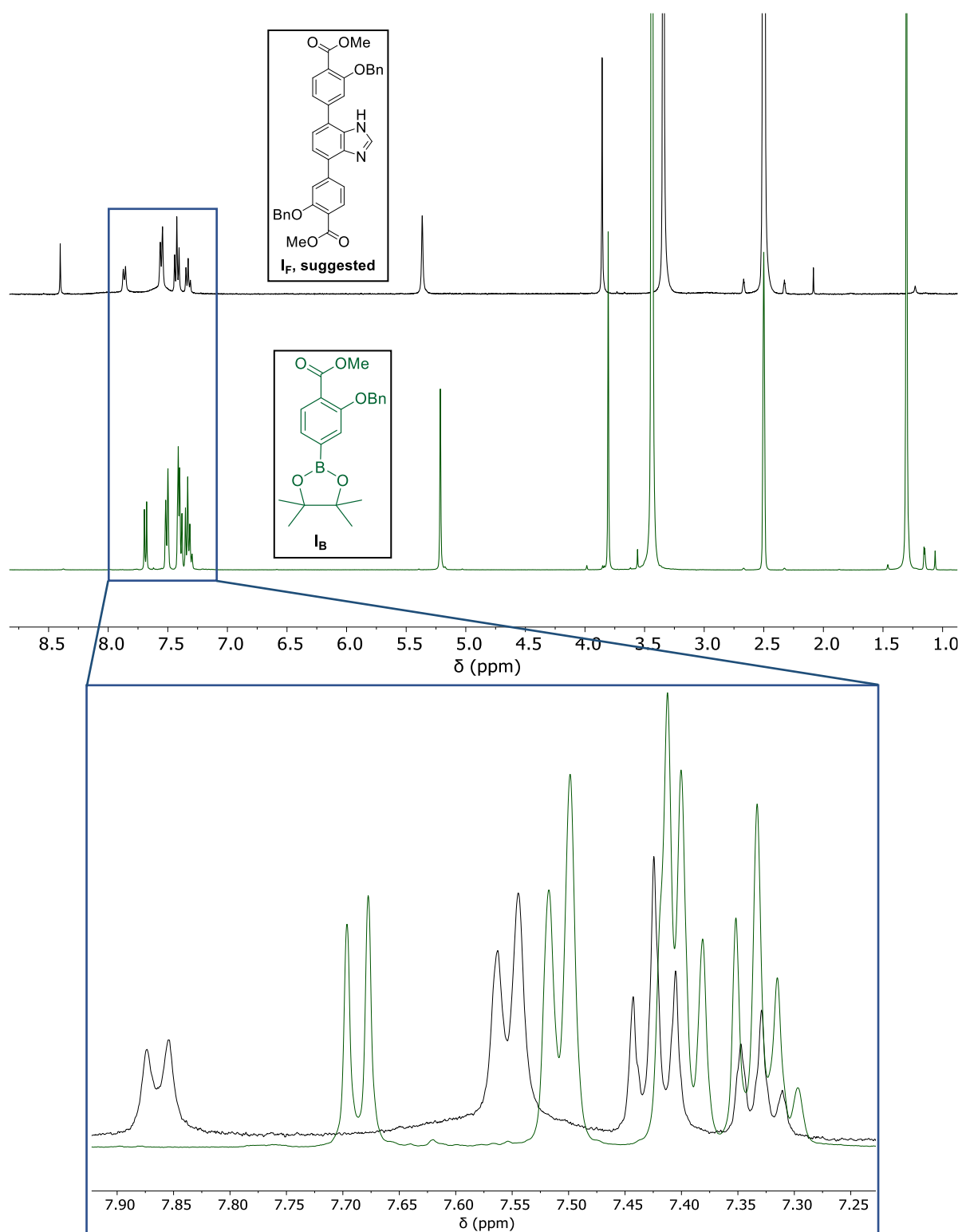
Figure A.16 - ^1\text{H} NMR stacked and superimposed spectra of IF (black) and IB (green) intermediate in (\text{CD}_3)_2\text{SO} .
