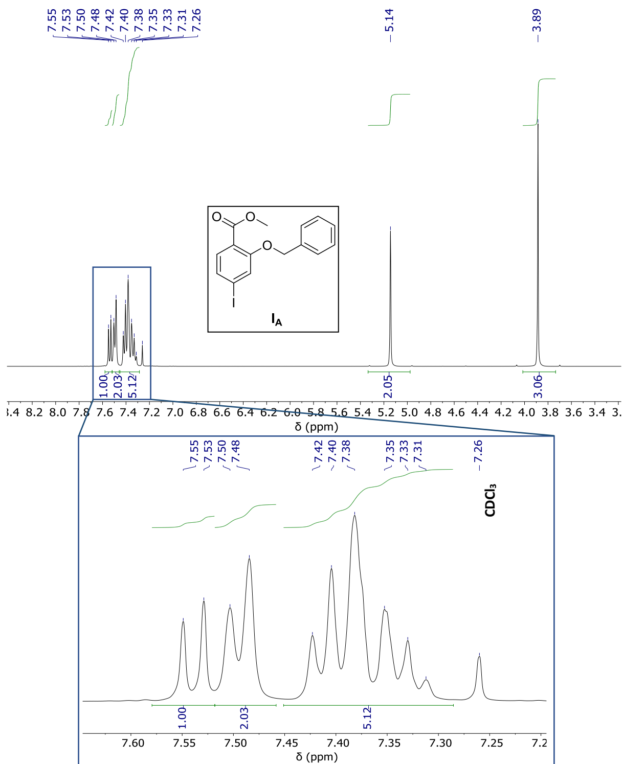
Figure A.2 - ^1\text{H} NMR spectrum of \mathbf{1_A} Intermediate in \text{CDCl}_3 .
