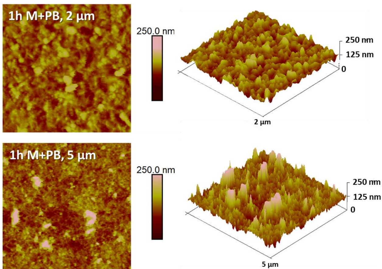
Figure A.72 - 2D and 3D AFM images of the M+PB film (2:1 ratio of M:PB , respectively) deposited at -1.3 V for 1 hour, with dimensions of 2x2 μm and 5x5 μm.
