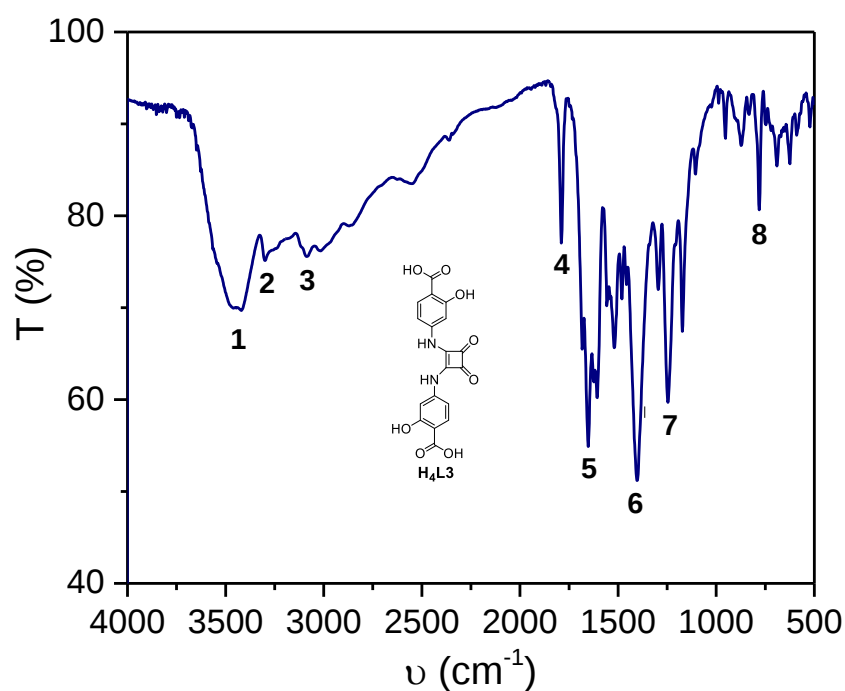
Figure A.28 - FTIR spectrum of H 4 L3 in KBr pellets. Spectrum was recorded in a range of 4000-500 \text{cm}^{-1} .
