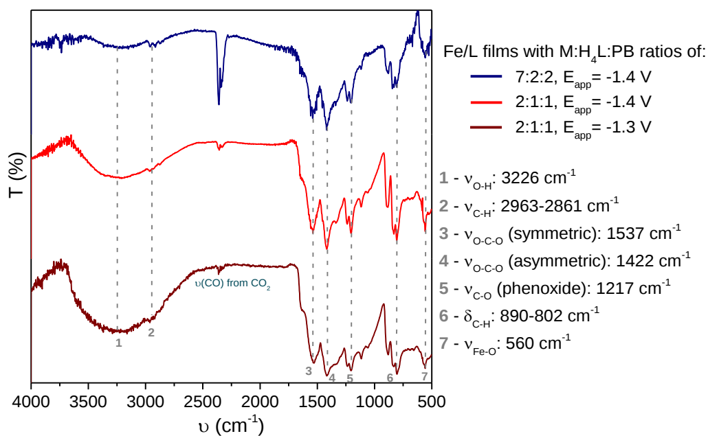
Figure A.54 - DRIFT spectra of the Fe/L film (7:2:2 ratio of M:H 4 L:PB, respectively) deposited at -1.4 V (blue) and the Fe/L films (2:1:1 ratio of M:H 4 L:PB, respectively) deposited at -1.4 (red) and -1.3 V (burgundy) for 1 hour. Spectra were obtained in a range of 4000-500 cm^{-1} and blank was measured with a gold coated plate.
