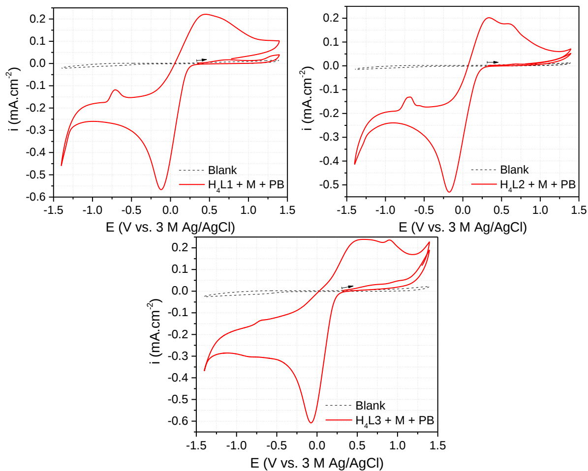
Figure A.88 - Cyclic voltammograms of a) H 4 L1+M+PB b) H 4 L2+M+PB and c) H 4 L3+M+PB . CVs were performed in 10 mL of N 2 saturated DMF with TBAPF 6 as the supporting electrolyte and recorded at 100 mV.s -1 . The one-compartment electrochemical cell was also constituted by FTO as working, platinum wire as counter and 3 M Ag/AgCl as reference electrodes. Species quantities: 4 mM of M , 2 mM of H 4 L1 , H 4 L2 or H 4 L3 and 2 mM of PB .
