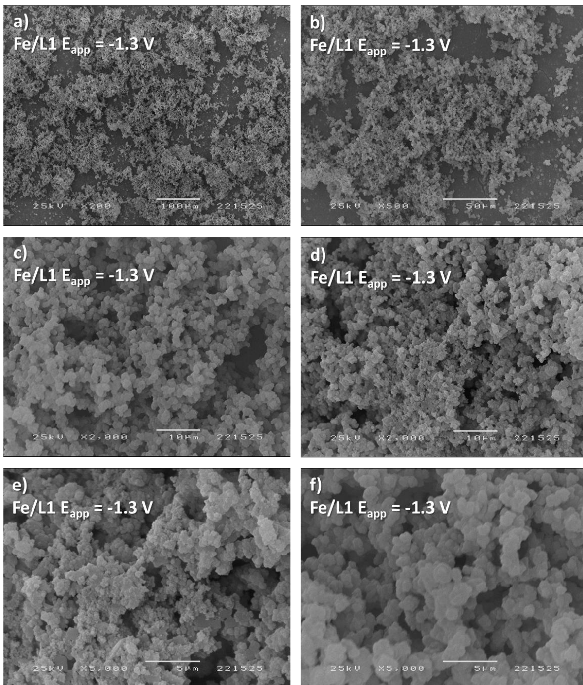
Figure A.91 - SEM images of the Fe/L1 film deposited at -1.3 \text{ V} , magnified at a) \times 200 , b) \times 500 , c) \times 2000 , d) \times 2000 , e) \times 5000 and f) \times 5000 .
