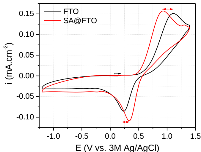
Figure 2.17 - Cyclic voltammograms of 1 mM of ferrocene with FTO ( black ) and SA@FTO ( red ) as working electrodes. Studies were performed in 10 mL of N 2 saturated DMF with TBAPF 6 as the supporting electrolyte and recorded at 100 mV.s -1 . The one-compartment electrochemical cell was also constituted by platinum wire as counter and 3 M Ag/AgCl as reference electrodes.
