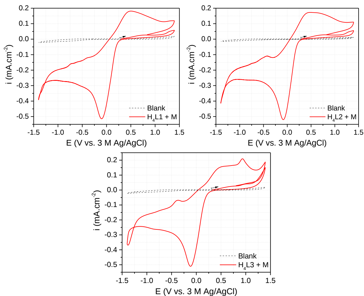
Figure A.87 - Cyclic voltammograms of a) H_4L1+M b) H_4L2+M and c) H_4L3+M . CVs were performed in 10 mL of N_2 saturated DMF with TBAPF_6 as the supporting electrolyte and recorded at 100 \text{ mV.s}^{-1} . The one-compartment electrochemical cell was also constituted by FTO as working, platinum wire as counter and 3 M Ag/AgCl as reference electrodes. Species quantities: 4 mM of M , 2 mM of H_4L1 , H_4L2 or H_4L3 .
