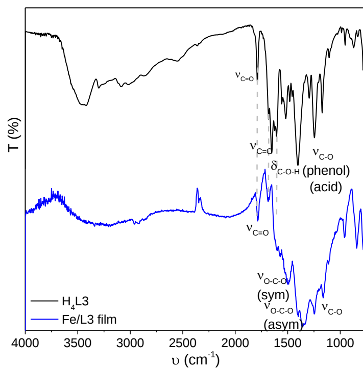
Figure A.90 - FTIR spectrum of H_4L3 (black) and DRIFT spectrum of the Fe/L3 film (blue) deposited at -1.3 V. Spectra were recorded in a range of 4000-500 cm^{-1} .
