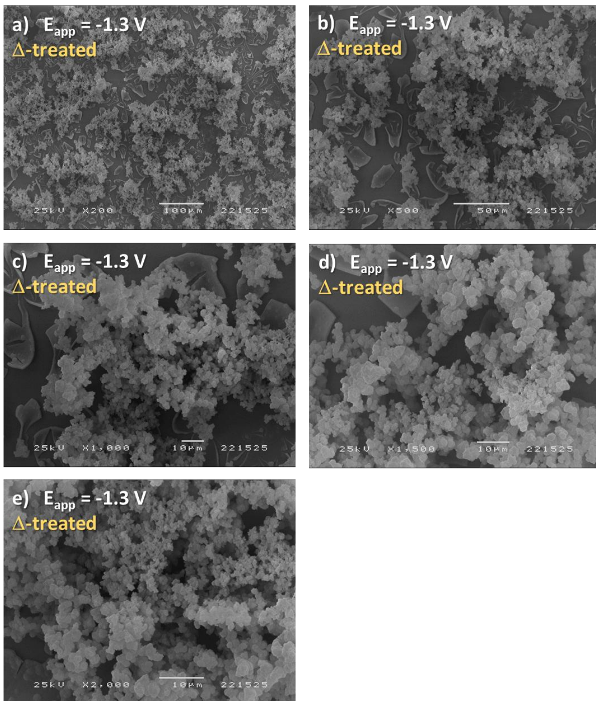
Figure A.58 - SEM images of the temperature-treated Fe/L film (2:1:1 ratio of M:H 4 L:PB , respectively) deposited at -1.3 V, magnified at a) x200, b) x500, c) x1000, d) x1500 and e) x2000.
