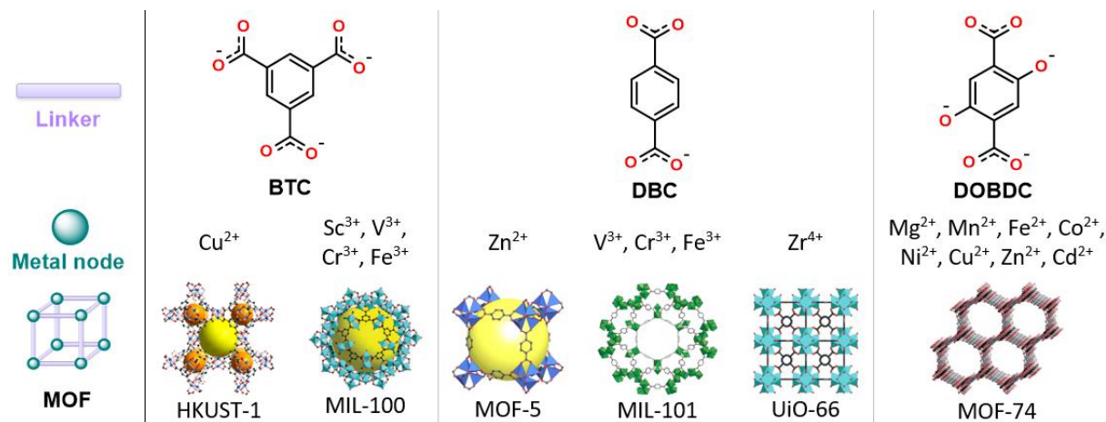
Figure 1.4 -Representation of BTC, DOBDC and BDC ligand structures with the related MOFs and ion metals, adapted from refs. [52–58]
