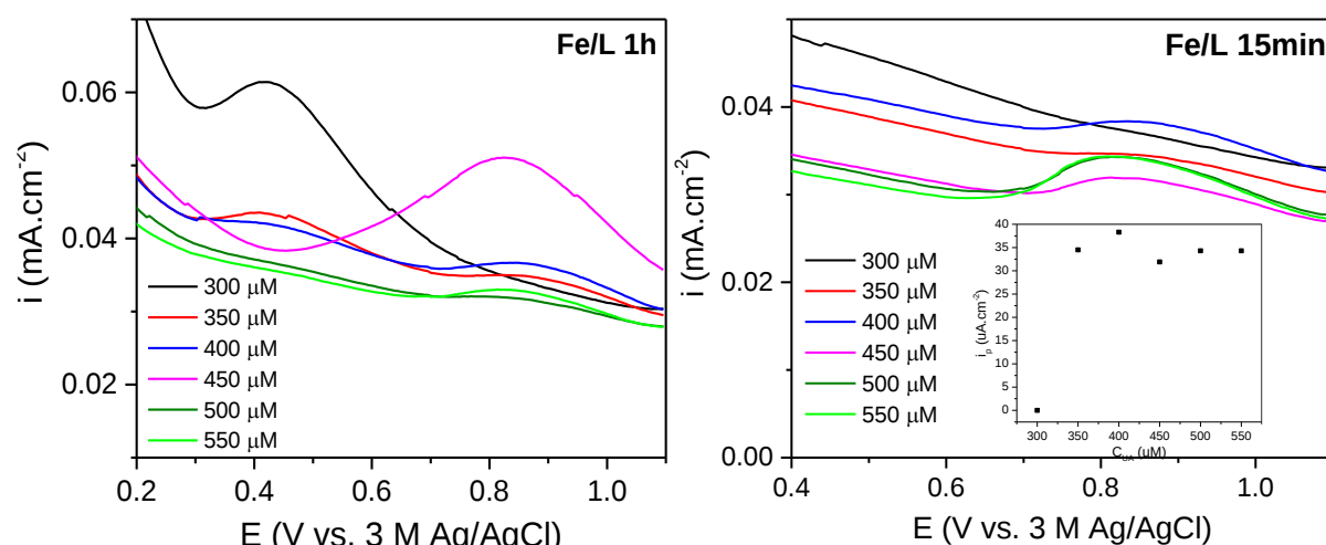
Figure 2.50 - DPV voltammograms of UA concentrations on a range of 300 to 550 \mu\text{M} on 1-hour and 15-minutes Fe/L films (2:1:1 ratio of M:H 4 L:PB , respectively) in PBS buffer.
