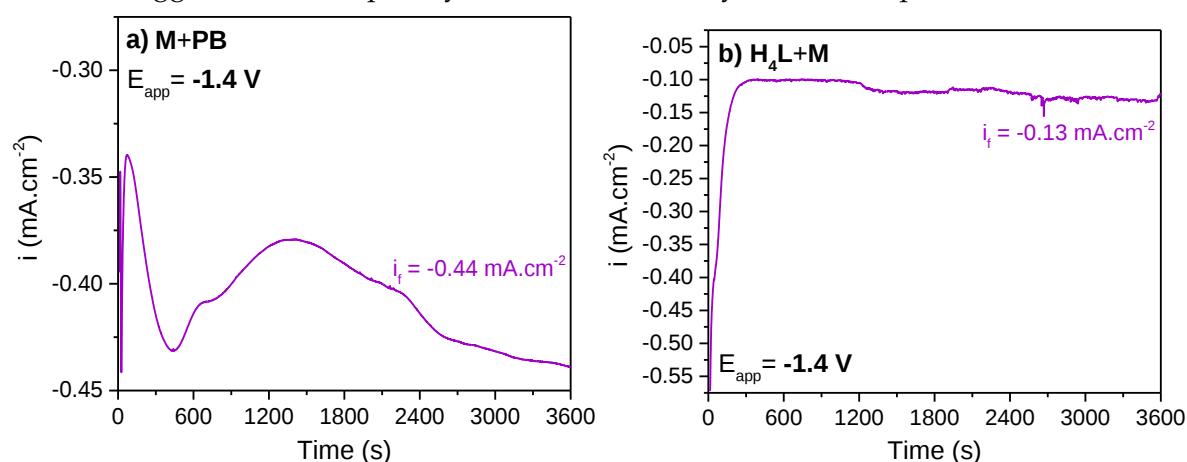
Figure 2.10 - Chronoamperograms following the deposition of a) the M+PB and b) M+H 4 L mixtures. Electrodepositions were performed in 10 mL of \text{N}_2 saturated DMF with \text{TBAPF}_6 as the supporting electrolyte and recorded at 100 \text{ mV.s}^{-1} . The one-compartment electrochemical cell was also constituted by FTO as working, platinum wire as counter and 3 M \text{Ag/AgCl} as reference electrodes. Precursors quantities: 7 mM of M , 2 mM of H 4 L and 2 mM of PB .
