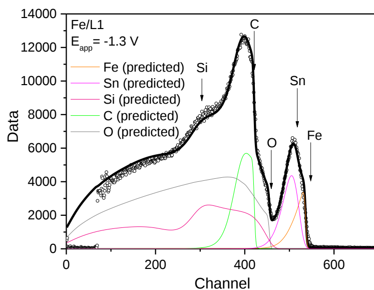
Figure A.94 - Adjusted RBS spectrum of the Fe/L1 film deposited at -1.3 V in the zone Identified as 007 (beam dimension: 3x4 \mu\text{m}^2 ).
