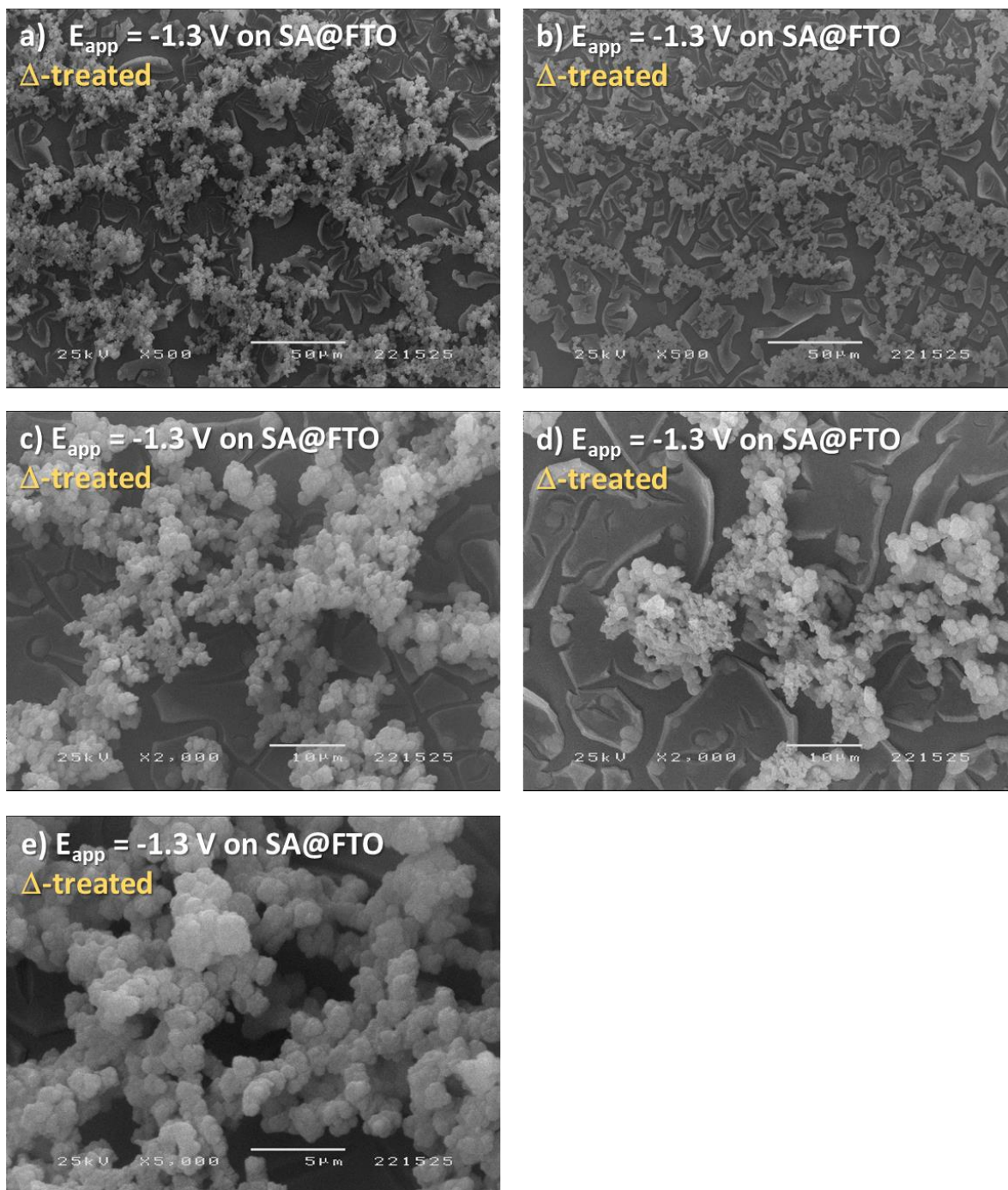
Figure A.59 - SEM images of the temperature-treated Fe/L film (2:1:1 ratio of M:H 4 L:PB , respectively) deposited at -1.3 V on SA@FTO after, magnified at a) x500, b) x500, c) x2000, d) x2000 and e) x5000.
