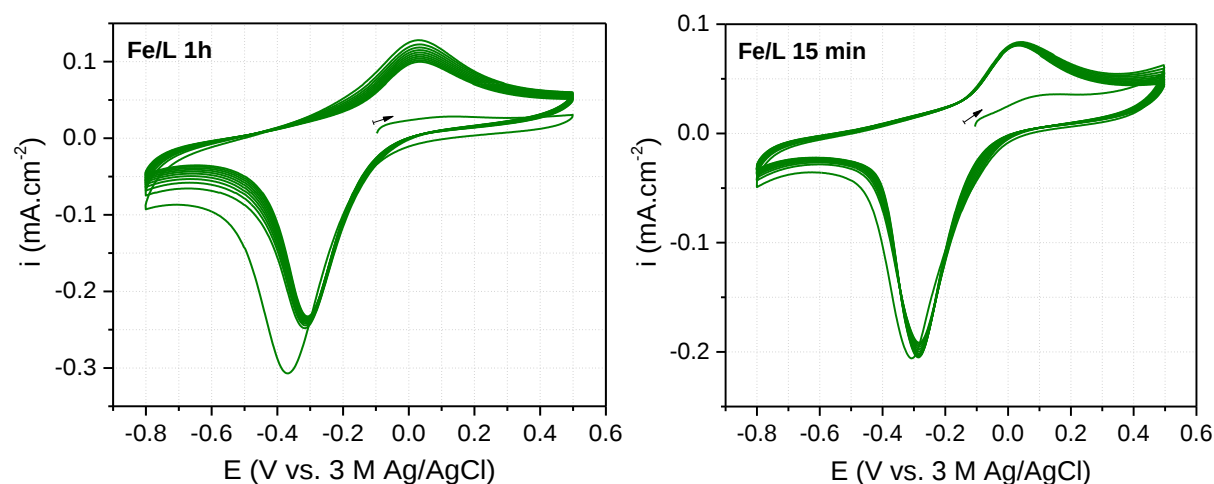
Figure 2.49 - Cyclic voltammograms of the 1-hour and 15-minute Fe/L films (2:1:1 ratio of M:H 4 L:PB , respectively) deposited on the FTO working electrode (0.7 cm 2 ). CVs were performed in 10 mL of N 2 saturated PBS buffer and recorded at 100 mV.s -1 . The one-compartment electrochemical cell was also constituted by platinum wire as counter and 3 M Ag/AgCl as reference electrodes.
