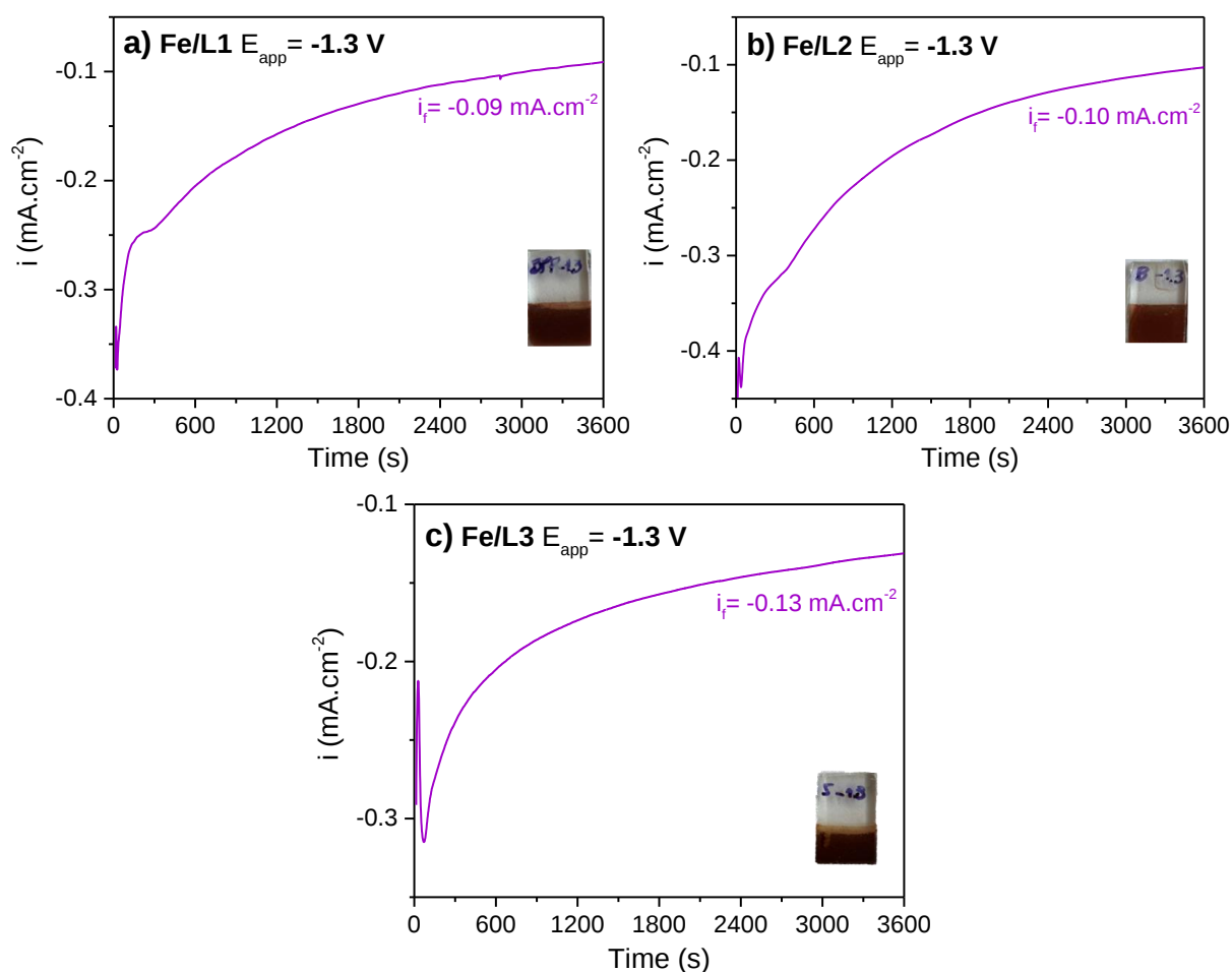
Figure 2.37 - Chronoamperograms following the deposition of a) Fe/L1 , b) Fe/L2 and c) Fe/L3 films at -1.3 V. Electrodepositions were performed in 10 mL of N 2 saturated DMF and TBAPF 6 as the supporting electrolyte. The one-compartment electrochemical cell was also constituted by FTO as working, platinum wire as counter and 3 M Ag/AgCl as reference electrodes. Precursor quantities: 4 mM of M , 2 mM of H 4 L1 , H 4 L2 or H 4 L3 and 2 mM of PB .
