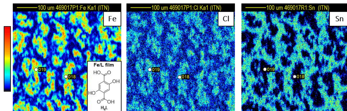
Figure 2.34 - Fe, Cl and Sn atom mapping of temperature-treated Fe/L film (2:1:1 ratio of M:H 4 L:PB , respectively) deposited at -1.3 V on SA@FTO, obtained by PIXE (beam size of 530×530 \mu\text{m}^2 ).
