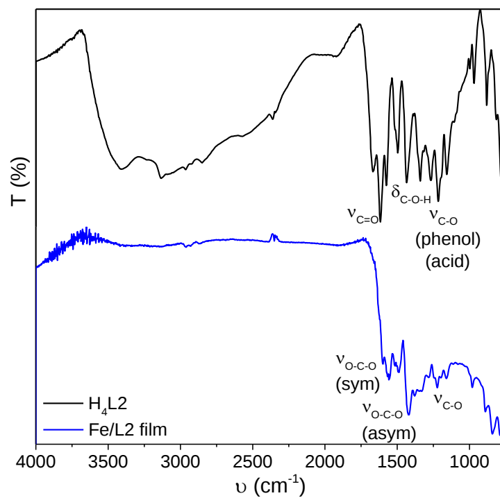
Figure A.89 - FTIR spectrum of H_4L2 (black) and DRIFT spectrum of the Fe/L2 film (blue) deposited at -1.3 V. Spectra were recorded in a range of 4000-500 cm^{-1} .
