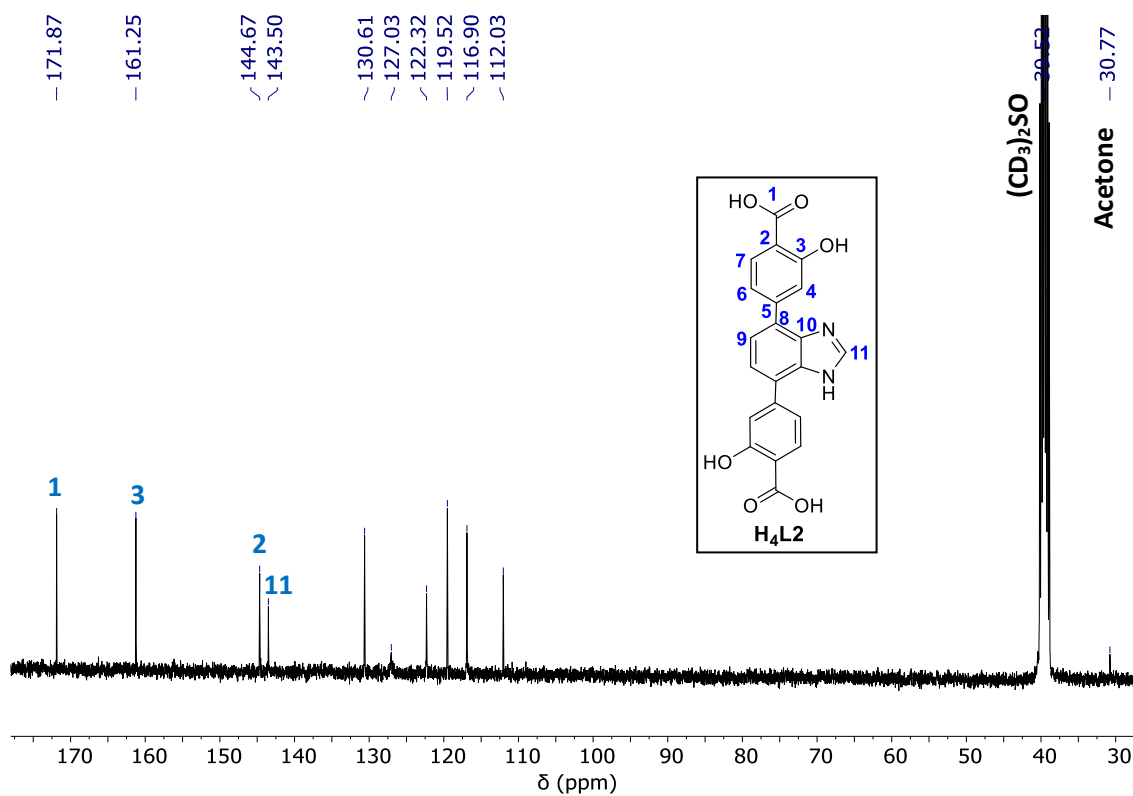
Figure 2.2 - ^{13}C NMR spectrum of H_4L2 in (CD_3)_2SO .
