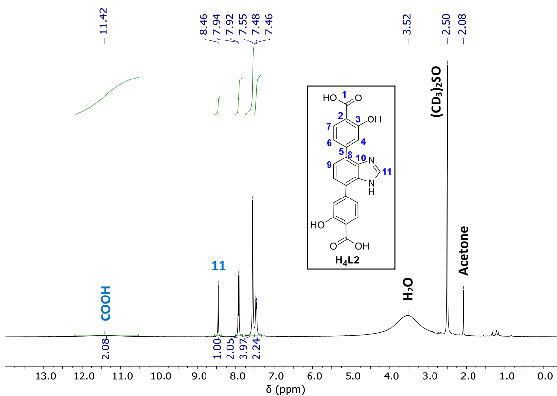
Figure 2.1 - ^1H NMR spectrum of H_4L2 in (CD_3)_2SO .
