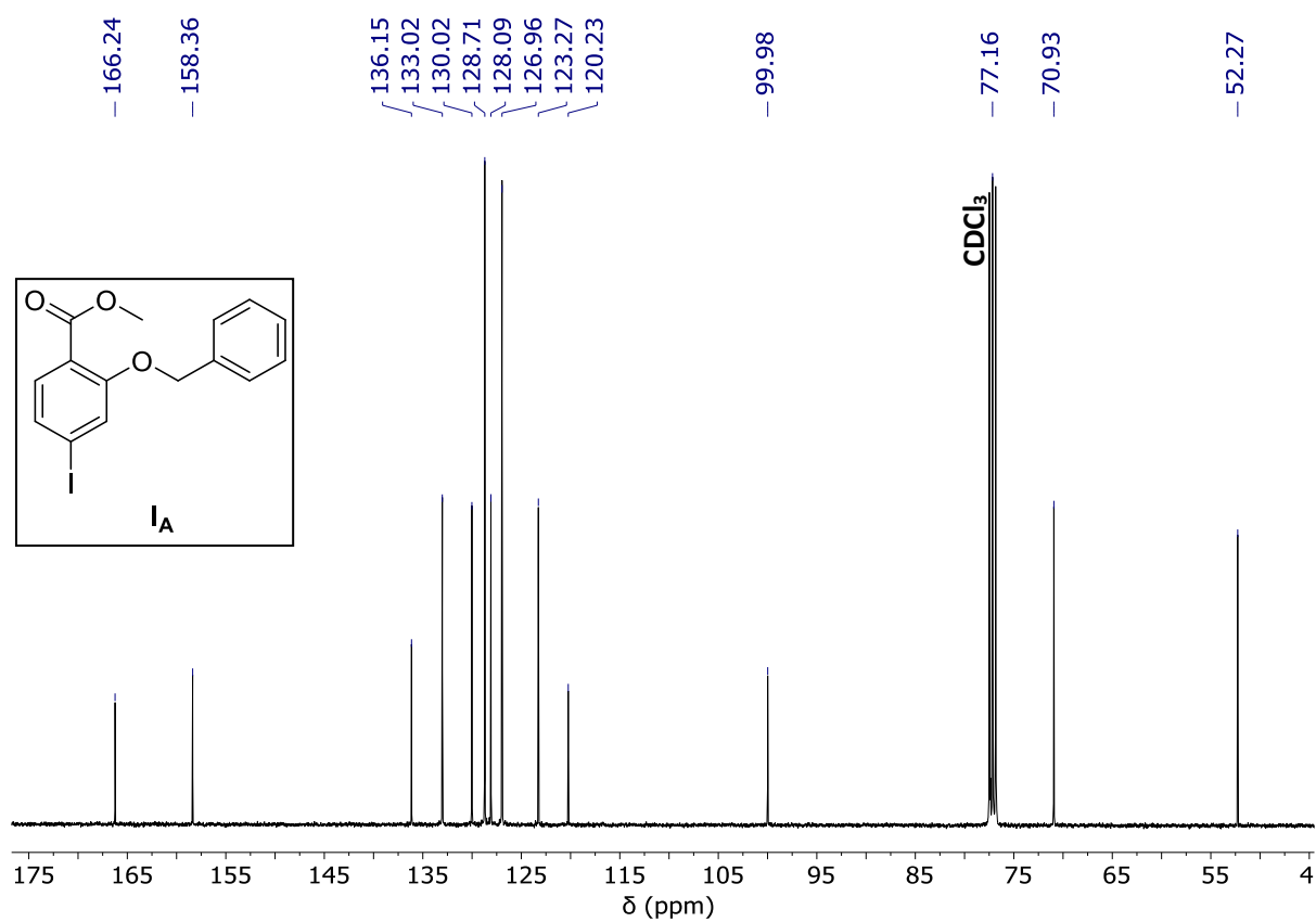
Figure A.3 - ^{13}\text{C} NMR spectrum of I_A intermediate in CDCl 3 .
