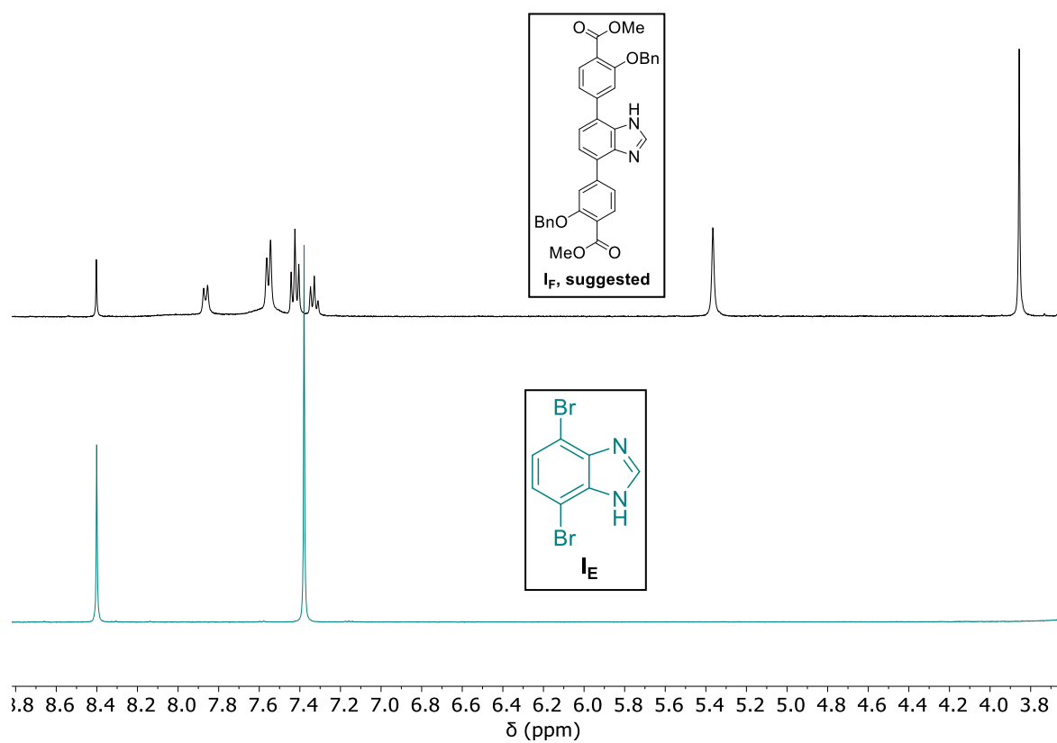
Figure A.15 - ^1\text{H} NMR superposed spectra of If (black) and IE (turquoise) intermediate in (\text{CD}_3)_2\text{SO} .
