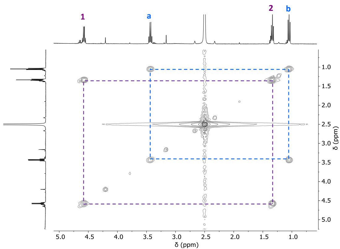
Figure A.24 - COSY spectrum of 1H in (\text{CD}_3)_2\text{SO} .
