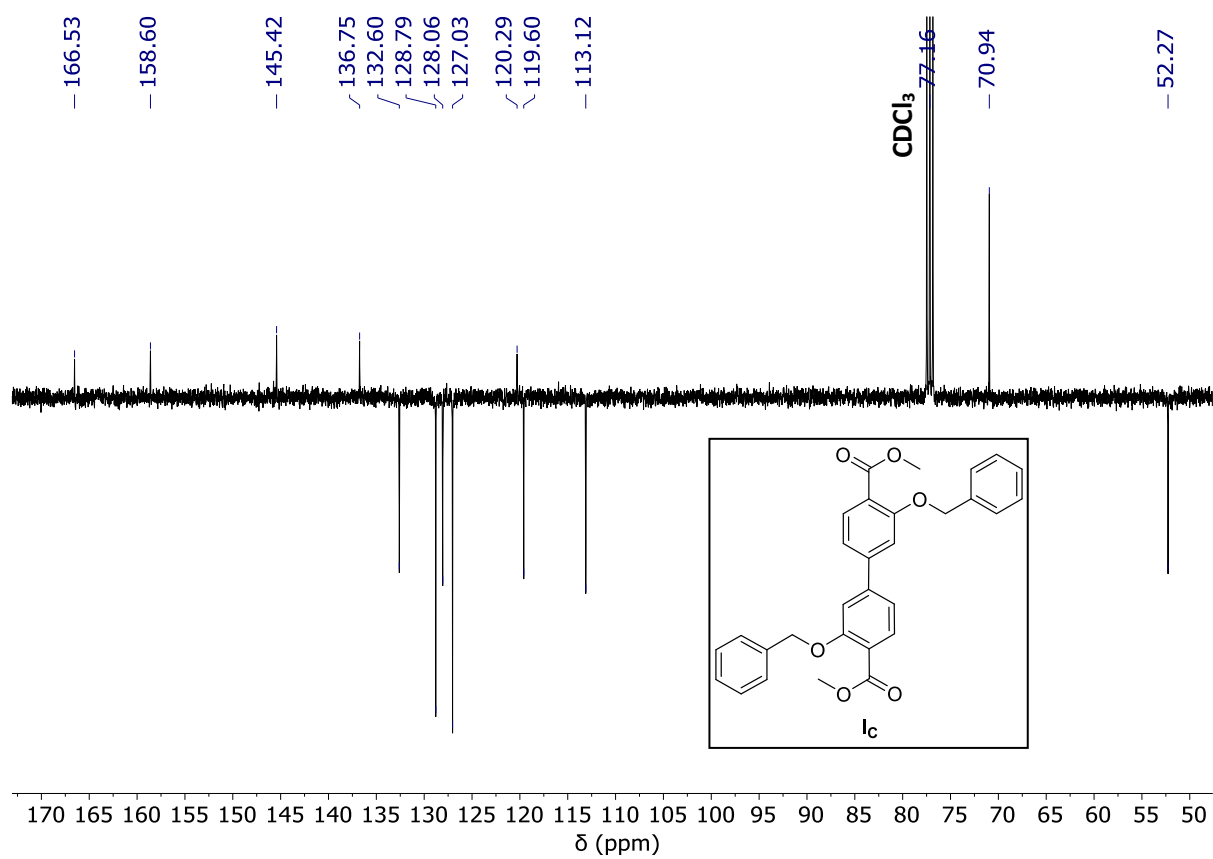
Figure A.7 - 13 C APT NMR spectrum of Ic intermediate in CDCl 3 .
