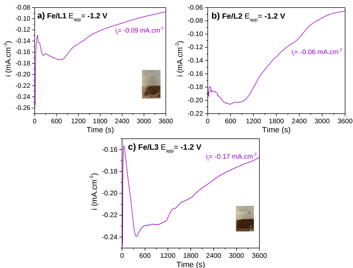
Figure 2.38 - Chronoamperograms following the deposition of a) Fe/L1 , b) Fe/L2 and c) Fe/L3 films at -1.2 V. Electrodepositions were performed in 10 mL of N 2 saturated DMF and TBAPF 6 as the supporting electrolyte. The one-compartment electrochemical cell was also constituted by FTO as working, platinum wire as counter and 3 M Ag/AgCl as reference electrodes. Precursor quantities: 4 mM of M , 2 mM of H 4 L1 , H 4 L2 or H 4 L3 and 2 mM of PB .
