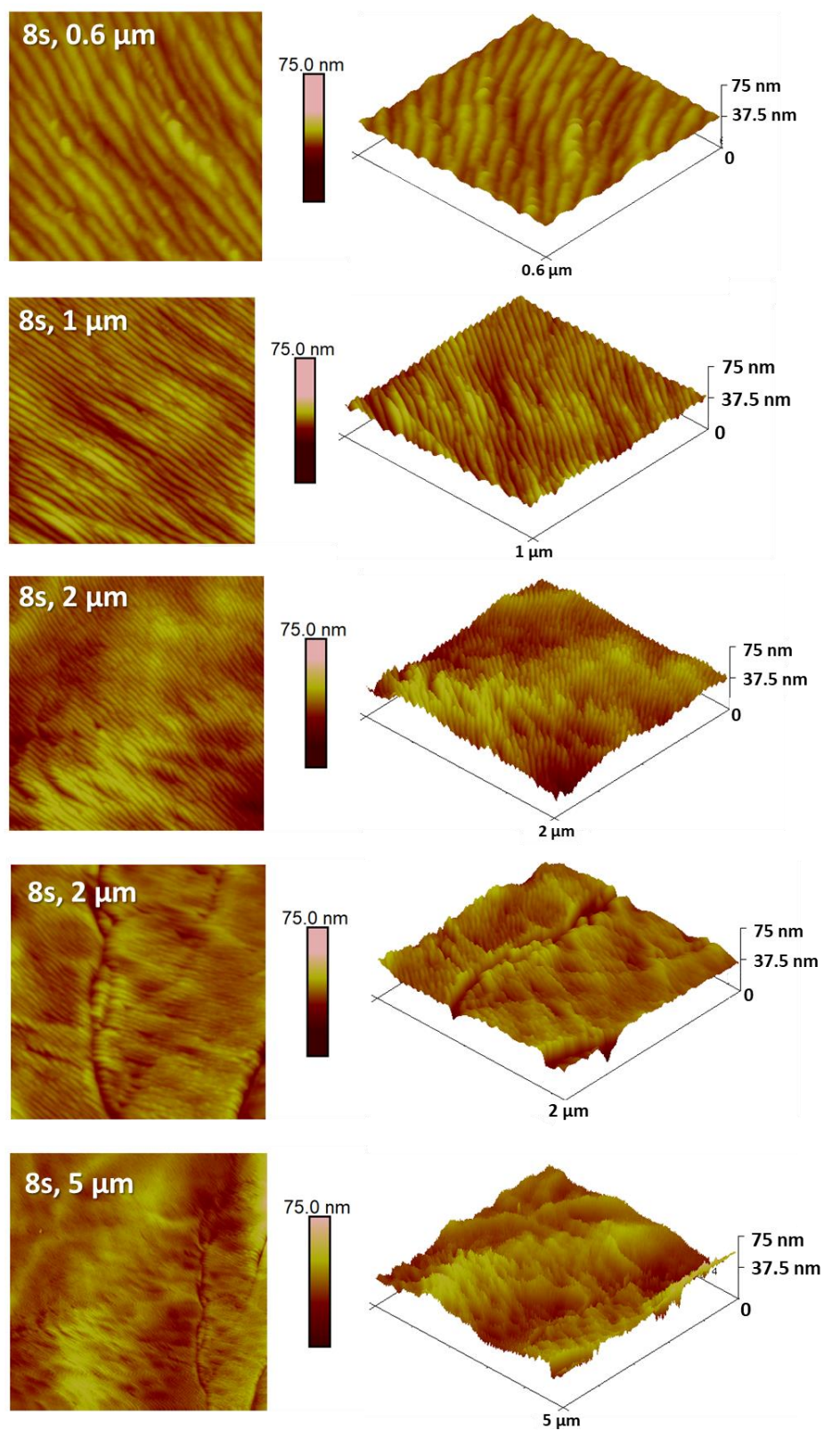
Figure A.67 - 2D and 3D AFM images of the Fe/L film (2:1:1 ratio of M:H 4 L:PB , respectively) deposited at -1.3 V for 8 seconds, with dimensions of 0.6x0.6 μm, 1x1 μm, 2x2 μm and 5x5 μm.
