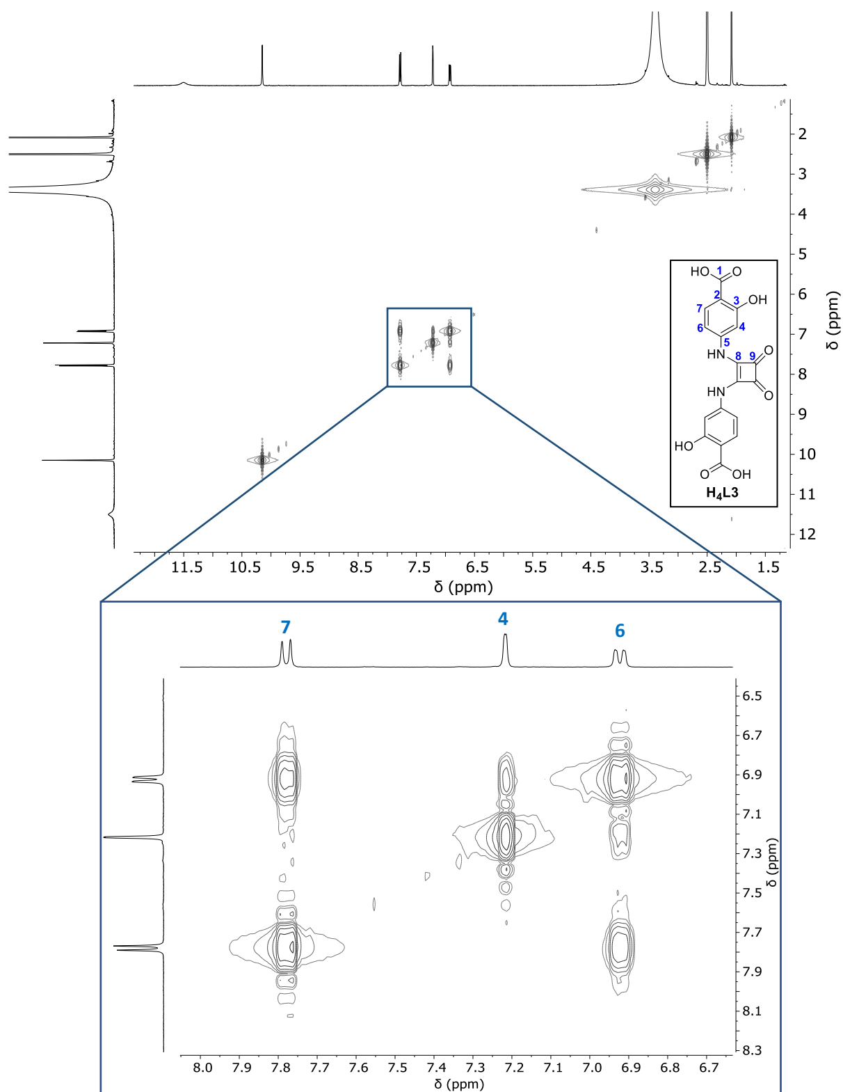
Figure A.25 - COSY spectrum of H 4 L3 in (\text{CD}_3)_2\text{SO} .
