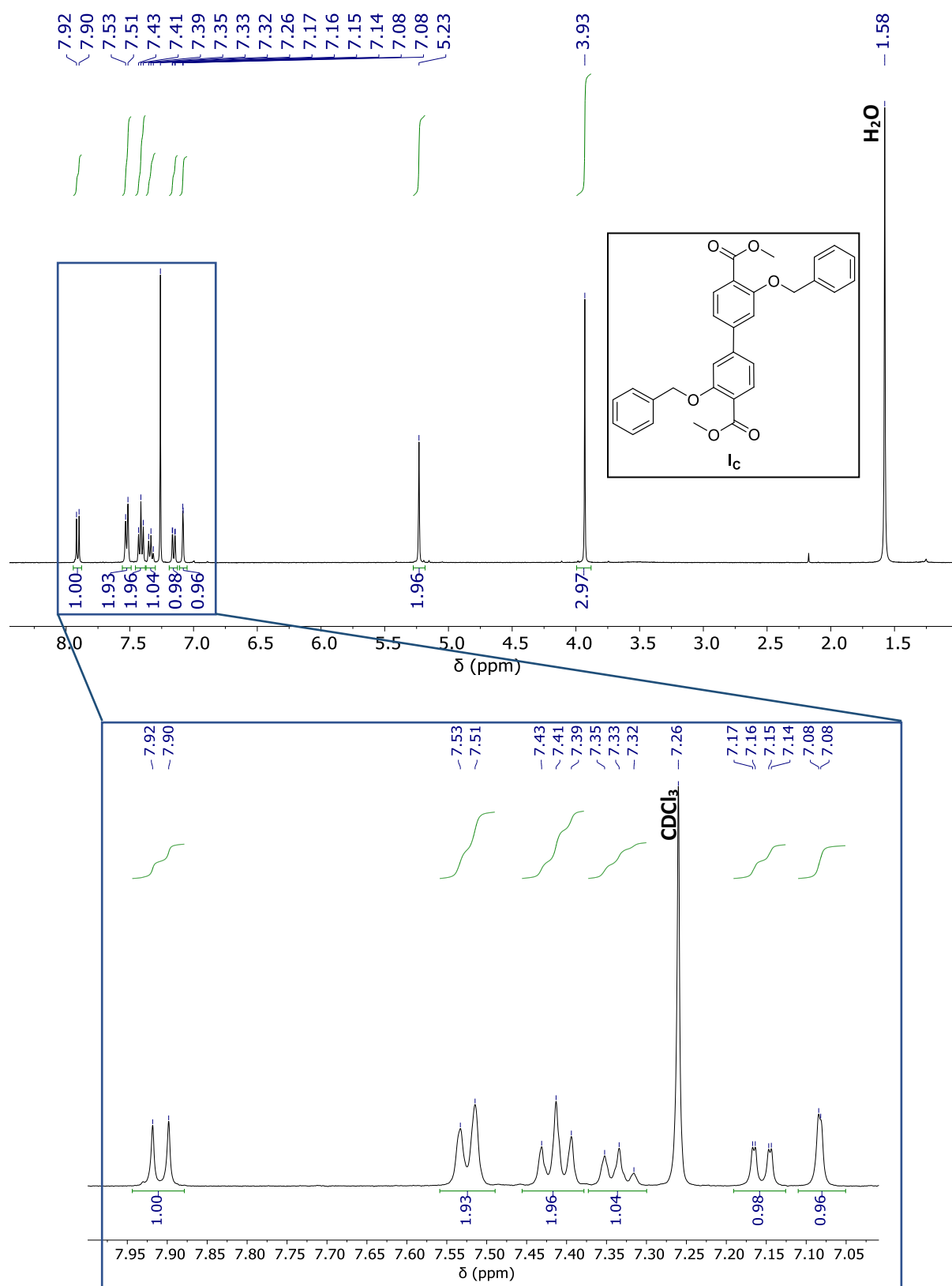
Figure A.6 - 1 H NMR spectrum of Ic intermediate in CDCl 3 .
