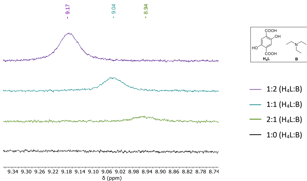
Figure A.46 - ^1\text{H} NMR spectra of \text{H}_4\text{L}:\text{B} mixtures in ratios of 1:2 (purple), 1:1 (turquoise), 2:1 (green) and 1:0 (black), respectively, in (\text{CD}_3)_2\text{SO} . Spectra were approximated in the range of 9.34-8.74 ppm.
