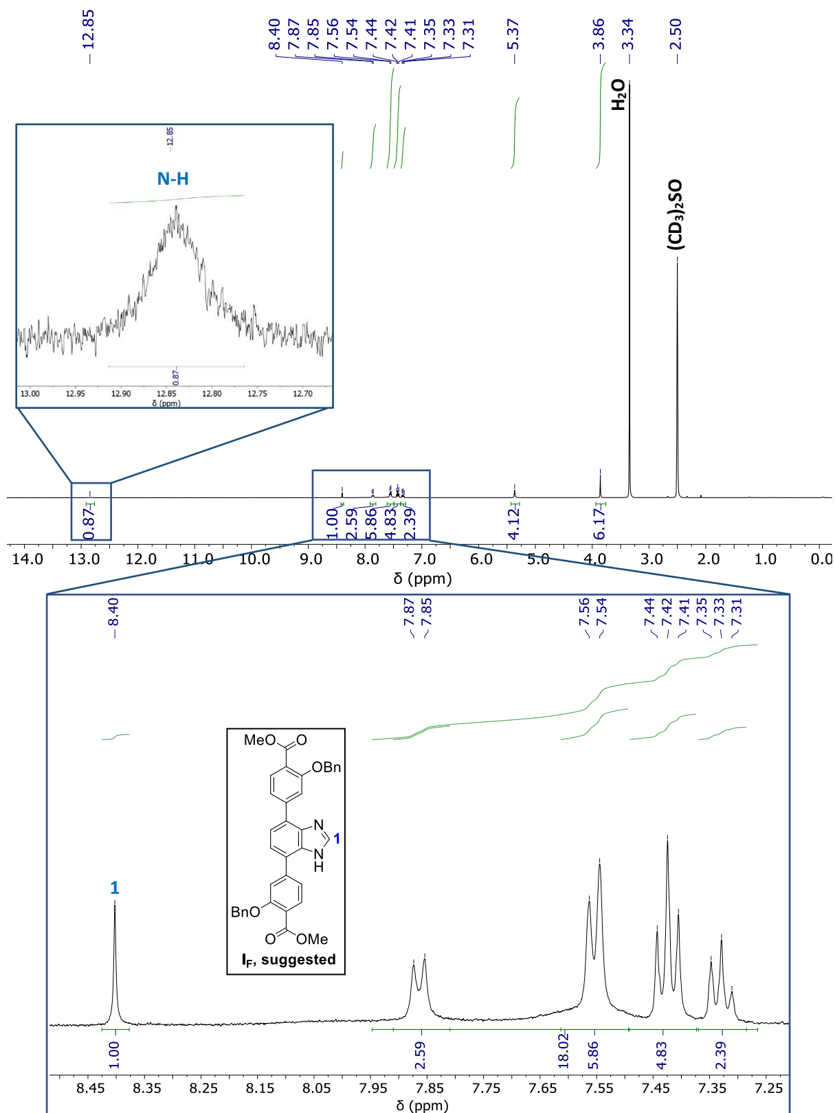
Figure A.14 - ^1\text{H} NMR spectrum of 1_E intermediate in (\text{CD}_3)_2\text{SO} .
