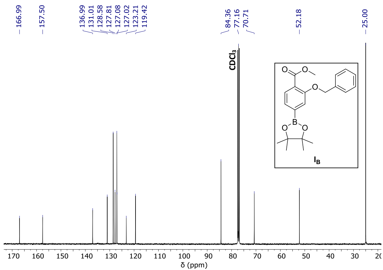
Figure A.5 - ^{13}\text{C} NMR spectrum of I_B intermediate in \text{CDCl}_3 .
