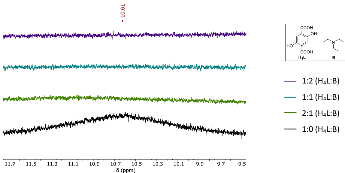
Figure A.45 - ^1\text{H} NMR spectra overlapping of \text{H}_4\text{L} and \text{B} mixtures in ratios of 1:2 (purple), 1:1 (turquoise), 2:1 (green) and 1:0 (black) of \text{H}_4\text{L}:\text{B} , respectively, in (\text{CD}_3)_2\text{SO} . Spectra were approximated in the range of 11.7-9.5 ppm.
