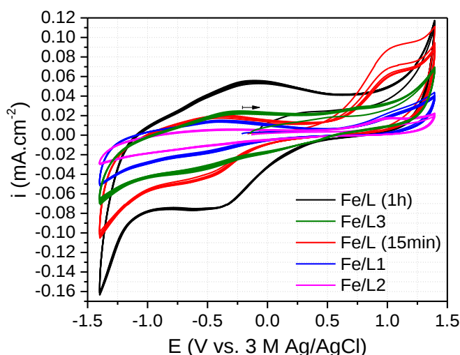
Figure 2.48 - Cyclic voltammograms of the Fe/L films deposited for 1 hour ( black ) and 15 minutes ( red ), as well as the Fe/L1 ( blue ), Fe/L2 ( pink ) and Fe/L3 ( green ) films, all deposited at -1.3 V. CVs were performed in 10 mL of N 2 saturated DMF and recorded at 100 mV.s -1 . The one-compartment electrochemical cell was also constituted by platinum wire as counter and 3 M Ag/AgCl as reference electrodes.
