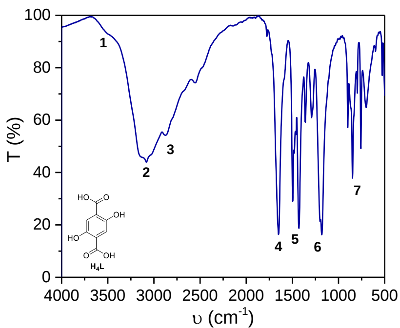
Figure A.29 - FTIR spectrum of H 4 L in KBr pellets. Spectrum was recorded in a range of 4000-500 cm -1 .
