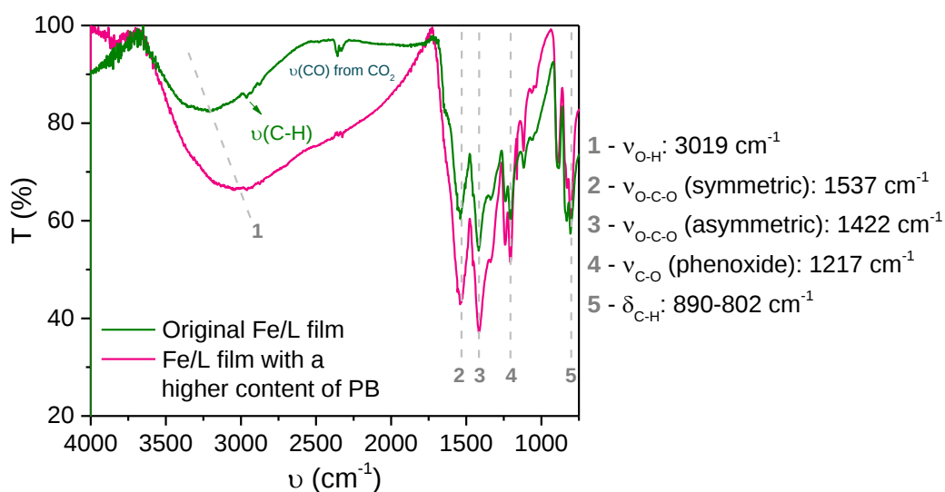
Figure A.80 - DRIFT spectra of the original (green) and with 4 mM of PB (pink) Fe/L films. Spectra were recorded in a range of 4000-750 cm -1 and the blank was measured with a gold coated plate.
