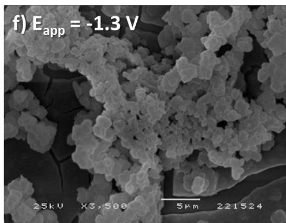
Figure A.56 - SEM images of the Fe/L film (2:1:1 ratio of M:H 4 L:PB , respectively) deposited at -1.3 V and magnified at a) x200, b) x500, c) x1500, d) x2000, e) x2000 and f) x3500.
