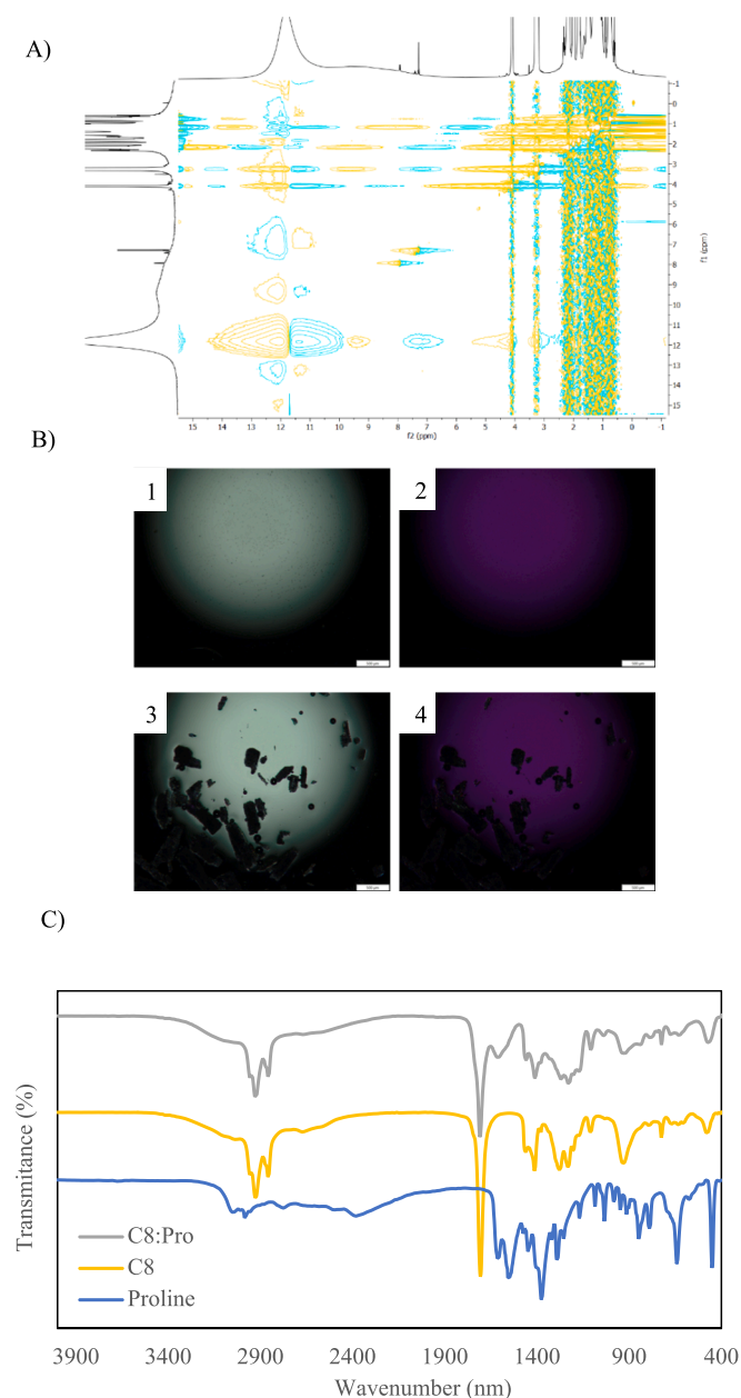
Fig. 4. ^1\text{H} - ^1\text{H} -NOESY spectra and signal assignment of C8:Pro (4:1) (A), Optical microscopy of 1) DES C8:Pro (4:1), and 3) physical mixture C8 + Pro; and POM images of 2) DES C8:Pro (4:1), and 4) physical mixture C8 + Pro (B), FTIR spectra of C8:Pro and individual components (C).
