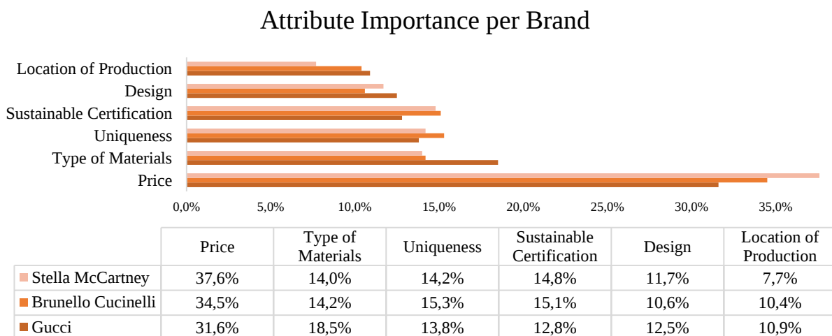
Figure 3.6 - Attribute importance
