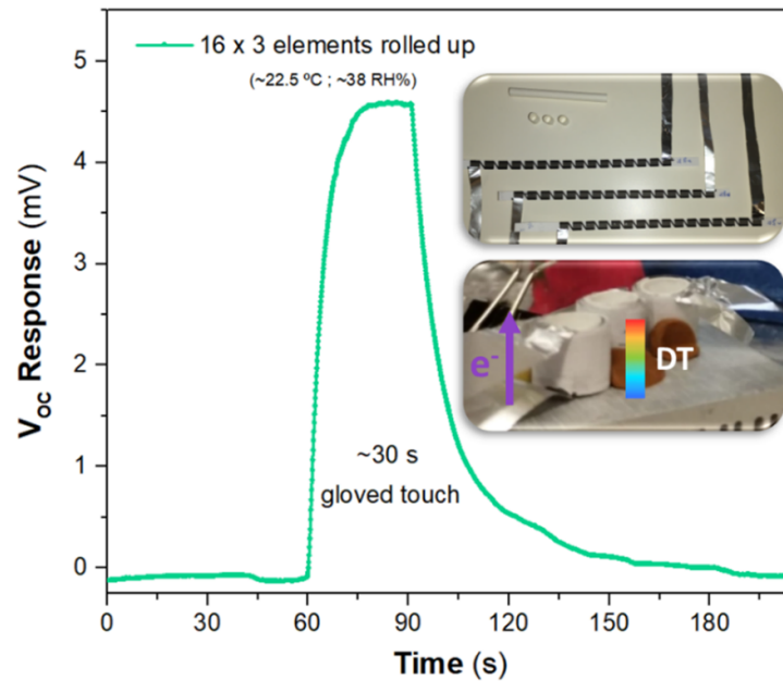
Figure 11. Voltage response ( V_{OC} ) of three rolled arrays of 16 TE elements, totaling 48 elements connected electrically in series, printed on office paper, with two layers and 20 wt% G_{Flakes} .
