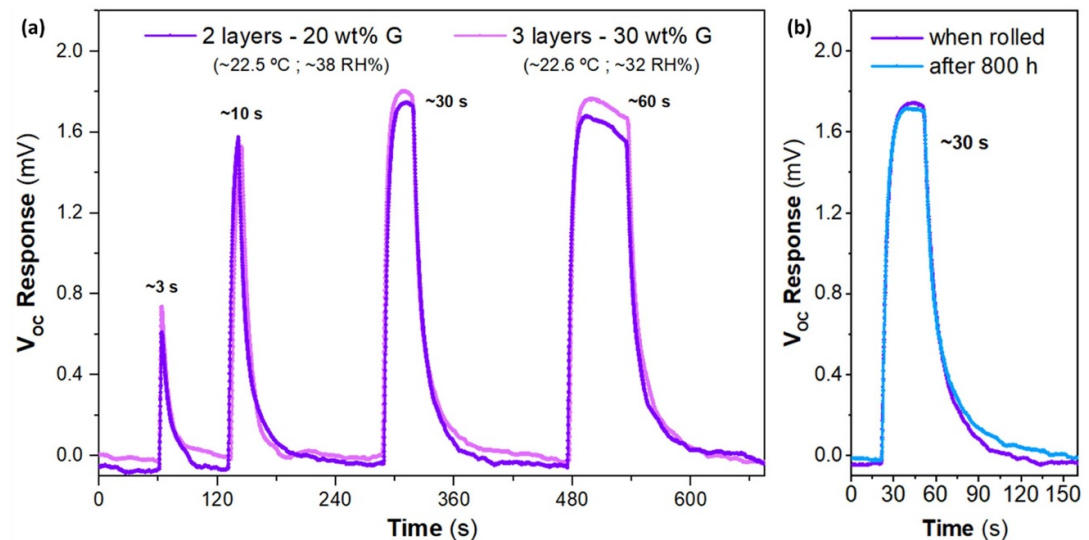
Figure 10. Comparison of 16-elements connected electrically in series, printed on paper with different conditions, (a) the dark purple curve is of a sample with two printed layers of 20 wt% G_{\text{Flakes}} , and the light purple is of a sample with three layers of 30 wt% G_{\text{Flakes}} , and (b) the sample in dark purple being remeasured after 800 h rolled up.
