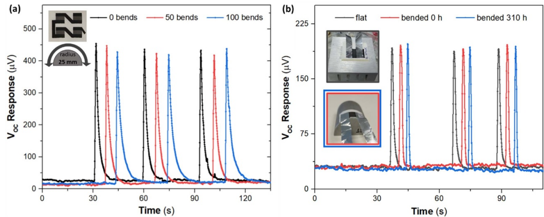
Figure 9. (a) Results for a dynamic bending test using a cylinder with 25 mm of curvature radius, with a four-element sample printed on cotton (three layers, 30 wt% G_{\text{Flakes}} ), and (b) Static bending test for a single element touch sensor using a sticker label substrate—three layers of 30 wt% G_{\text{Flakes}} .
