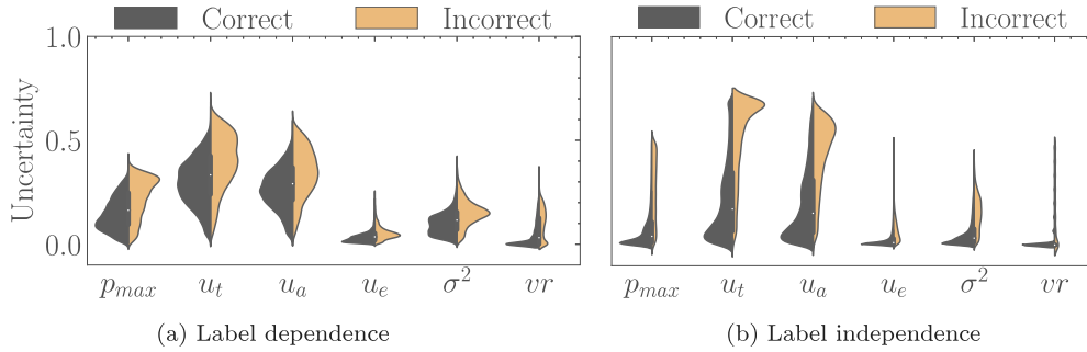
Fig. 9. Comparison of uncertainty value distributions for correctly and incorrectly classified samples using DeepEnsemble model. (a) label dependence approach, where the entire label combination is considered as either correct or incorrect, and (b) label independence approach, where each class is treated as a separate binary classification problem.
