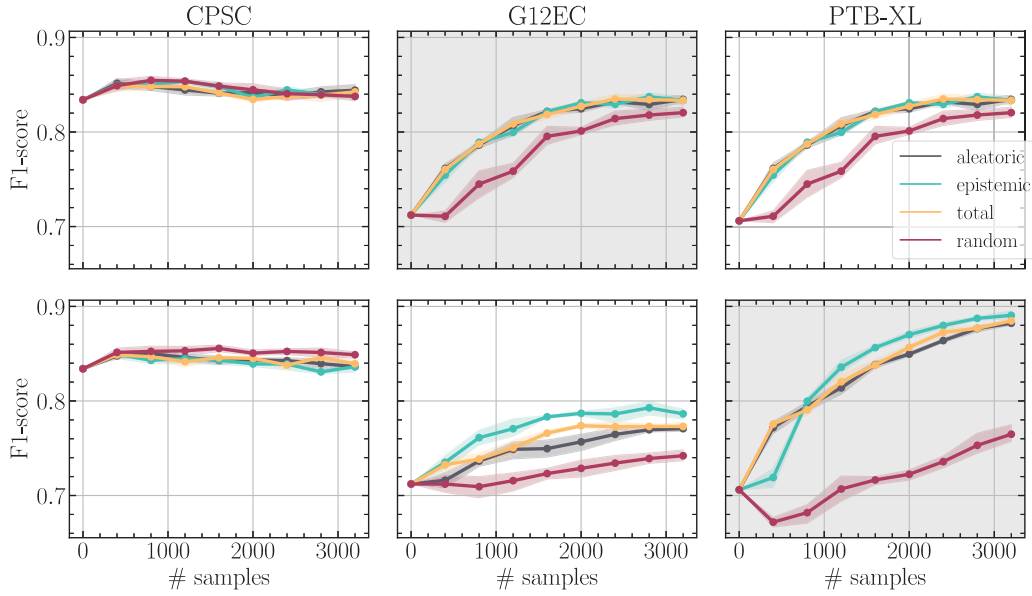
Fig. 13. Classification performance as a function of the number of samples used to retrain the DeepEnsemble. In the upper plots data from the G12EC dataset was used to retrain the model, and in the lower plots, PTB-XL data was used. The gray background represents the dataset used to retrain the models.
