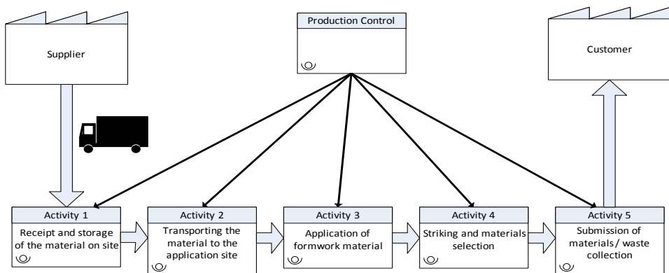
Figure 1: Formwork - Current Value Stream Mapping
