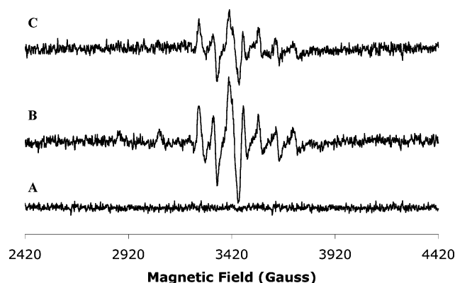
Fig. 7 Frozen aqueous solution X-band EPR spectra of 25 mM decavanadate (vanadate total) in (A) 2 mM Tris (pH 7.5), 0.2 mM \text{CaCl}_2 , 0.2 mM ATP with (B) 100 \mu M G-actin or (C) 100 \mu M F-actin. Upon protein addition the oxidovanadium(IV) typical signals are elicited.
