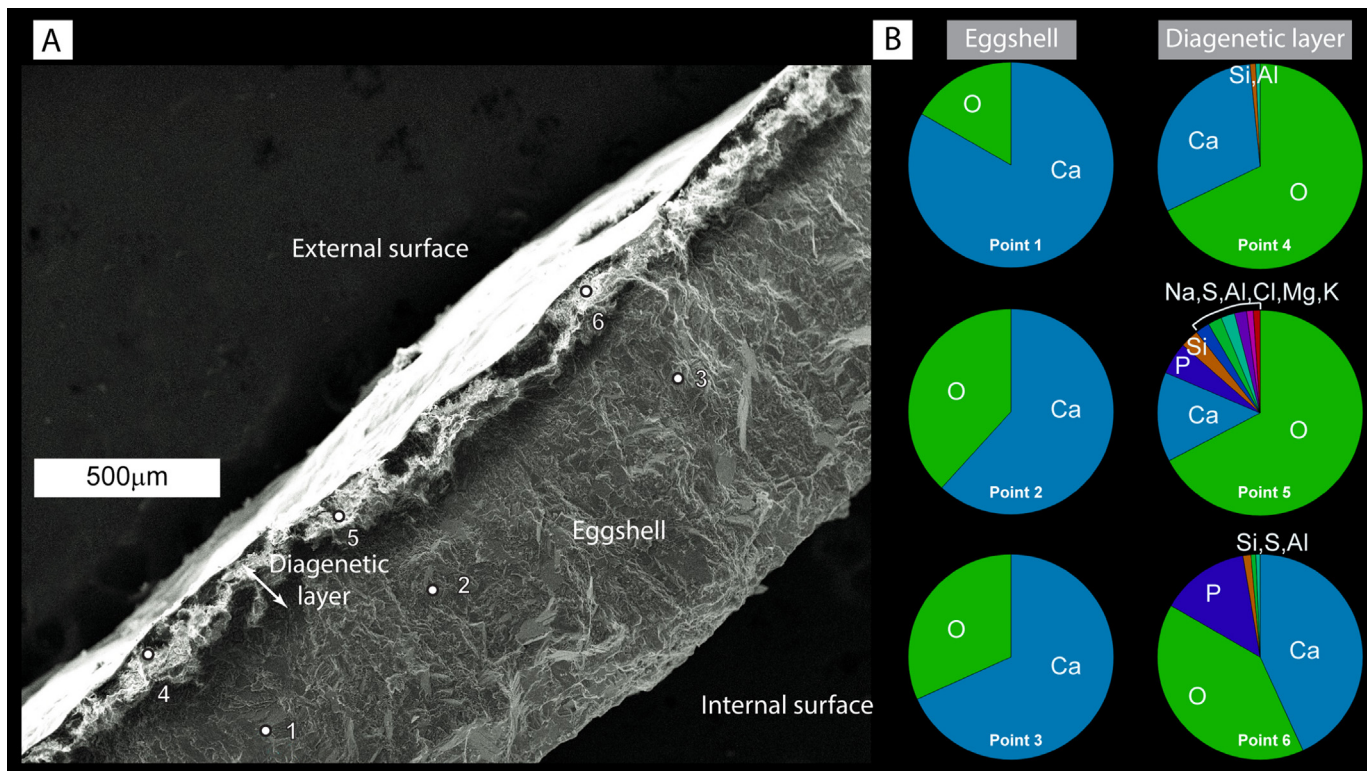
Fig. 5. Representative example of ultrastructure inspection and elemental point analysis of Jurassic eggshells. A) Detail of eggshell structure with clear identification of the limits of the diagenetic layer. Numerals indicate the exact points chosen to perform elemental analysis. B) Point analysis results for eggshell (points 1 to 3) and adjacent diagenetic layer (points 4 to 6). Note a minor contribution of non-carbonate components (Si, Al, P, and others) throughout the diagenetic layer (see text for details).
