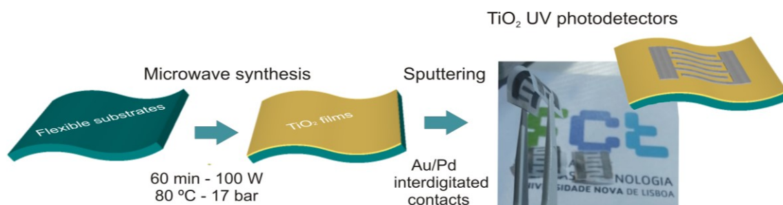
Figure 1 – Scheme of the TiO 2 UV photodetector production stages and photograph of the final device showing high flexibility.
