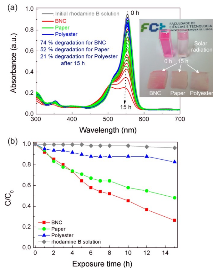
Figure 8. (a) Rhodamine B absorbance spectra at different solar light exposure times up to 15 h. The images of Rhodamine B solutions at 0 h and after 15 h are presented together with the materials after the photocatalytic experiments. (b) Rhodamine B degradation ratio ( C/C_0 ) vs. solar simulating light exposure time.
