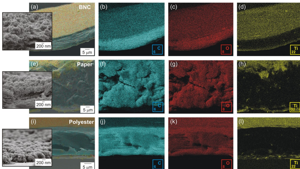
Figure 3. SEM images of the TiO 2 films grown on BNC (a), tracing paper (e) and polyester (i) substrates together with their corresponding EDS maps of C (b, f and j), O (c, g and k) and Ti (d, h and l). The insets show the cross-section SEM images of all materials.
