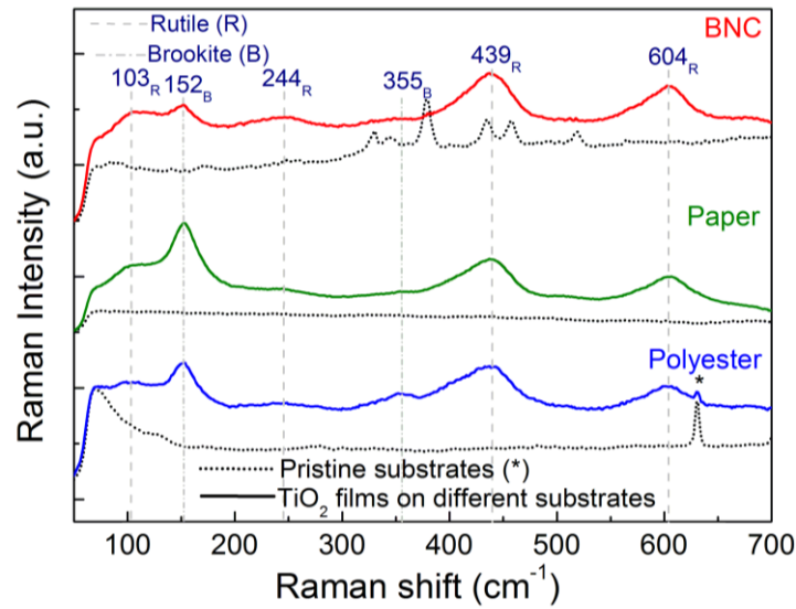
Figure 4. Raman spectra of the TiO 2 films together with their pristine substrates (dot lines). Dashed lines indicate the rutile bands and dot/dashed ones point out to the brookite ones.
