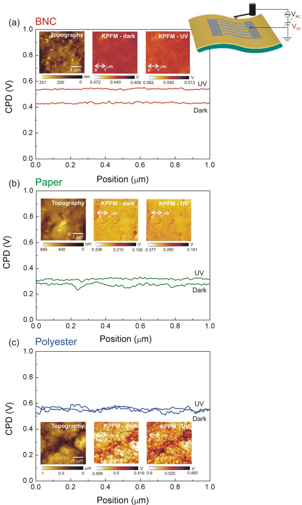
Figure 7. CPD averaged profiles together with the corresponding topography and surface potential images with and without UV irradiation at room temperature for the \text{TiO}_2 films grown on (a) BNC, (b) tracing paper and (c) polyester substrates. The profiles were carried out in regions that represented the average surface potential of the image. The scheme of the KPFM measurement is presented.
