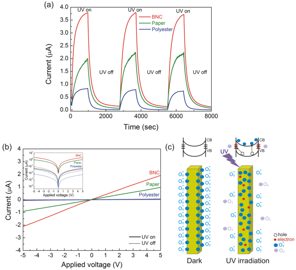
Figure 6. (a) Cycling behaviour of TiO 2 film photodetectors at 10 V and under a 360 nm UV source. (b) I – V curves showing the dark current and photocurrent of the produced devices. (c) Schematic diagrams of dark and UV irradiation processes. The top drawing shows the schematic of the energy band diagrams, where VB and CB are the valence and conduction band, respectively. The bottom drawing shows the dark and UV irradiation mechanisms, where in dark, the oxygen molecules adsorbed at the surface capture the free electron present in the n -type semiconductor forming a low-conductivity depletion layer near the surface. Under UV irradiation, photogenerated holes migrate to the surface and are trapped, leaving behind unpaired electrons that contribute to the photocurrent [60,61].
