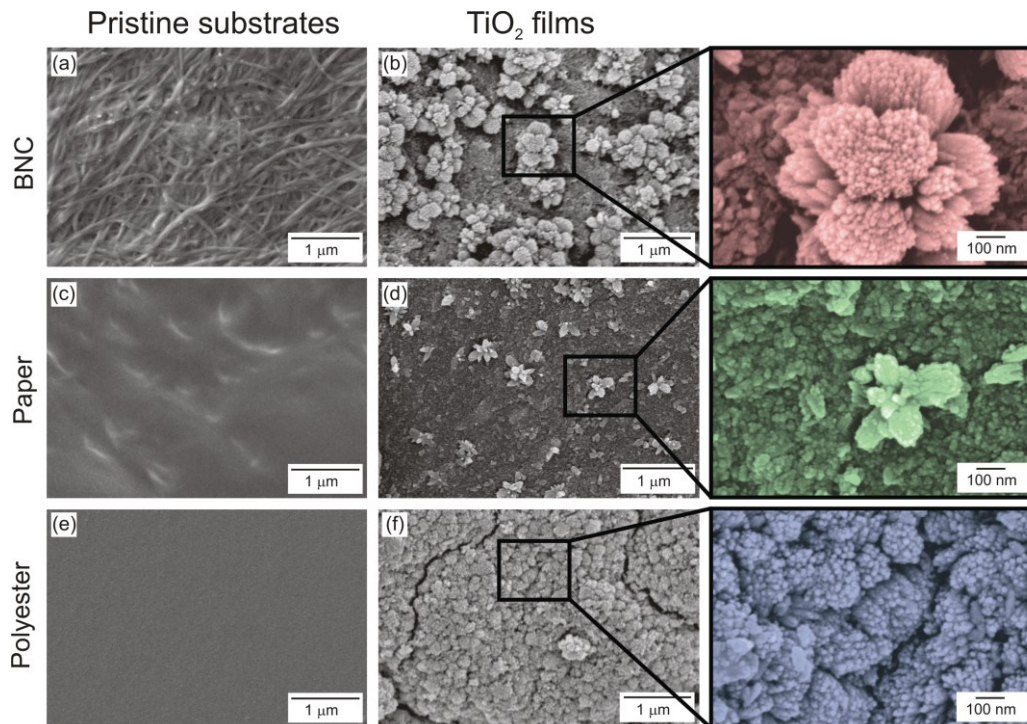
Figure 2. SEM images showing the BNC (a), paper (c) and polyester (e) pristine substrates together with the TiO 2 films grown on BNC (b), tracing paper (d) and polyester (f) substrates. The false colored insets show the TiO 2 films and the nanorod flower-like structures with a higher magnification.
