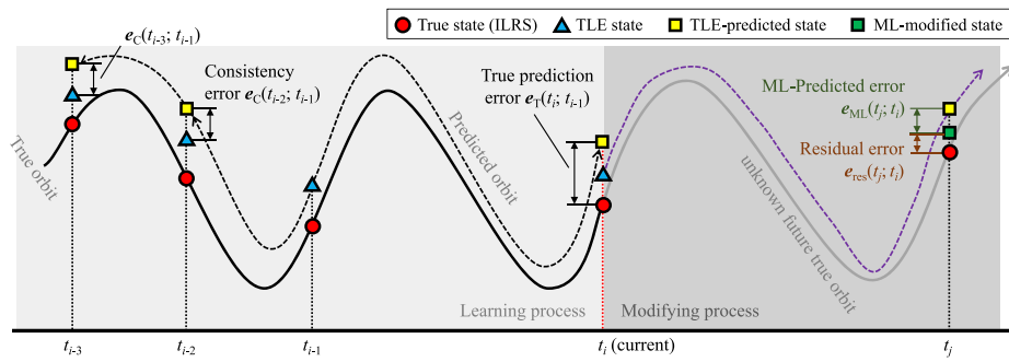
Fig. 5. Illustration of the dataset structure for the ML approach to SGP4 error correction, as presented by Peng and Bai [71].
